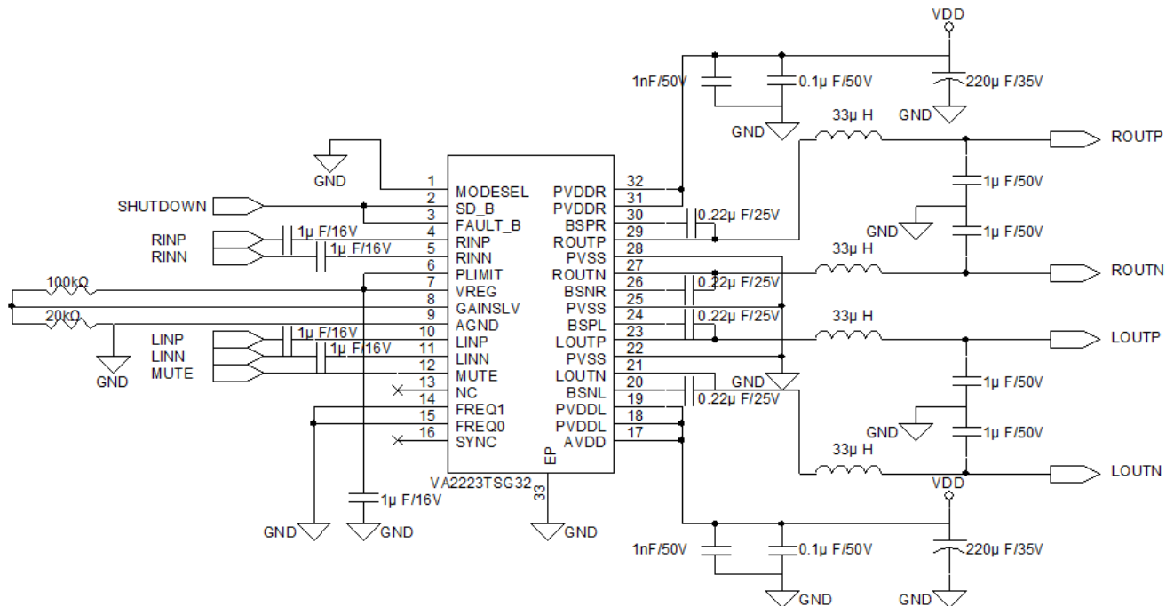
Figure 6. VA2223 TSSOP32 Stereo Reference Application
