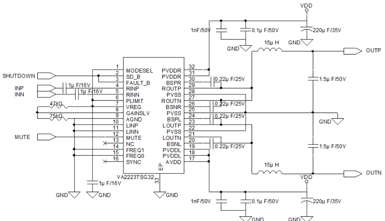
Figure 7. VA2223 TSSOP32 Mono Reference Application
