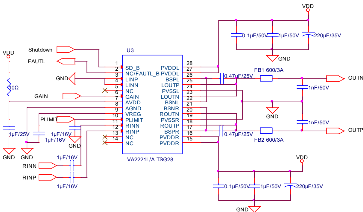
Figure 8. VA2221L/A Mono Reference Application with Ferrite Bead
