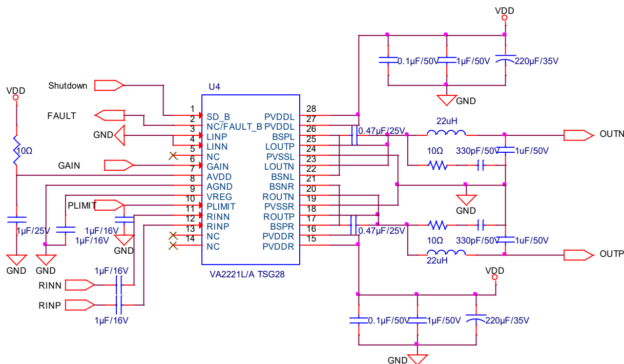
Figure 7. VA2221L/A Mono Reference Application with LC Filter
