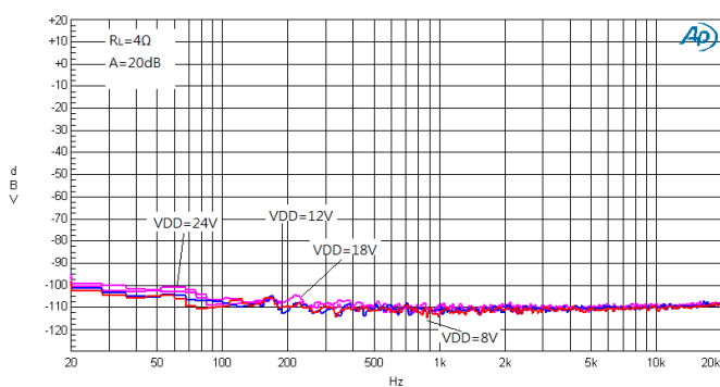
Figure 21. Noise FFT
