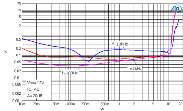
Figure 20. THD+N vs. Output Power
