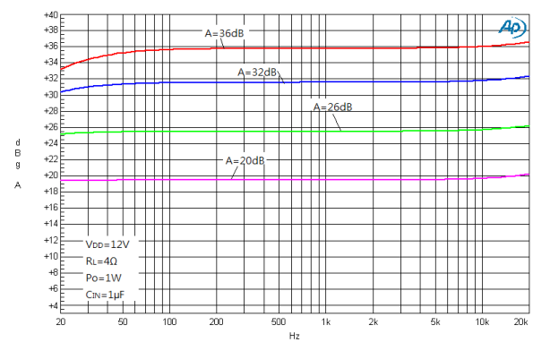
Figure 18. Frequency Response
