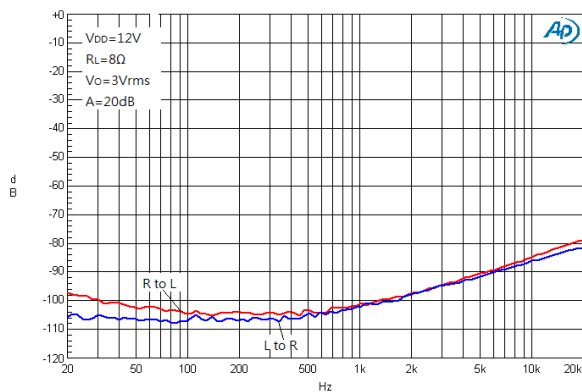
Figure 11. Crosstalk
