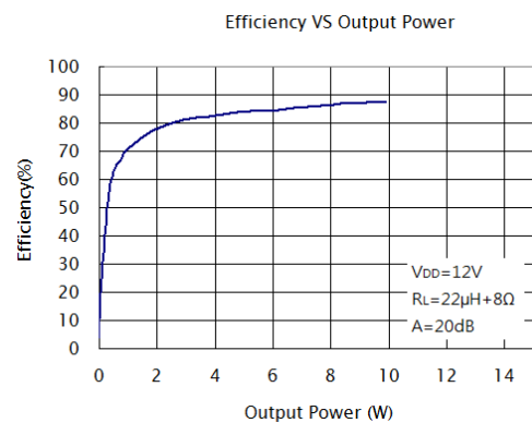
Figure 14. Efficiency
