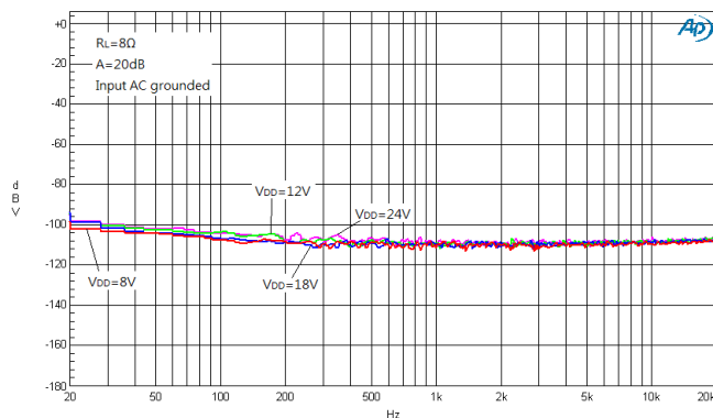
Figure 13. Noise FFT
