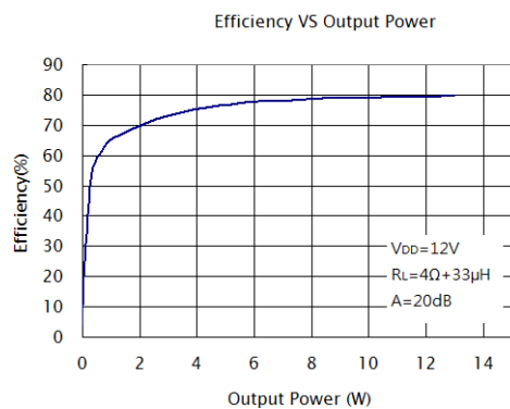
Figure 23. Efficiency
