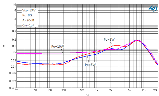
Figure 10. THD+N vs. Frequency
