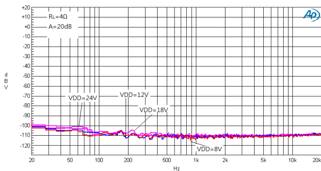
Figure 21. Noise FFT
