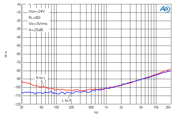
Figure 12. Crosstalk
