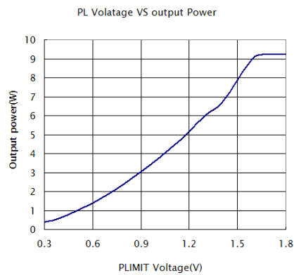
Figure 17. PLIMIT voltage vs. Output Power
