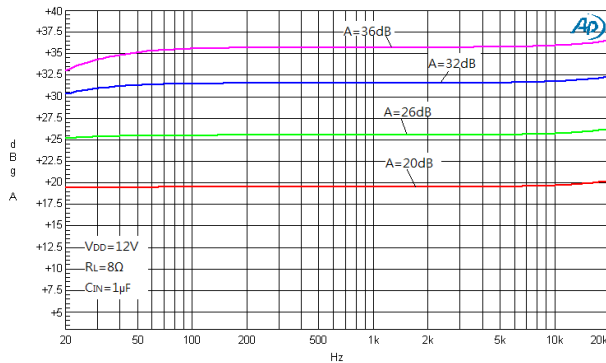
Figure 7. Frequency Response
