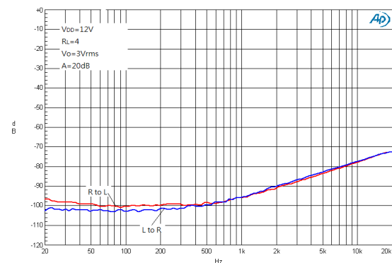
Figure 22. Crosstalk
