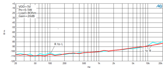
Figure 25. Crosstalk
