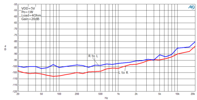
Figure 24. Crosstalk
