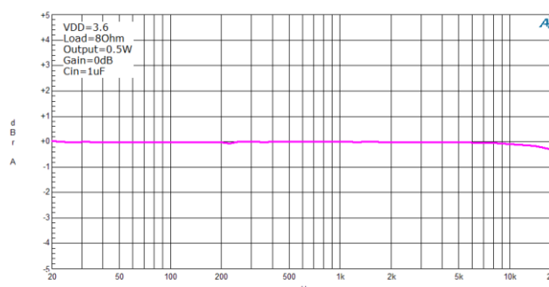
Figure 10. Frequency Response
