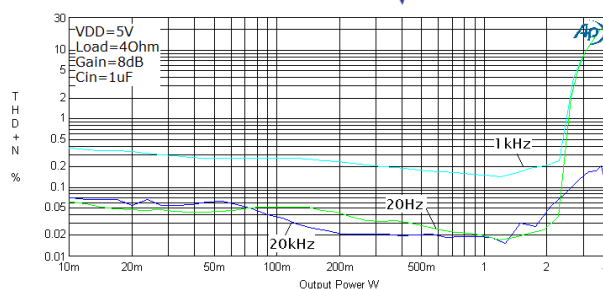
Figure 15. THD+N vs. Output Power
