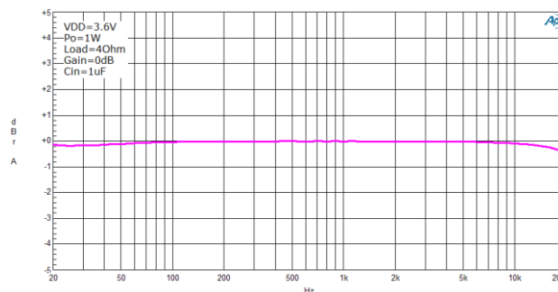
Figure 9. Frequency Response
