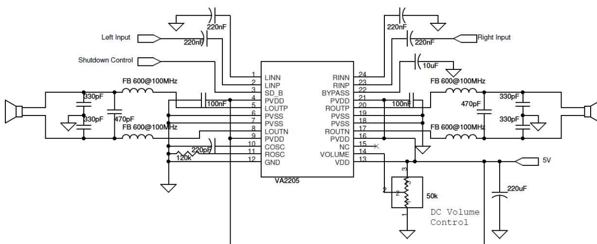
Figure 31. VA2205 with single-ended input configuration
