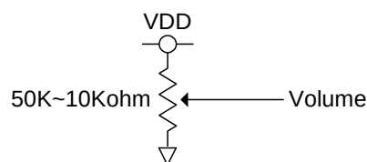
Figure 3. DC volume application circuit
