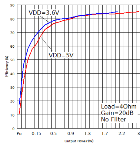
Figure 26. Efficiency
