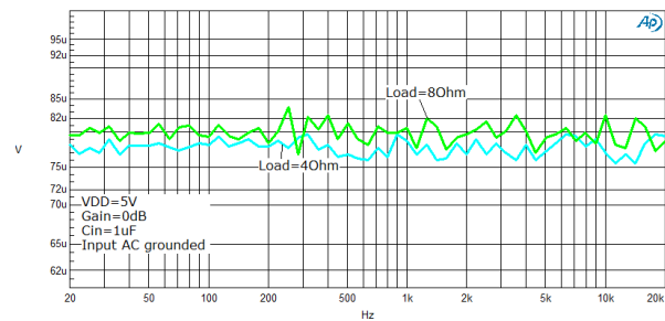
Figure 21. Integrated Noise
