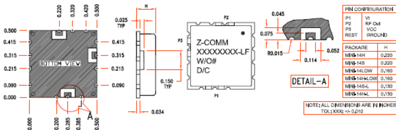
PHYSICAL DIMENSIONS
