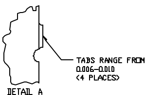
PHYSICAL DIMENSIONS
