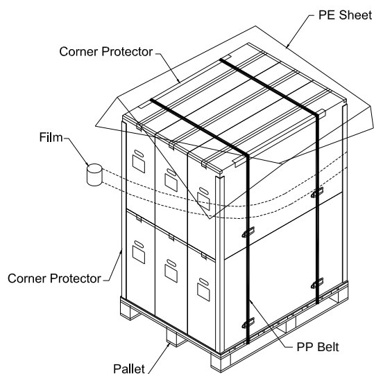
Figure.11-2 Packing method
