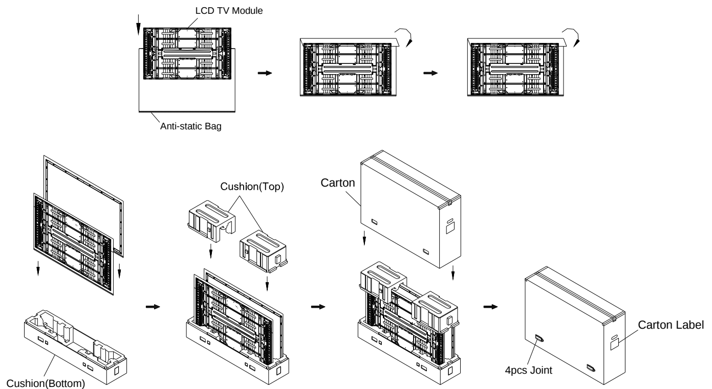
Figure.11-1 packing method
