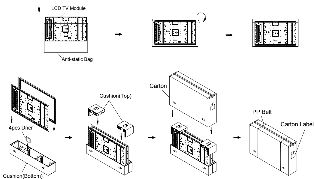
Figure.9-1 packing method
