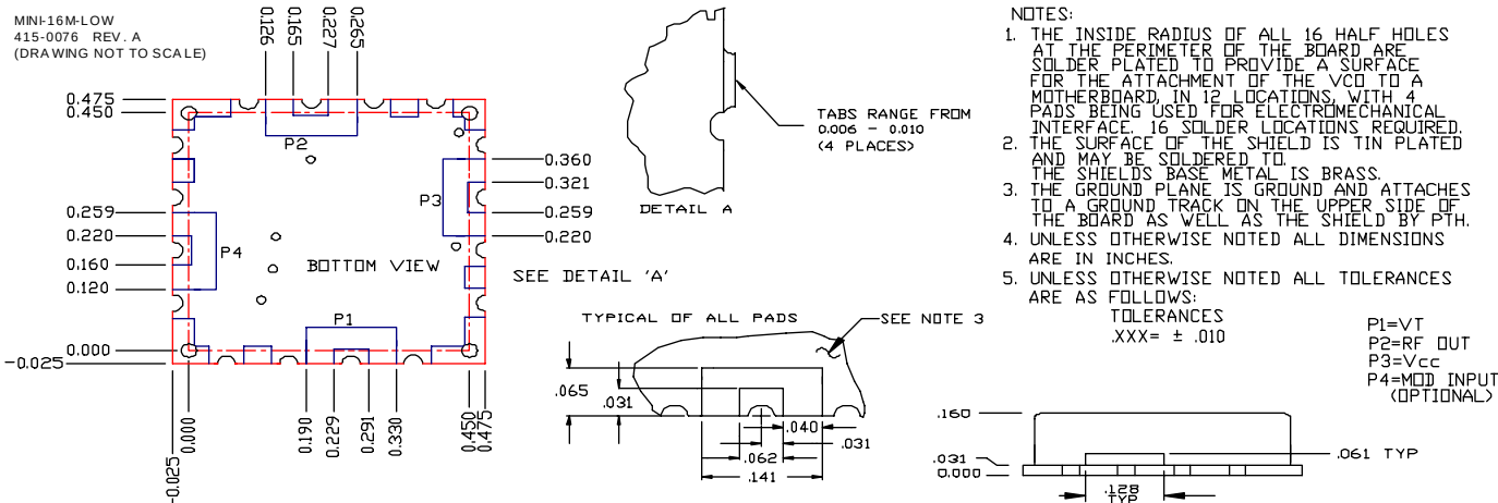
PHYSICAL DIMENSIONS
