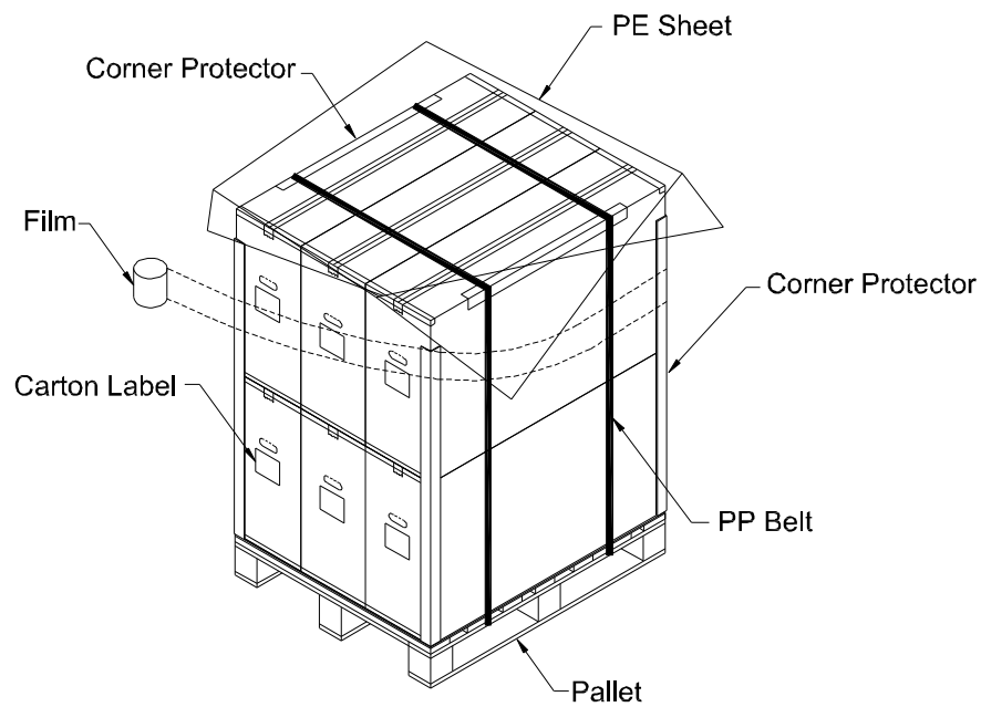
Figure.10-2 packing
