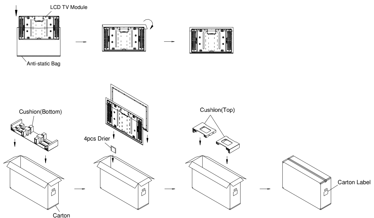
Figure.9-1 packing method
