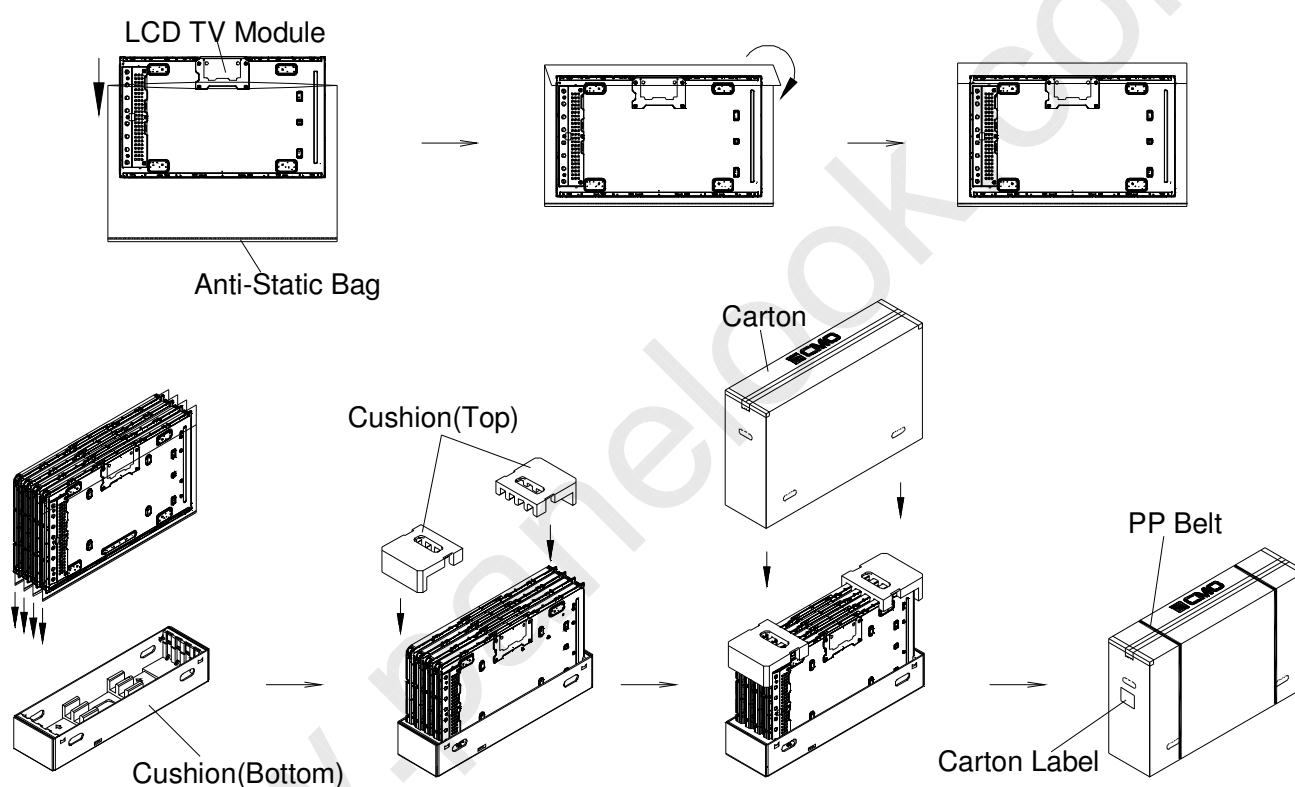
Figure 10-1 packing method
