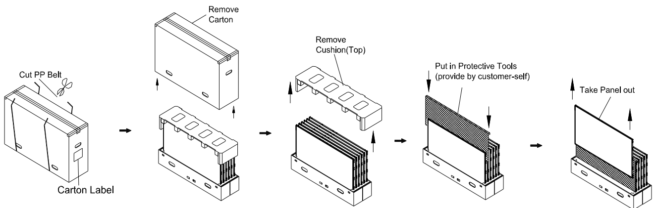
Figure 10-3 un-packing method
