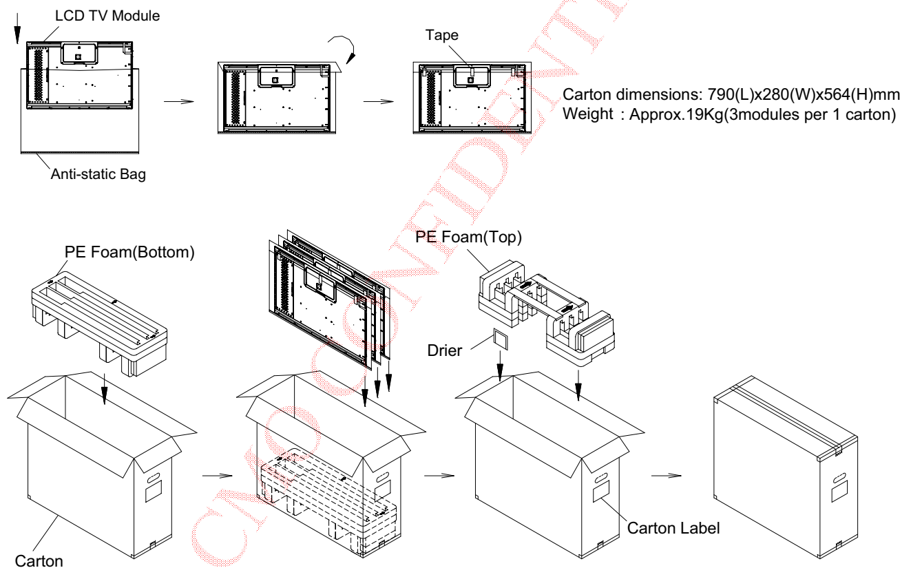
Figure.8-1 packing method
