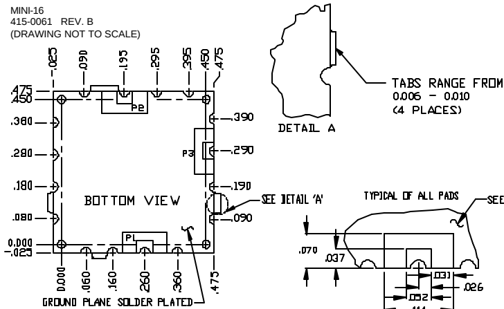
PHYSICAL DIMENSIONS
