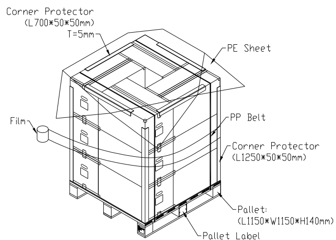
Figure. 9-2 Packing method
