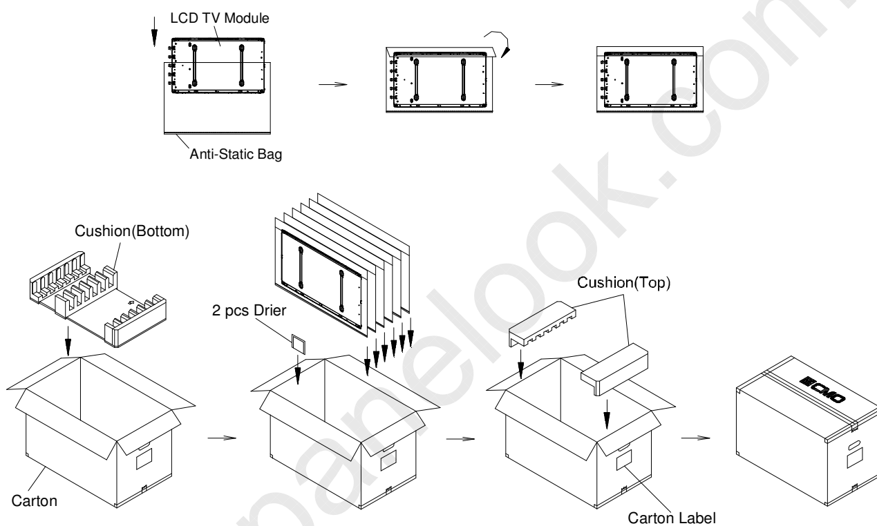
Figure.9-1 Packing Method
