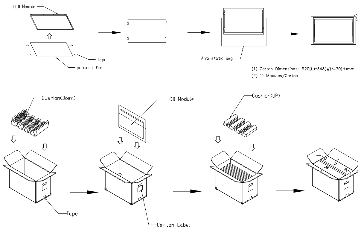
Figure 10-1 packing method
