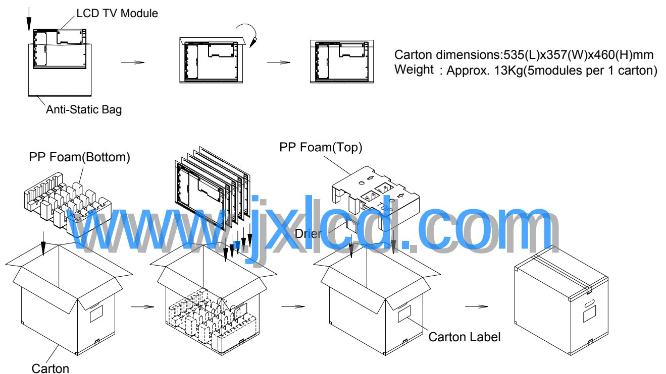
Figure.9-1 packing method
