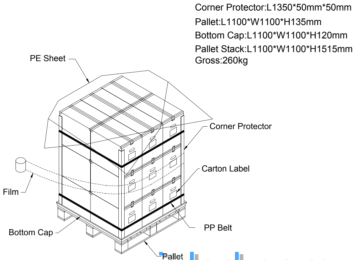
Figure. 9-2 Packing method
