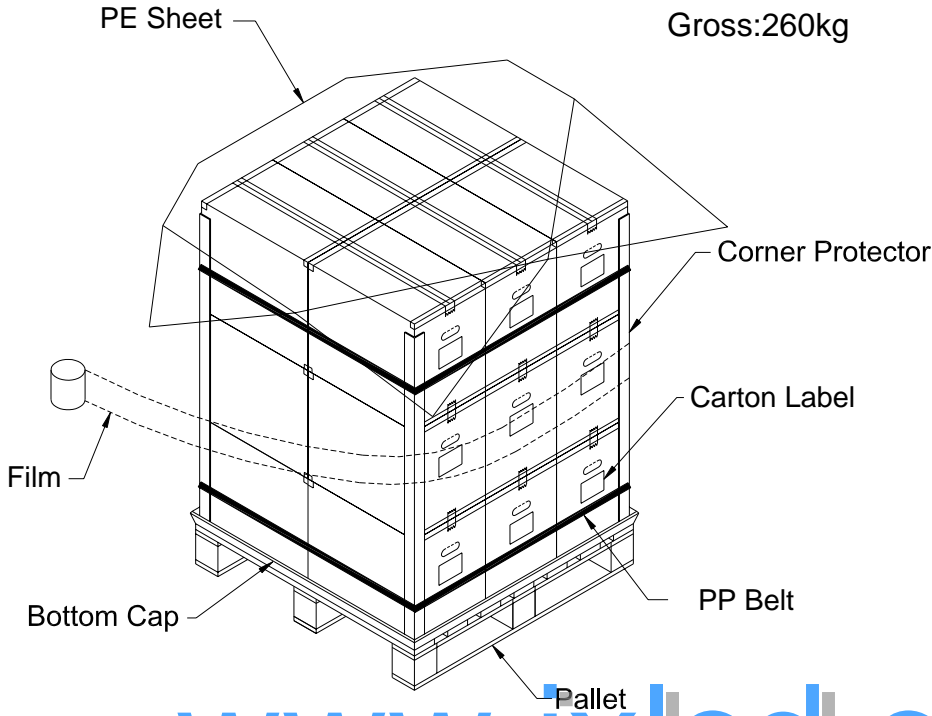
Figure. 9-2 Packing method
