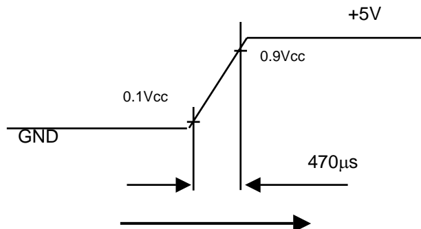
Vcc rising time is 470μs
