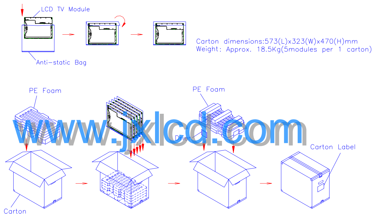
Figure.8-1 packing method
