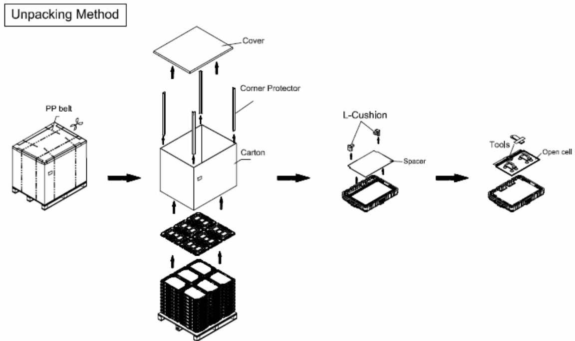
Figure 10-3 UN-packing method
