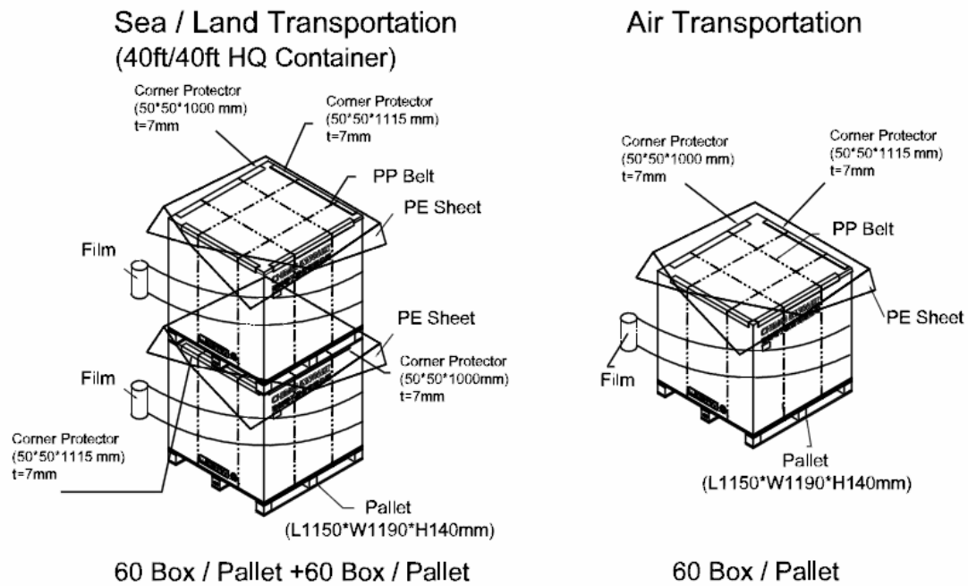
Figure 10-2 packing method
