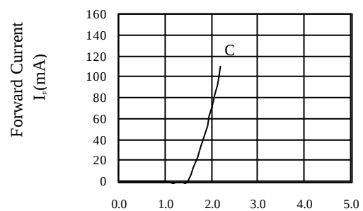
Forward Voltage (V) FIG.4 FORWARD CURRENT VS. FORWARD VOLTAGE
