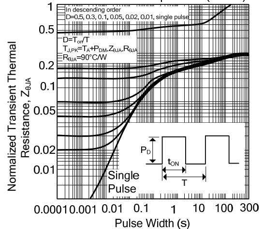
Figure 10: Normalized Maximum Transient Thermal Impedance (Note 6)
