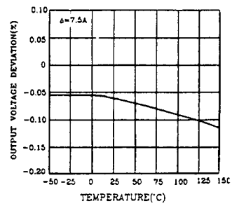
Load Regulation
