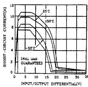
Short-Circuit Current
