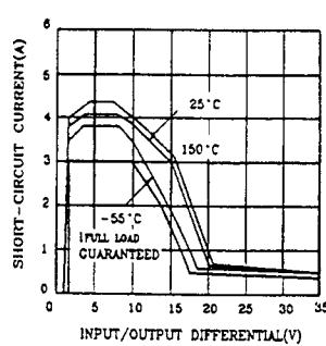
Short-Circuit Current
