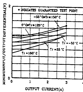
Dropout Voltage
