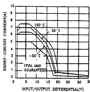
Short-Circuit Current
