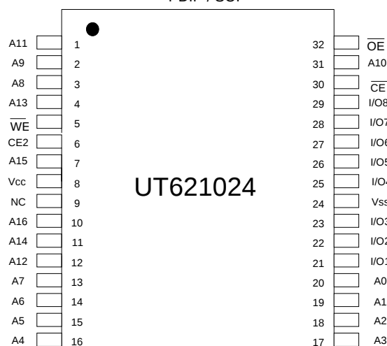
PDIP / SOP
