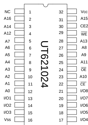
PDIP / SOP
