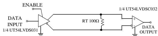
Figure 3. Point-to-Point Application
