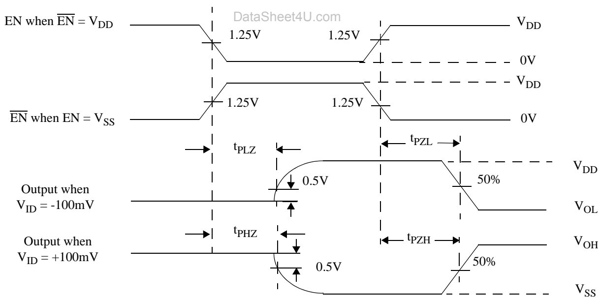
Figure 7. Receiver Three-State Delay Waveform
