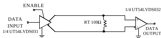
Figure 3. Point-to-Point Application
