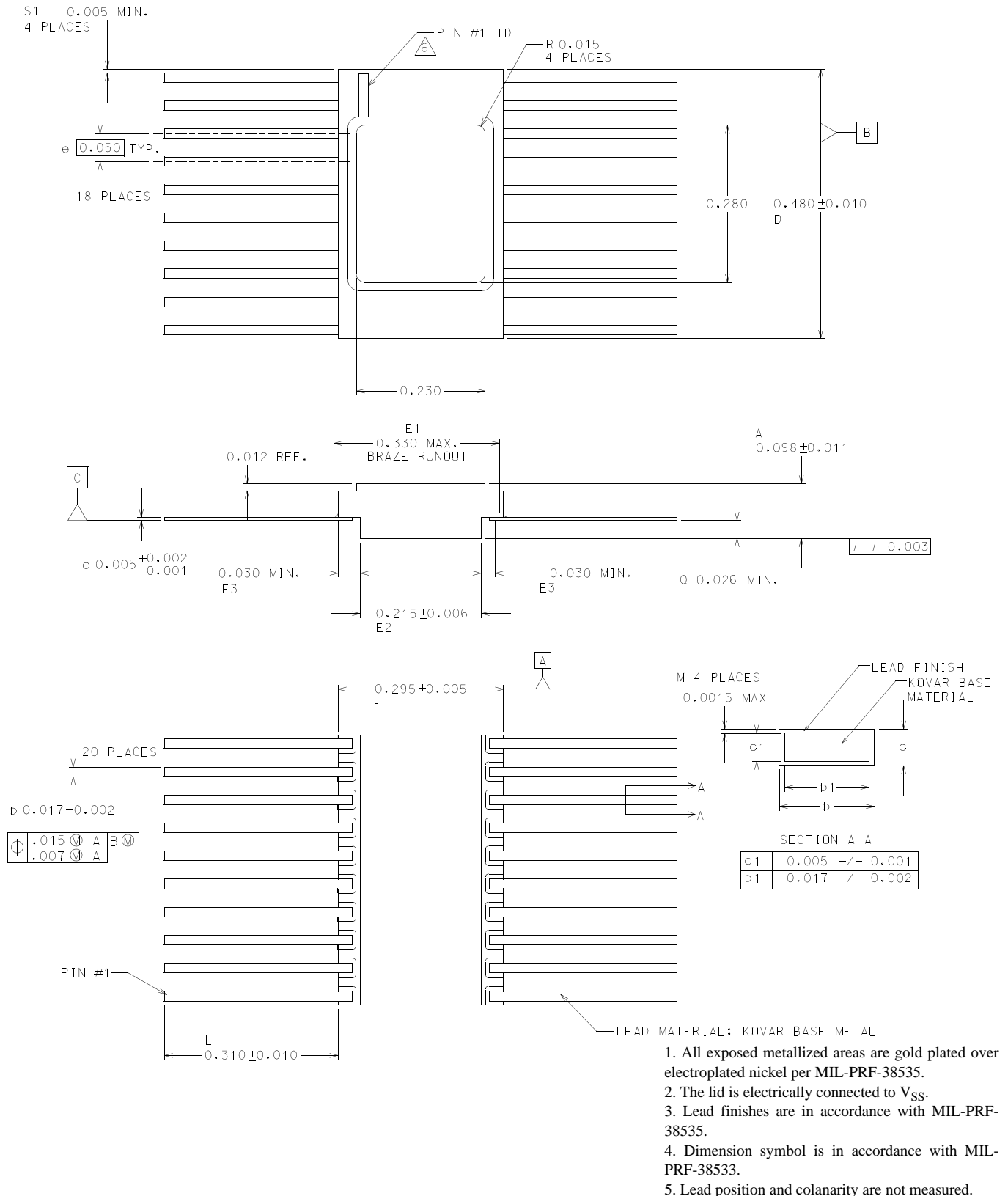
Figure 1. 20-lead Flatpack
