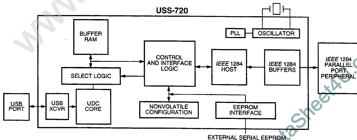
Figure 1. Block Diagram
