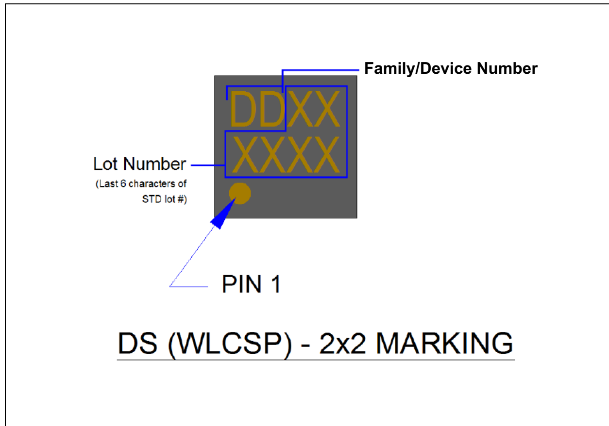
FIGURE 12-6: PACKAGE MARKING
