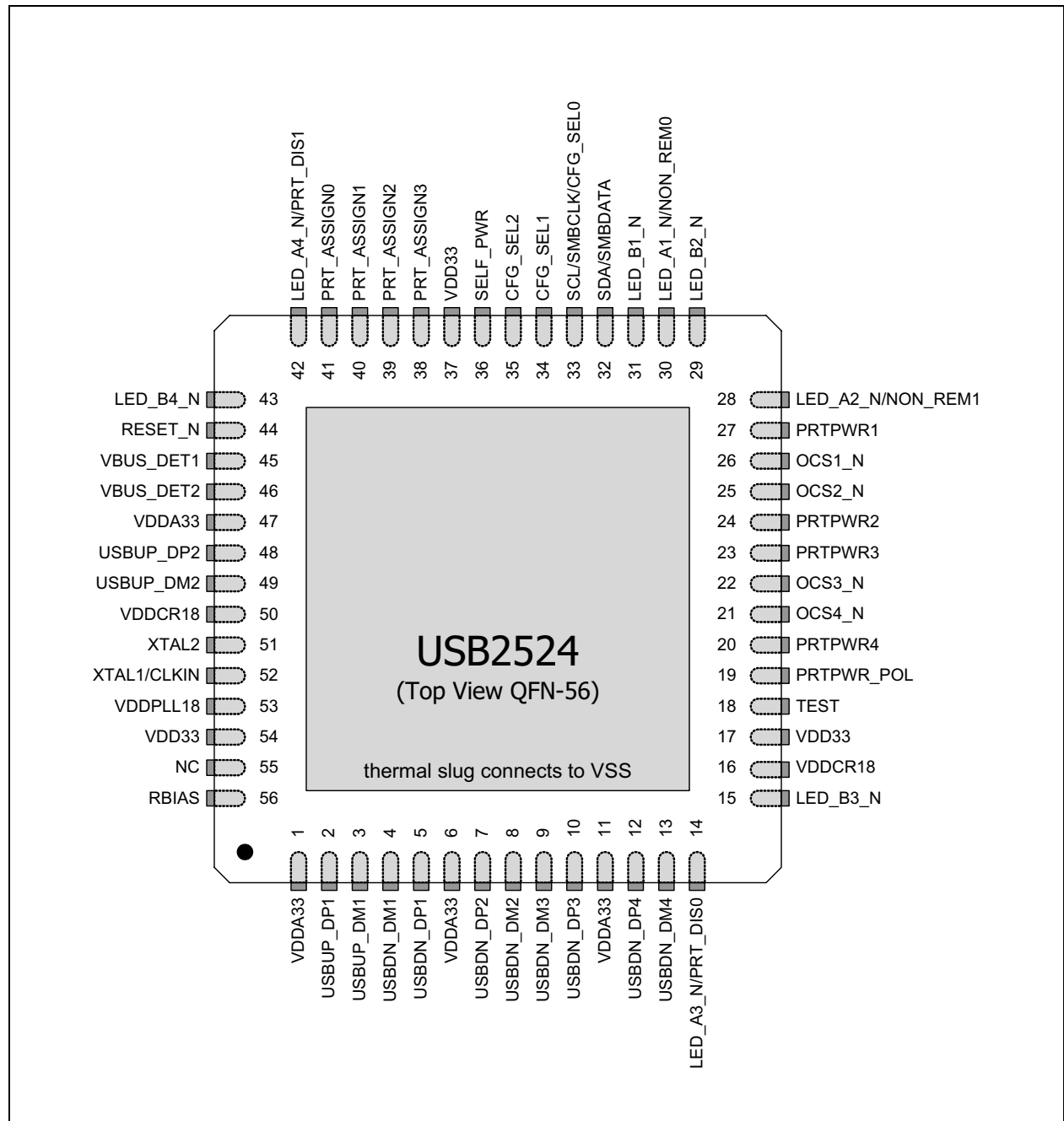
FIGURE 3-1: USB2524 QFN-56
