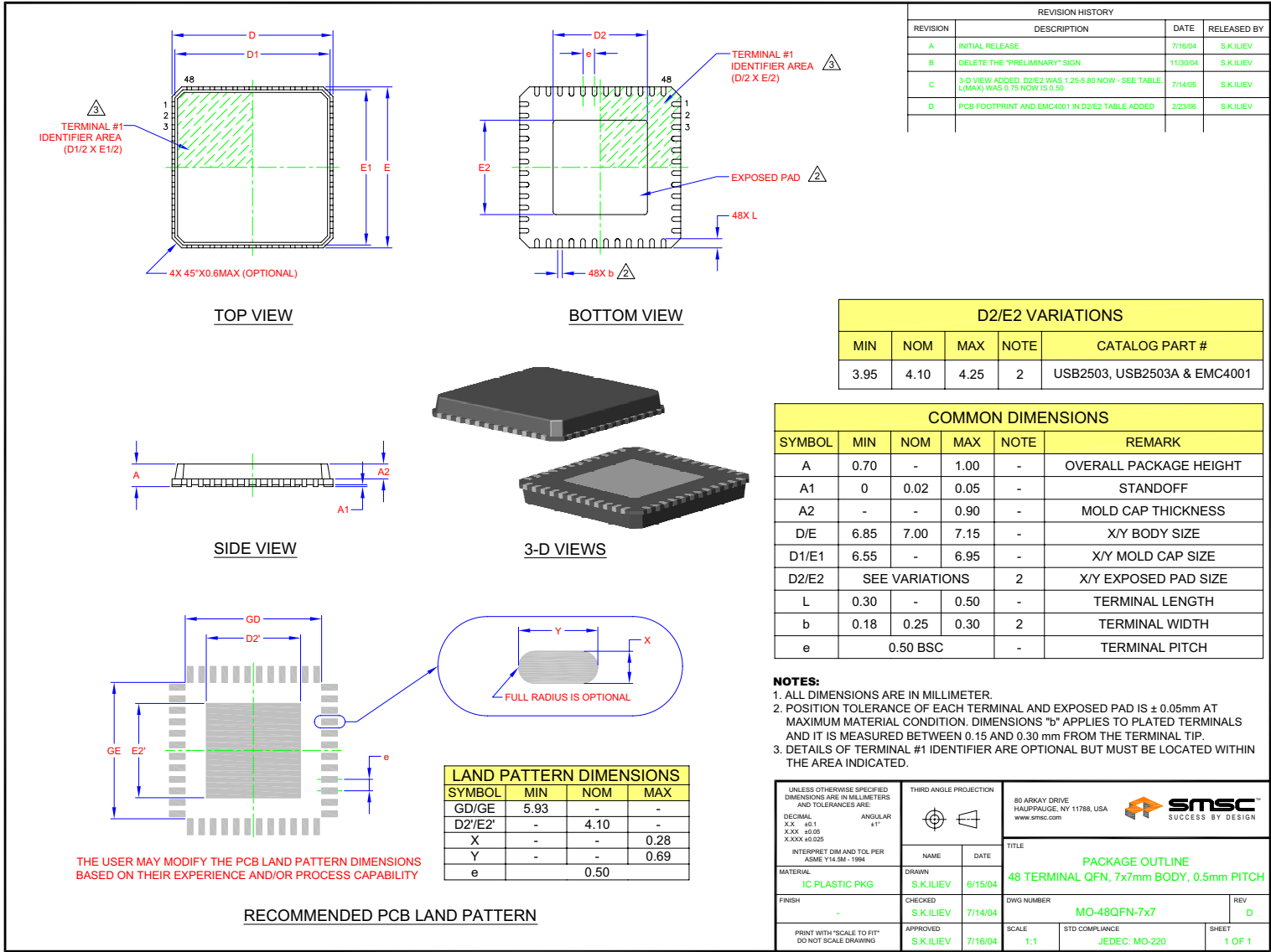
Figure 7.2 48-Pin QFN, 7x7mm Body, 0.5mm Pitch
