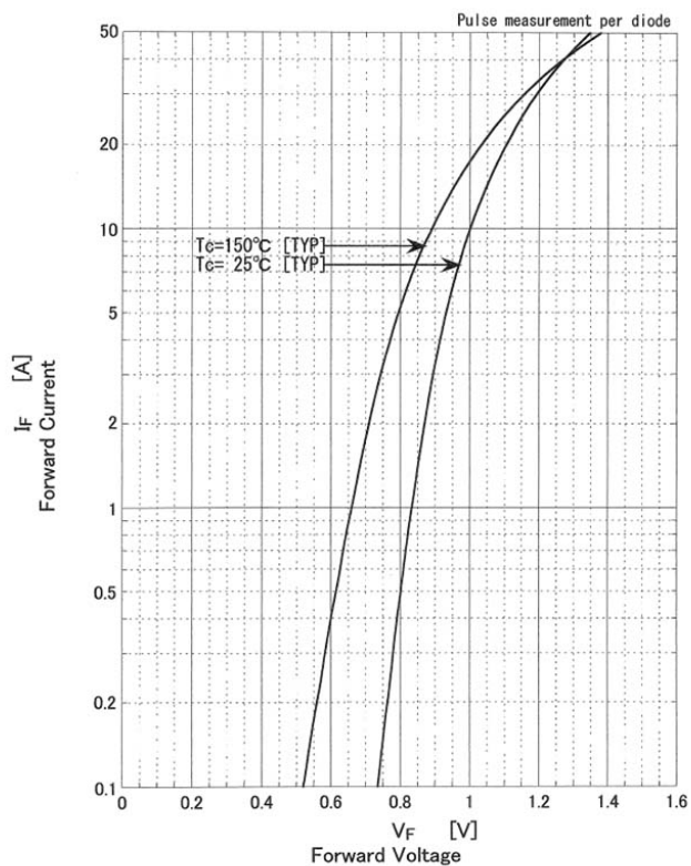
Forward Voltage
