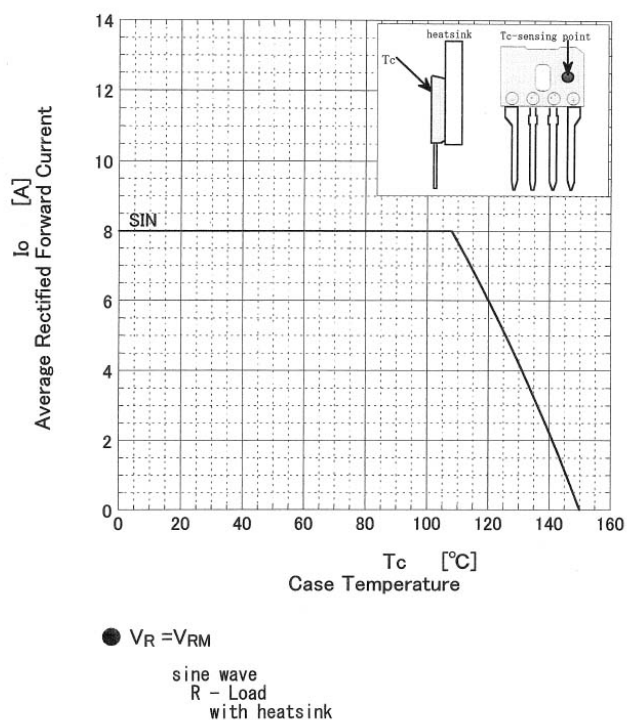
Derating Curve
