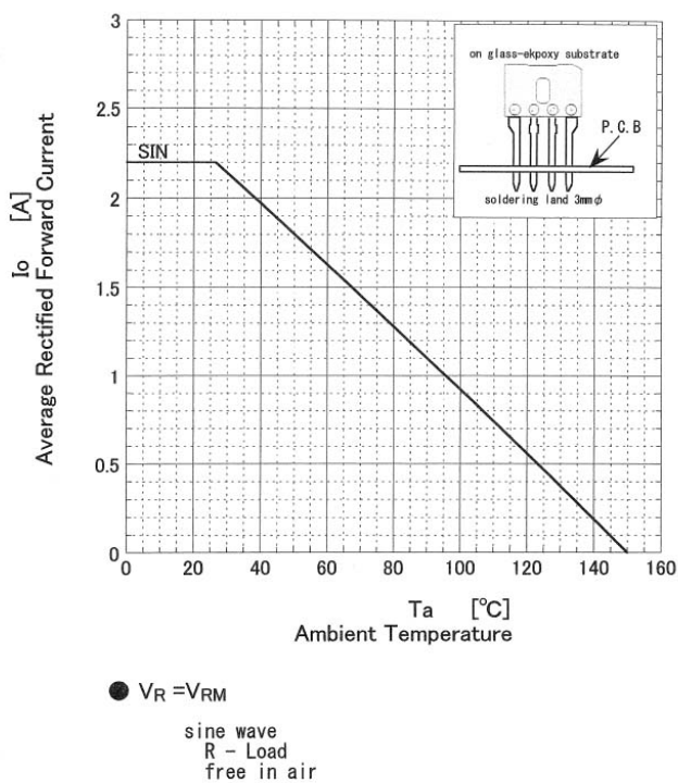
Derating Curve
