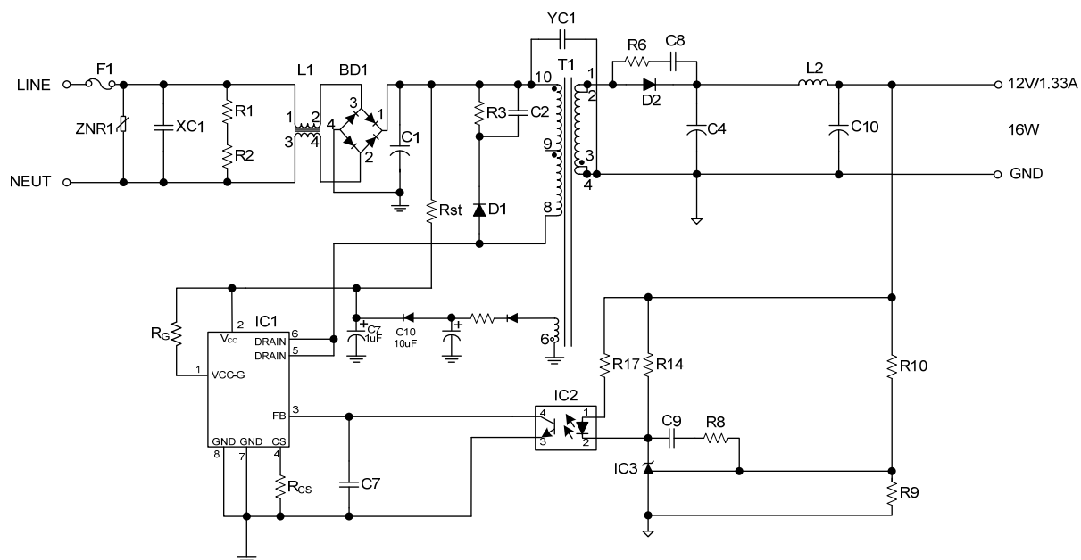
Fig.8 UTC US1602 Typical Application Circuit
