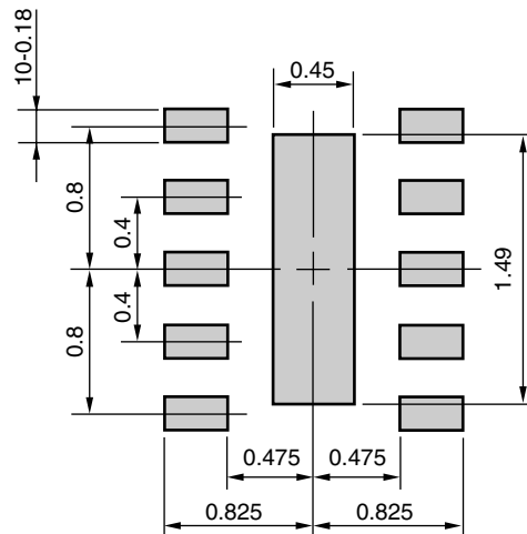
MOUNTING PAD
