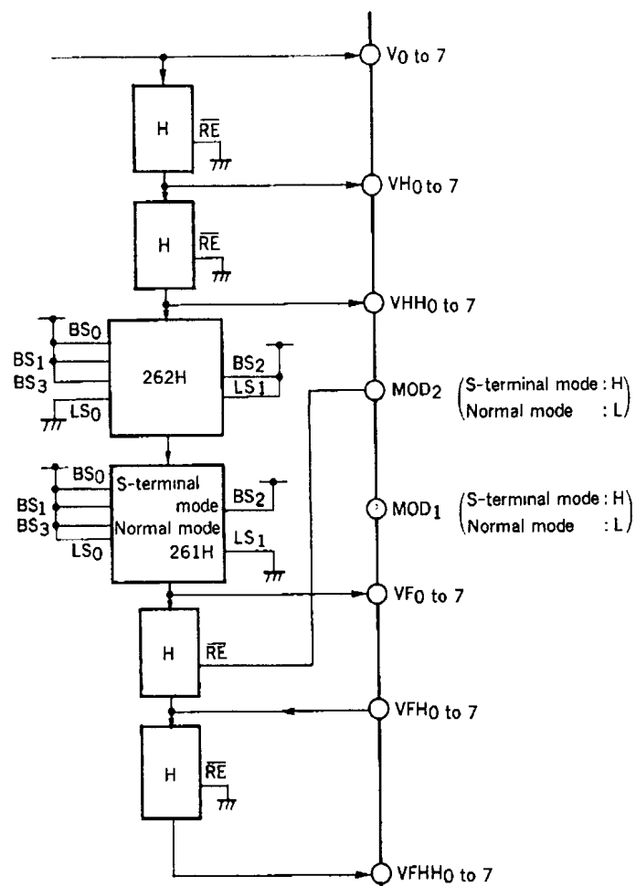
Fig. 4-3 Connection of Line and Field Buffers (Vertical contour compensation is acted)
