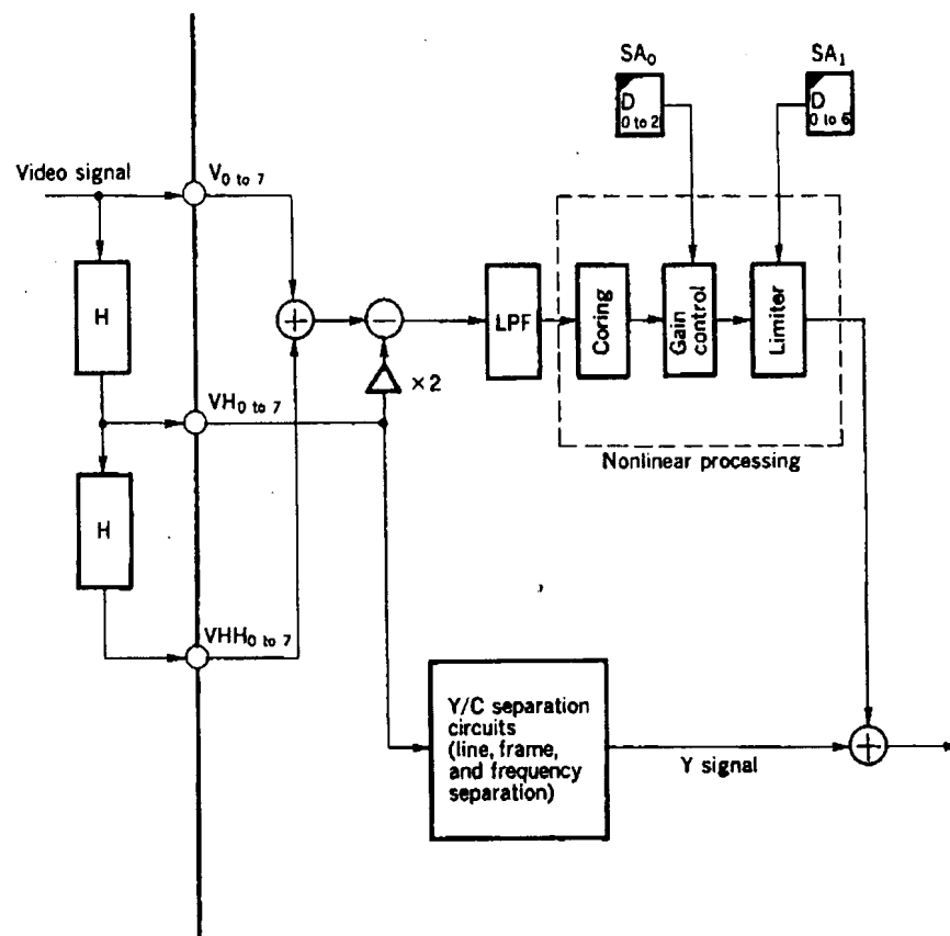
Fig. 4-2 Block Diagram of Vertical Aperture Compensation Circuit
