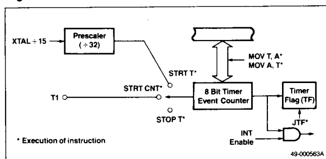
Figure 2. Timer/Event Counter
