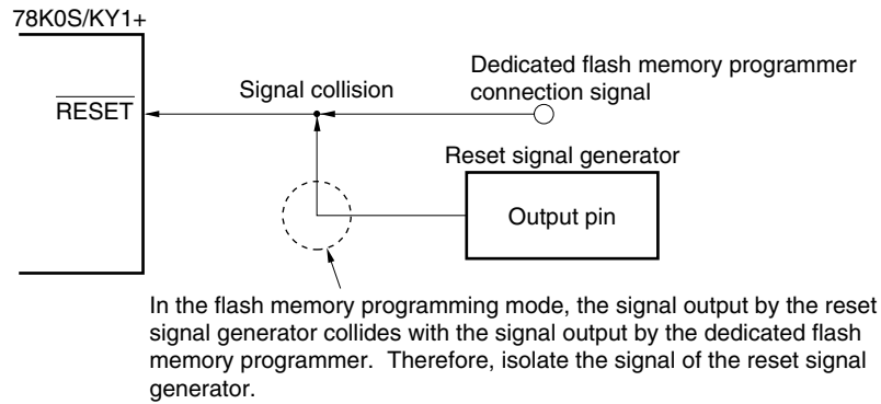
Figure 16-6. Signal Collision ( \overline{\text{RESET}} Pin)
