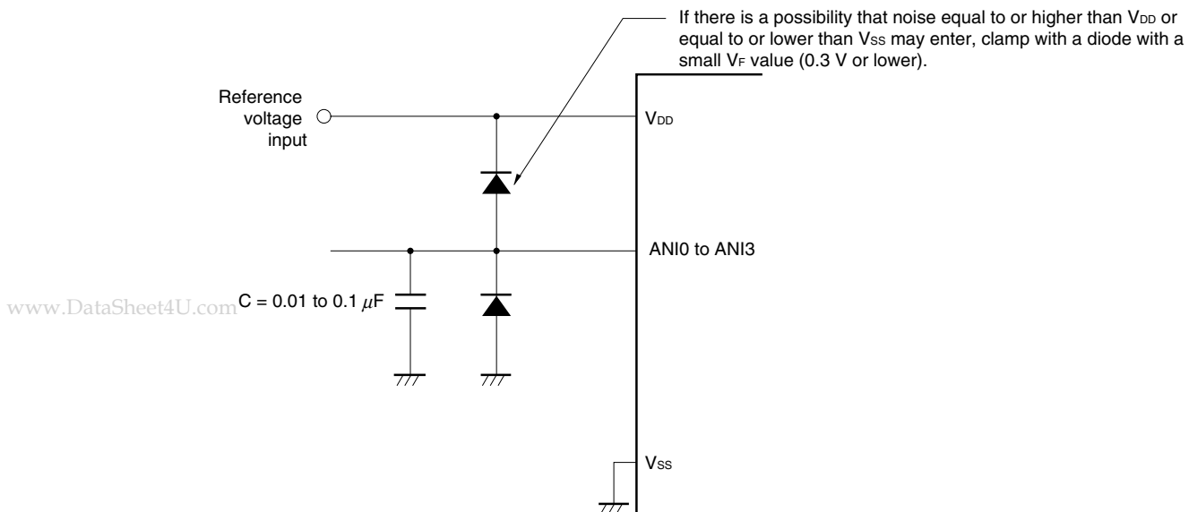
Figure 9-19. Analog Input Pin Connection
