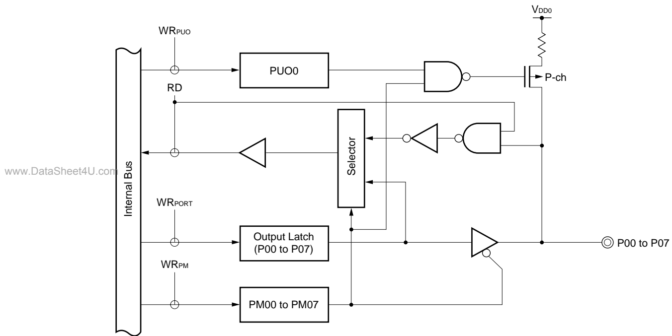
Figure 4-2. Block Diagram of P00 to P07
