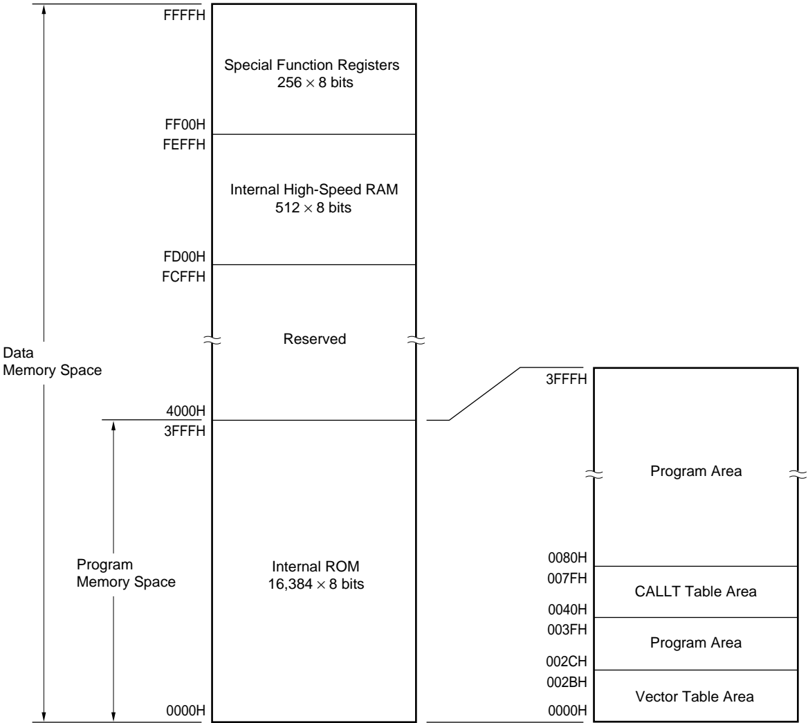
Figure 3-4. Memory Map (μPD789026)
