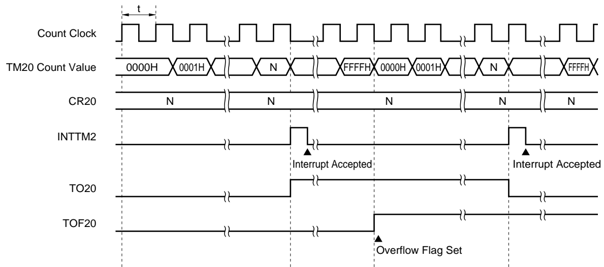
Figure 6-5. Timer Interrupt Operation Timing
