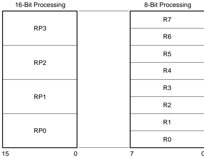
Figure 3-16. General-Purpose Register Configuration (a) Absolute Names
