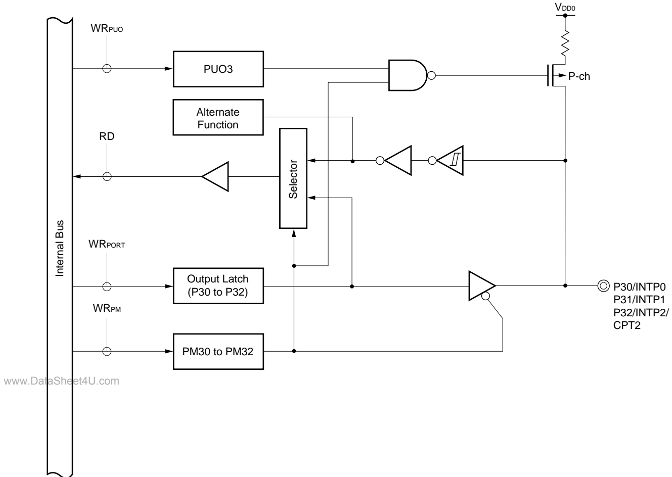
Figure 4-7. Block Diagram of P30 to P32
