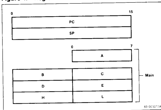
Figure 4. Registers
