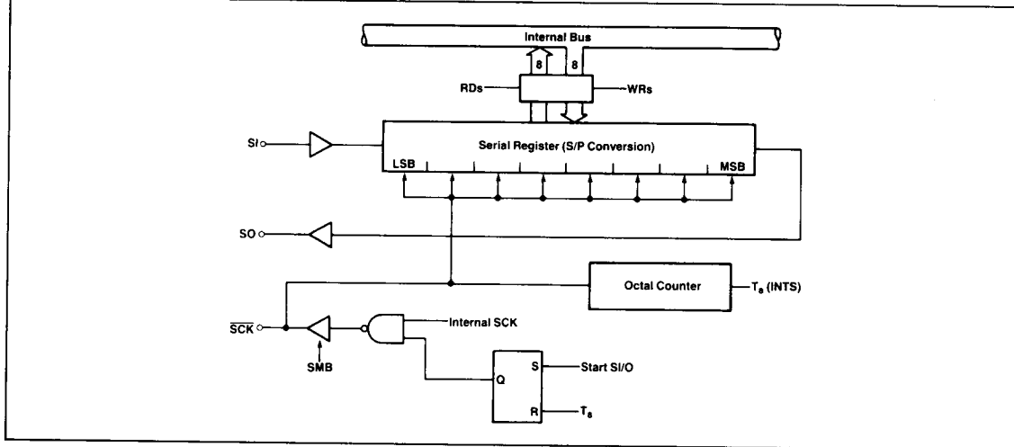
Figure 3. Serial Port Diagram
