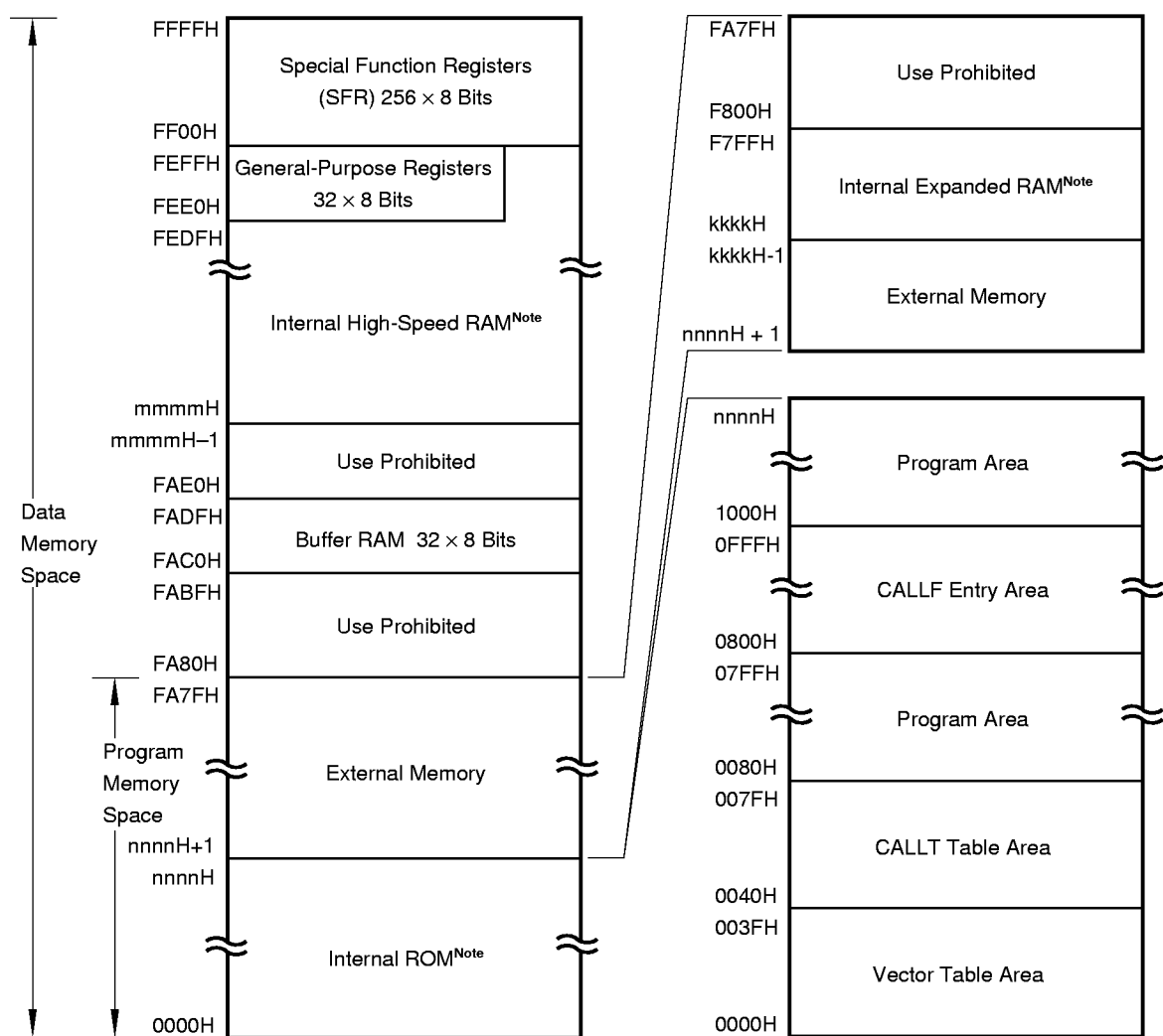
Figure 4-2. Memory Map ( \mu PD78015F(A), 78016F(A), 78018F(A))
