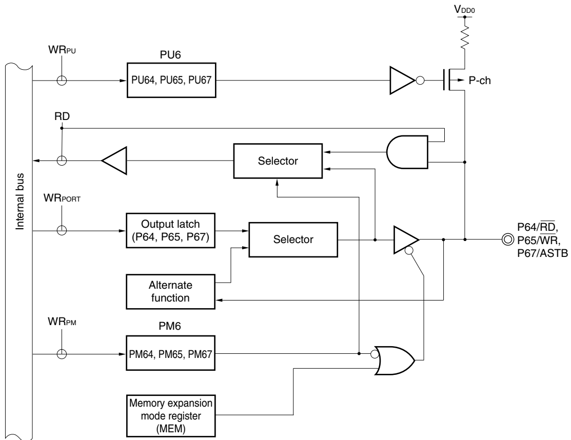
Figure 6-17. Block Diagram of P64, P65, and P67
