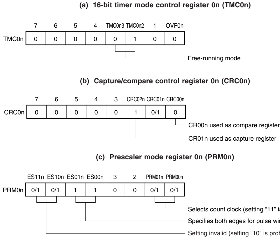
Figure 8-23. Control Register Settings for Pulse Width Measurement with Free-Running Counter and One Capture Register (When TI00n and CR01n Are Used)
