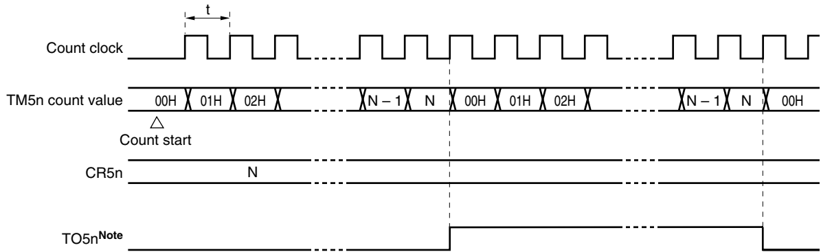
Figure 9-12. Square-Wave Output Operation Timing
