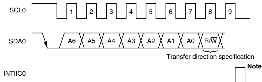
Figure 18-13. Transfer Direction Specification
