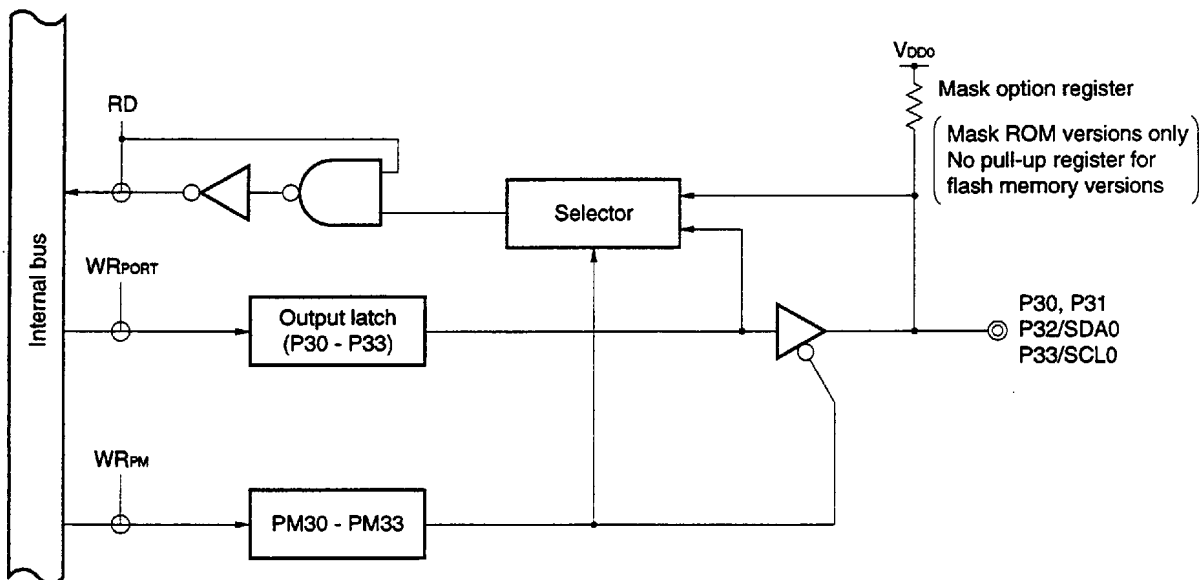
Figure 6-7. P30 to P33 Configurations ( \mu PD780024Y, 780034Y Subseries)
