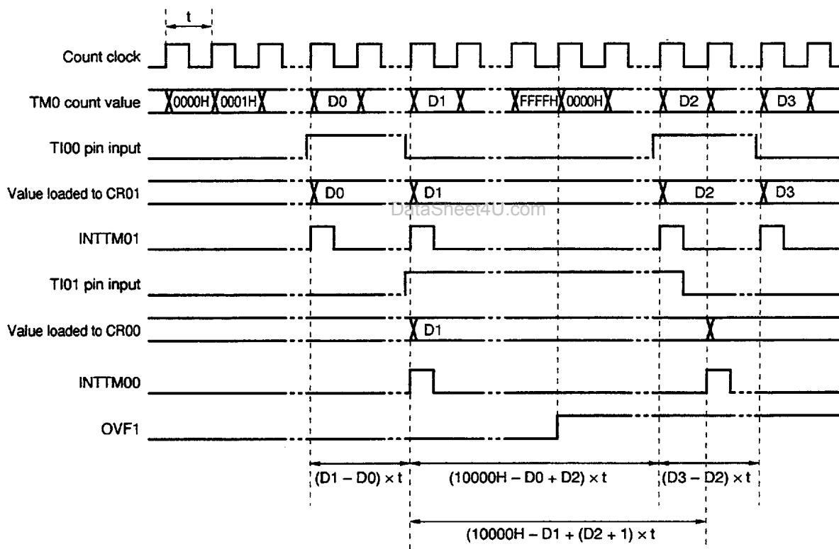
Figure 8-16. Timing of Pulse width Measurement operation with Free-Running Counter (with Both Edge specified)
