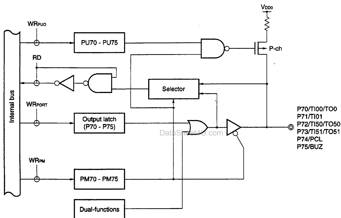
Figure 6-13. P70 to P75 Configurations
