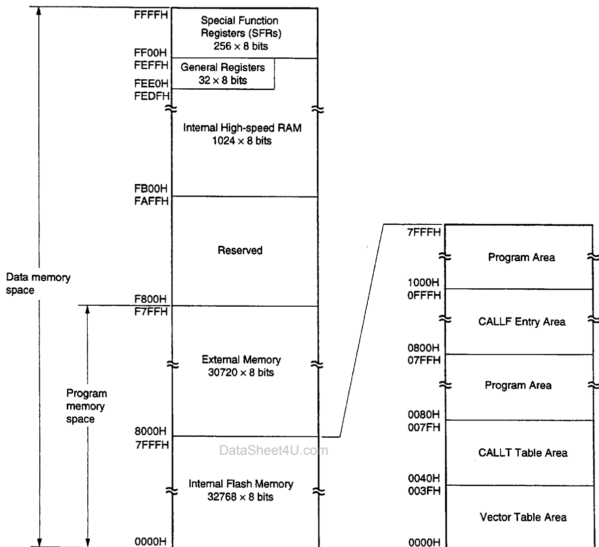
Figure 5-5. Memory Map ( \mu PD78F0034, 78F0034Y)
