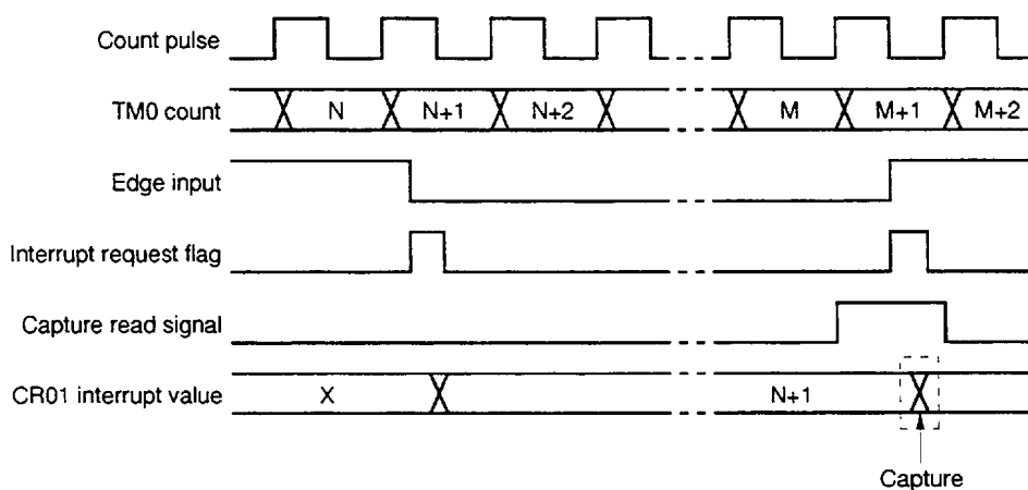
Figure 8-32. Capture Register Data Retention Timing
