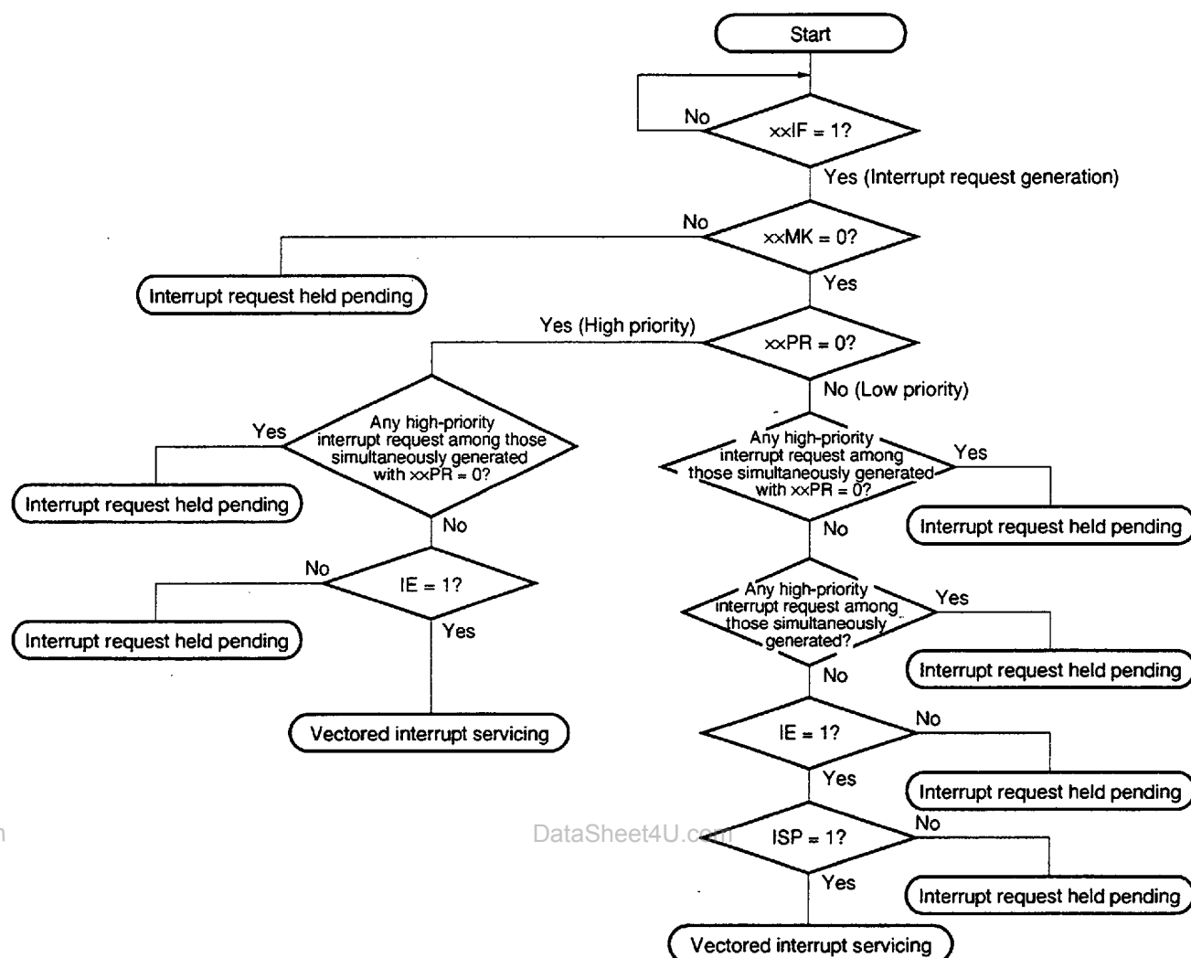
Figure 19-11. Interrupt Request Acknowledge Processing Algorithm
