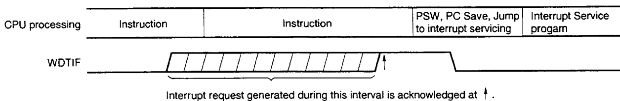
Figure 19-9. Non-Maskable Interrupt Request Acknowledge Timing
