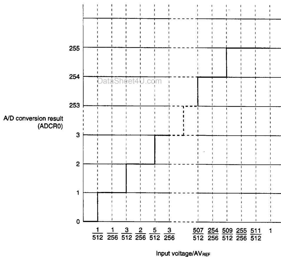
Figure 13-6. Relation between Analog Input Voltage and A/D Conversion Result
