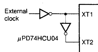
(b) External clock
