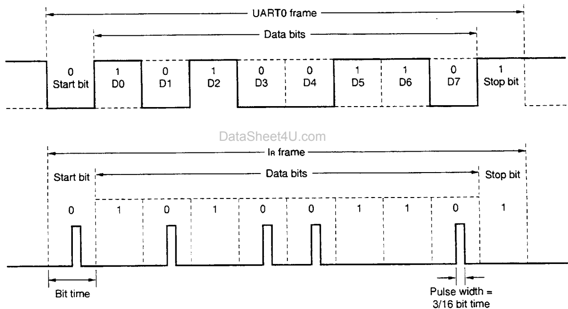
Figure 16-10. Data Format Comparison between IrDA0 Mode and UART0 Mode
