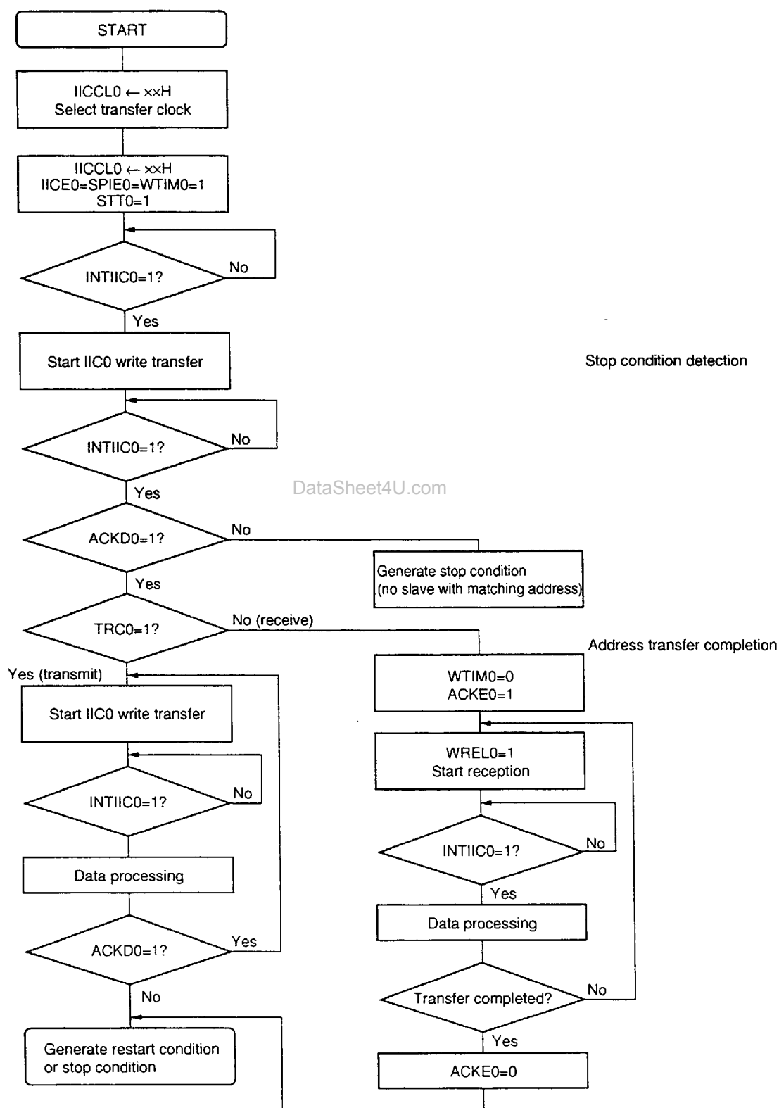
Figure 18-18. Master Operation Flow Chart
