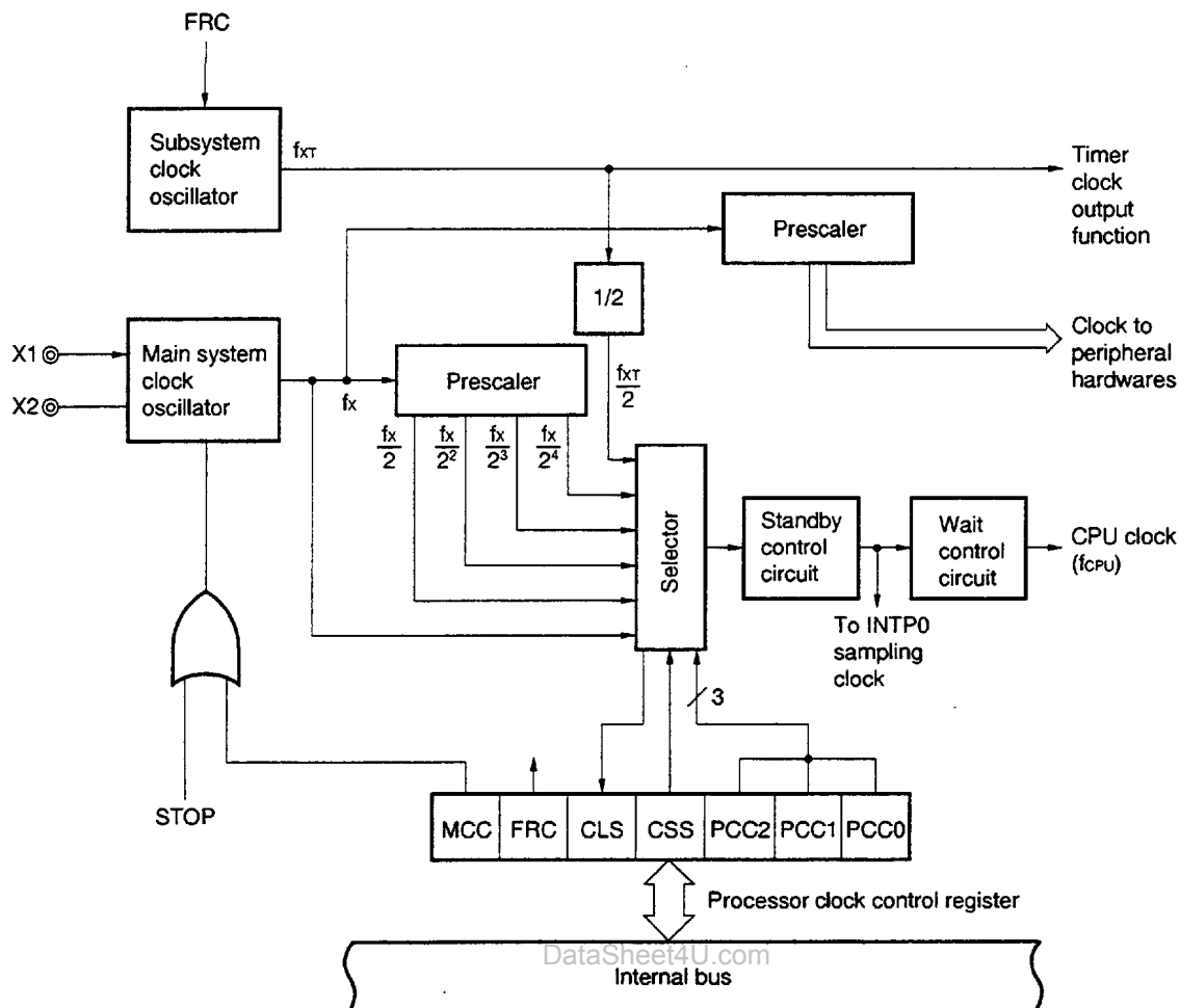
Figure 7-1. Block Diagram of Clock Generator
