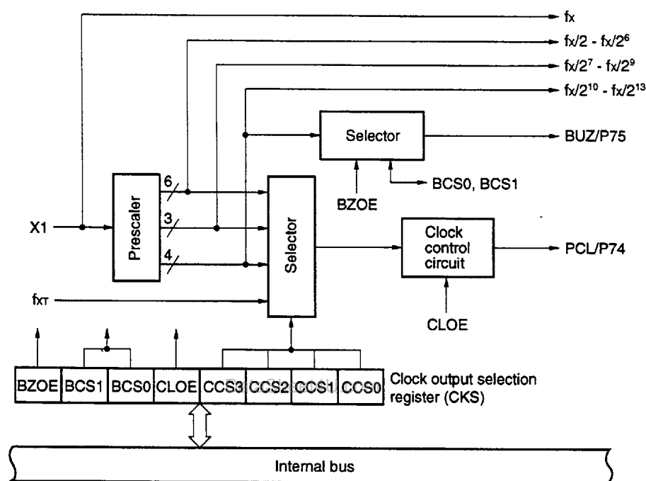
Figure 12-1. CKU Block Diagram
