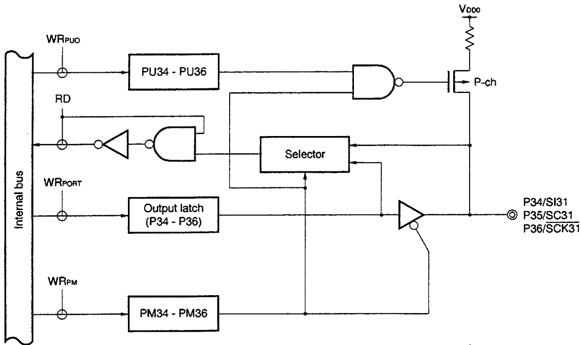
Figure 6-6. P34 to P36 Configurations ( \mu PD780024, 780034 Subseries)
