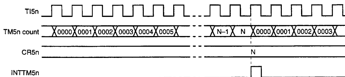
Figure 9-8. External Event Counter Operation Timings (with Rising Edge Specified)
