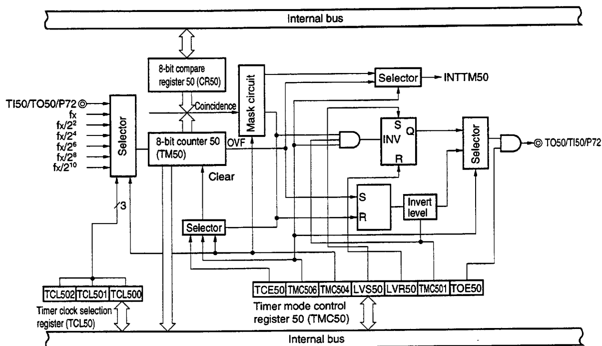
Figure 9-1. Block Diagram of TM50
