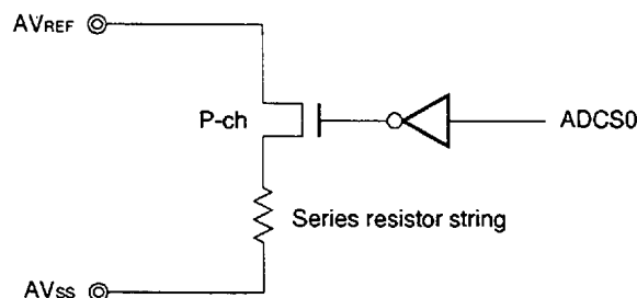
Figure 14-9. Example of Method of Reducing Power Dissipation in Standby Mode
