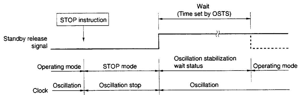
Figure 21-4. STOP Mode Release by Interrupt Generation
