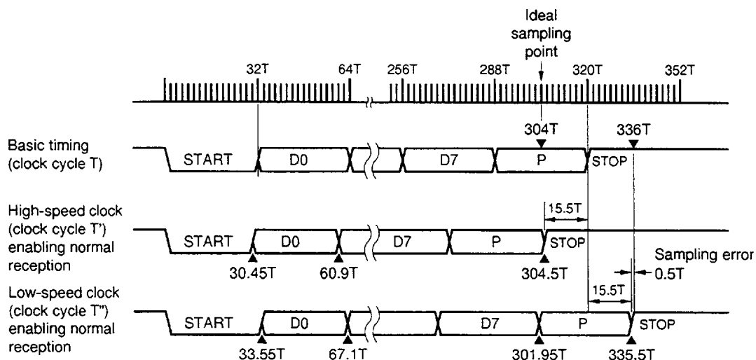
Figure 16-5. Error Tolerance (when k = 0 ), including Sampling Errors
