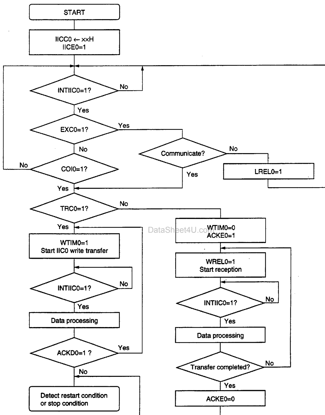
Figure 18-19. Slave Operation Flow Chart
