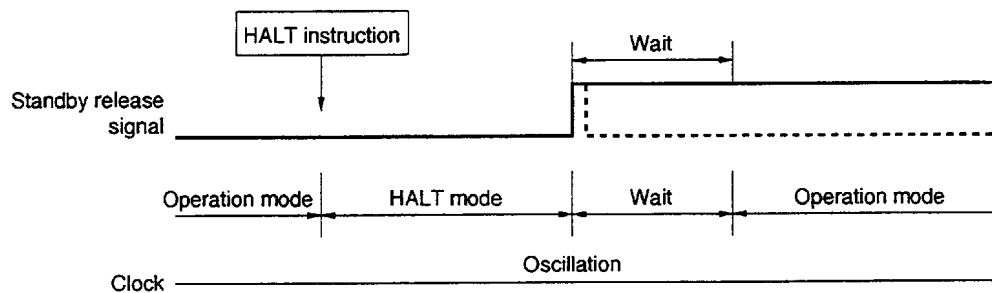
Figure 21-2. HALT Mode Clear Upon Interrupt Generation
