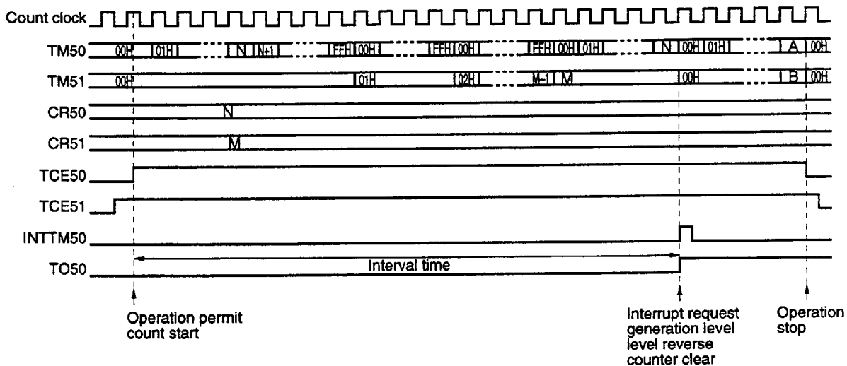
Figure 9-11. 16-bit Solution Cascade Connection Mode
