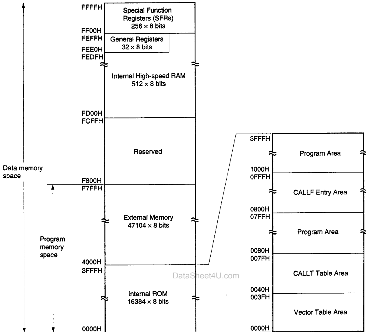
Figure 5-2. Memory Map ( \mu PD780022, 780032, 780022Y, 780032Y)
