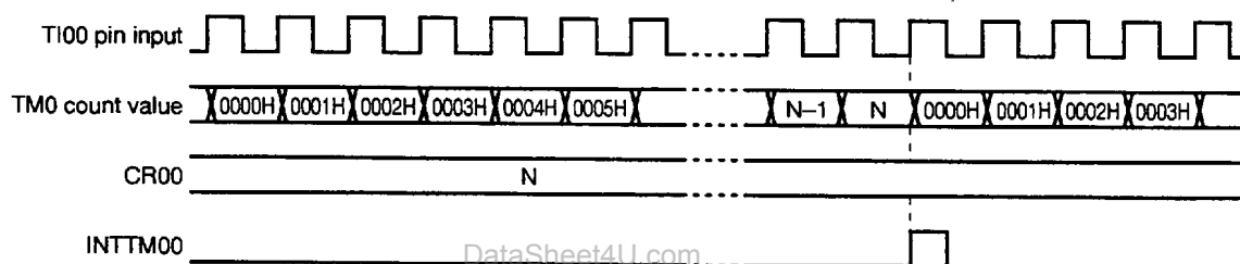
Figure 8-23. External Event Counter Operation Timings (with Rising Edge Specified)
