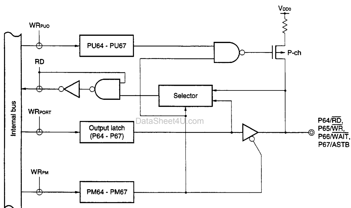
Figure 6-12. P64 to P67 Configurations
