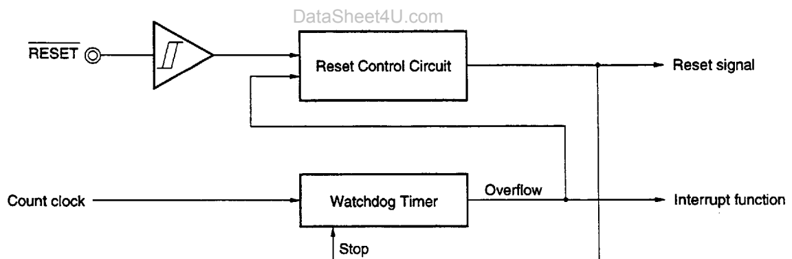
Figure 22-1. Block Diagram of Reset Function
