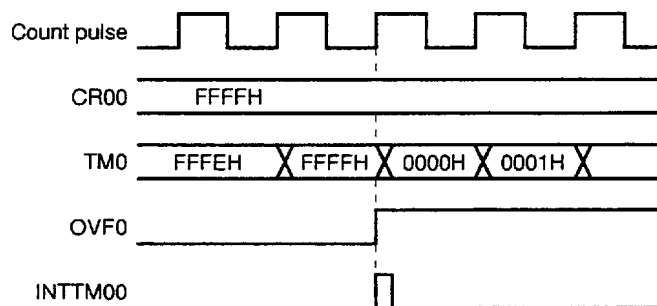
Figure 8-33. Operation Timing of OVF0 Flag
