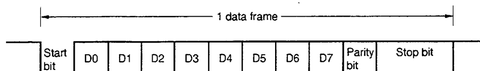
Figure 16-6. Format of Transmit/Receive Data in Asynchronous Serial Interface
