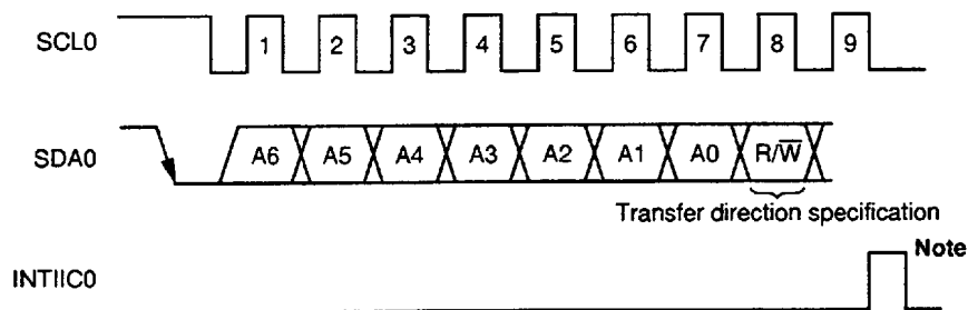
Figure 18-10. Transfer Direction Specification
