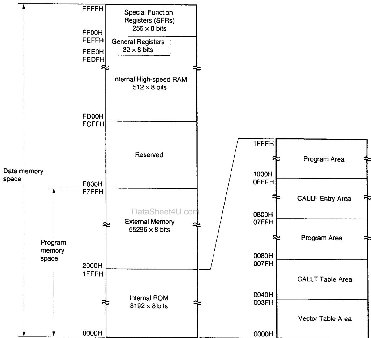
Figure 5-1. Memory Map ( \mu PD780021, 780031, 780021Y, 780031Y)
