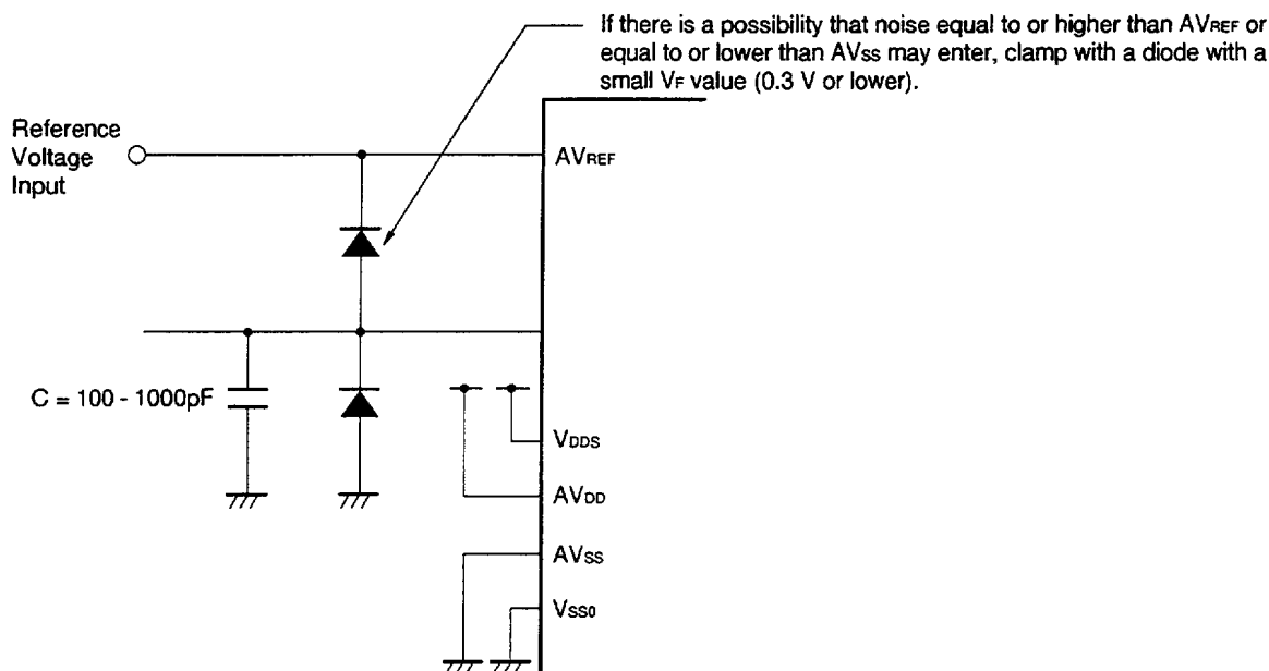
Figure 14-10. Analog Input Pin Handling
