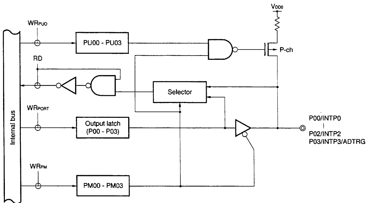
Figure 6-2. P00 and P03 Configurations
