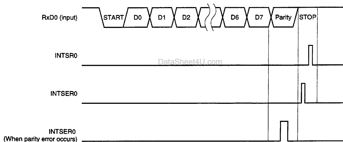
Figure 16-9. Receive Error Timing
