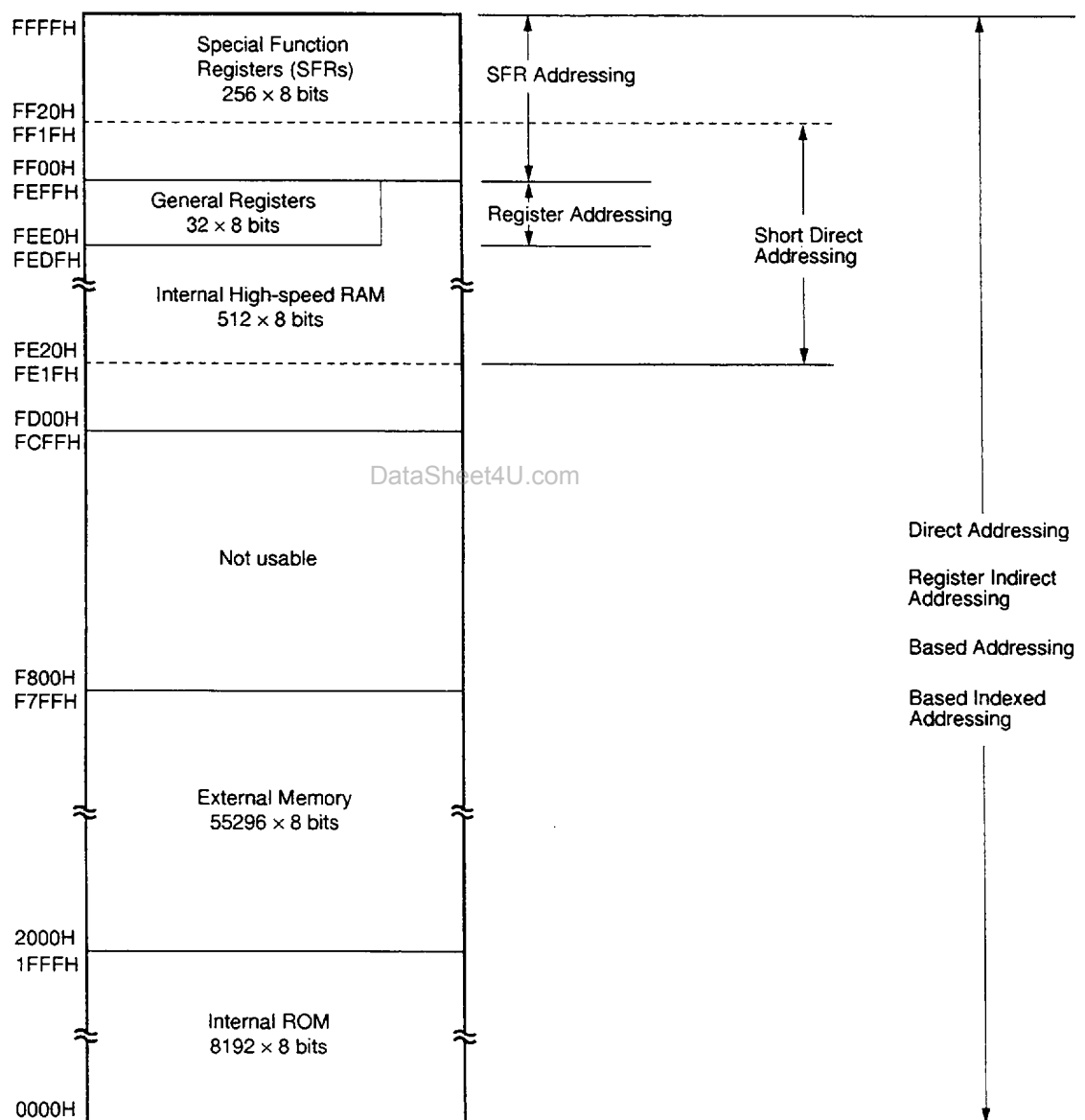
Figure 5-6. Data Memory Addressing ( \mu PD780021, 780031, 780021Y, 780031Y)
