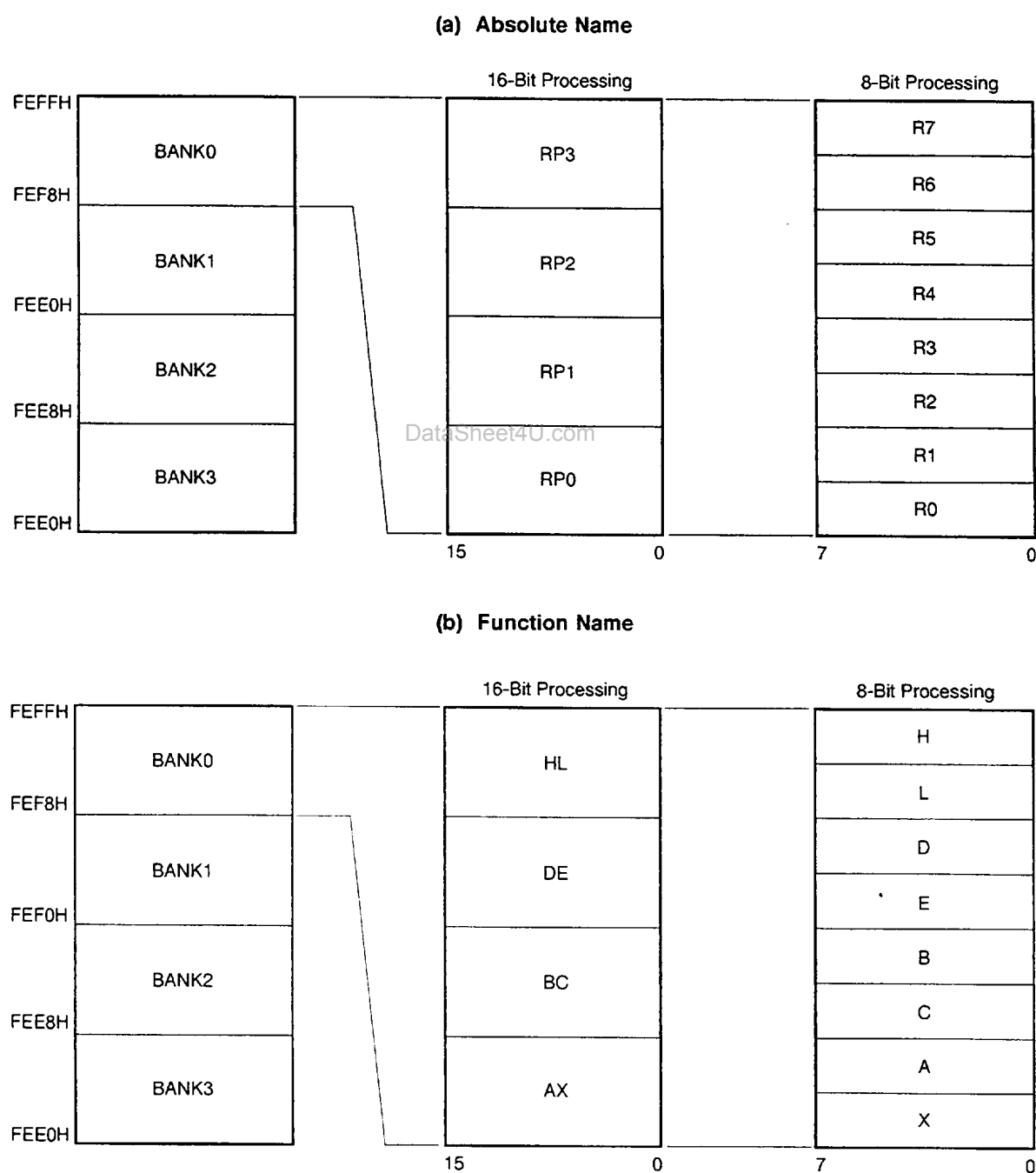
Figure 5-16. General Register Configuration
