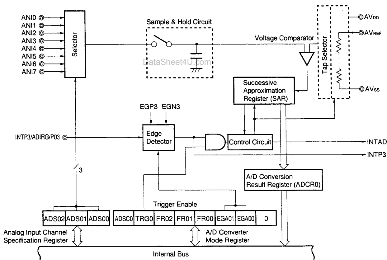
Figure 14-1. AD0 Block Diagram
