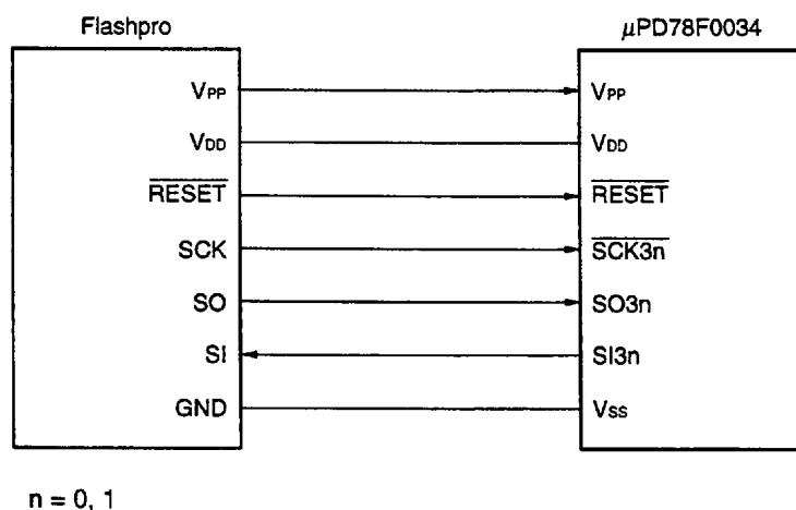
Figure 23-3. Connection of Flashpro Using 3-Wire Serial I/O Method
