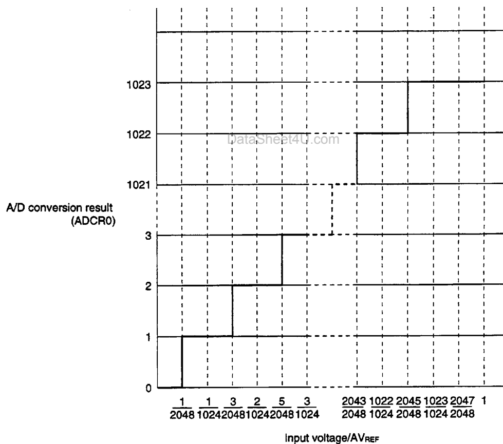
Figure 14-6. Relation between Analog Input Voltage and A/D Conversion Result
