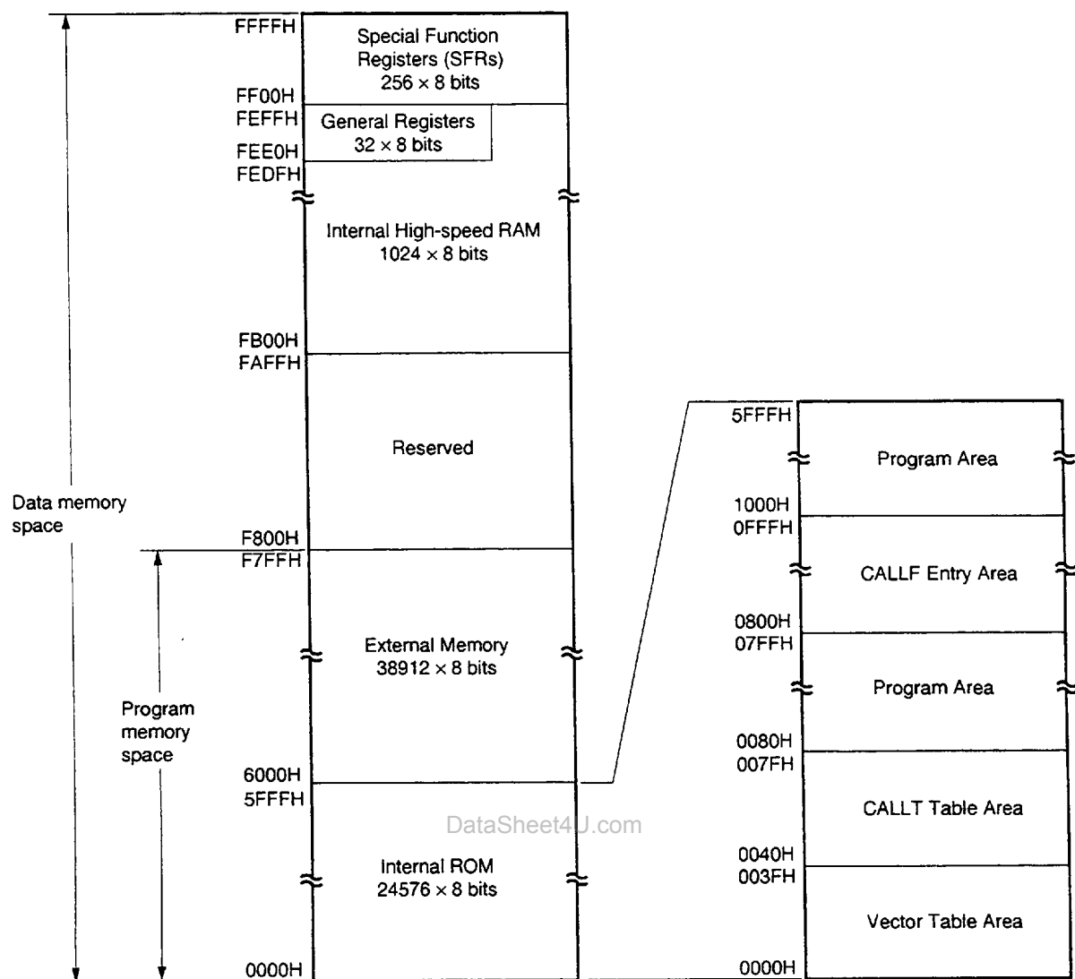
Figure 5-3. Memory Map ( \mu PD780023, 780033, 780023Y, 780033Y)
