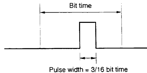
Figure 16-10. Data Format Comparison between IrDA0 Mode and UART0 Mode
