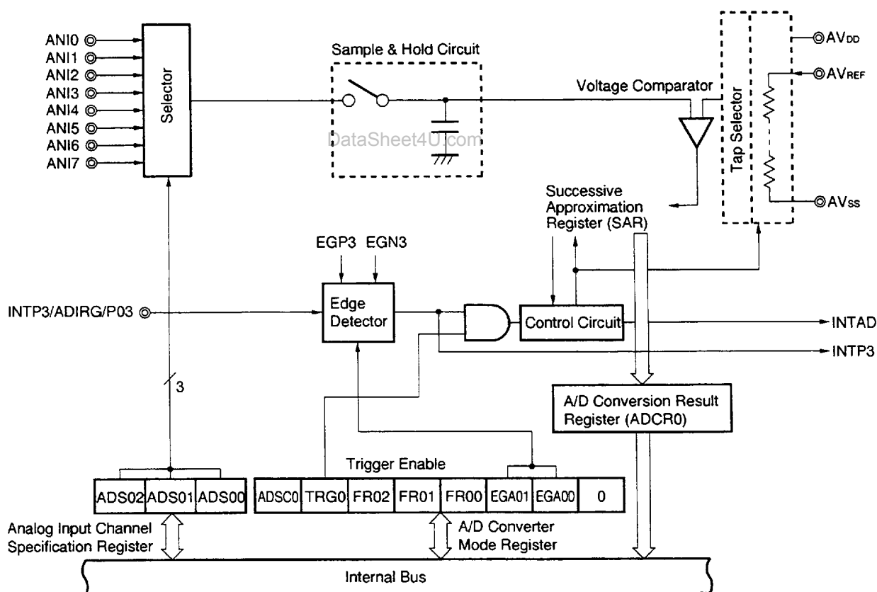
Figure 13-1. AD1 Block Diagram
