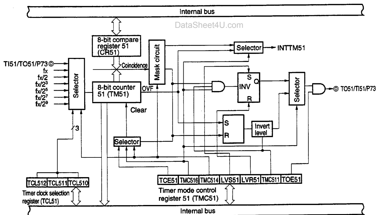
Figure 9-2. Block Diagram of TM51
