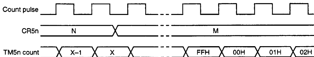
Figure 9-13. Timing after Compare Register Change during Timer Count Operation
