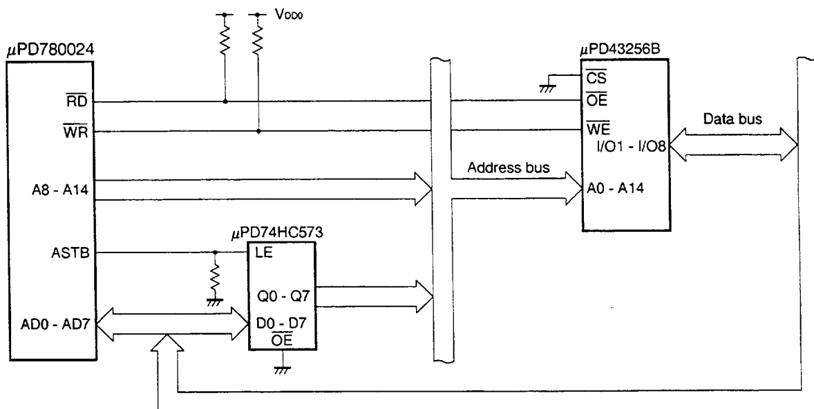
Figure 20-8. Connection Example of \mu PD780024 and Memory
