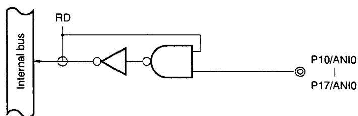
Figure 6-3. P10 to P17 Configurations
