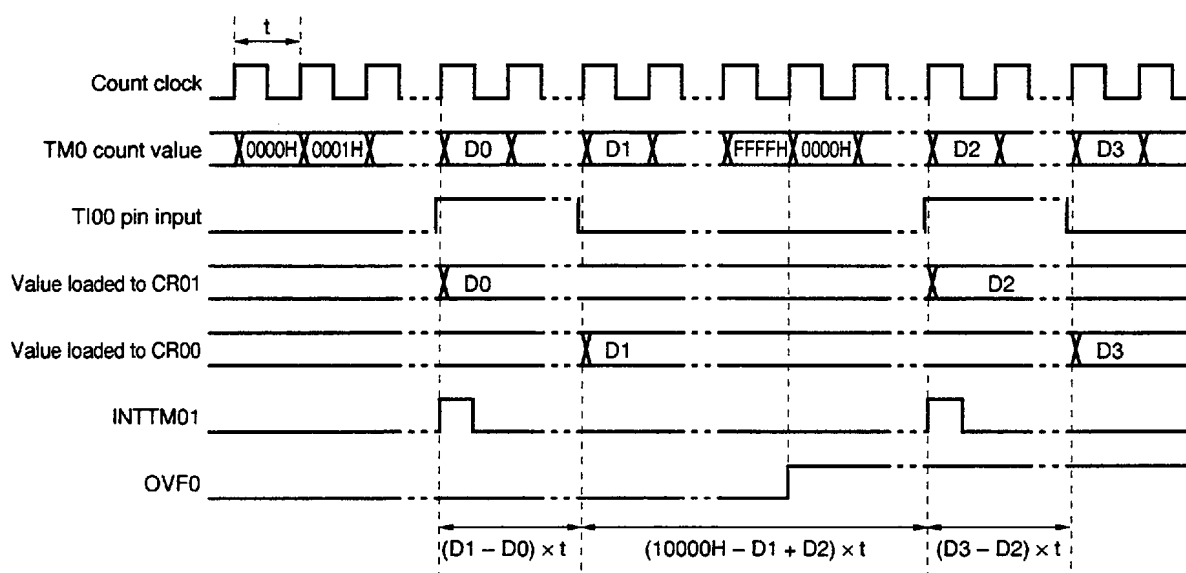
Figure 8-18. Timing of Pulse Width Measurement Operation by Free-Running Counter and Two Capture Registers (with Rising Edge Specified)
