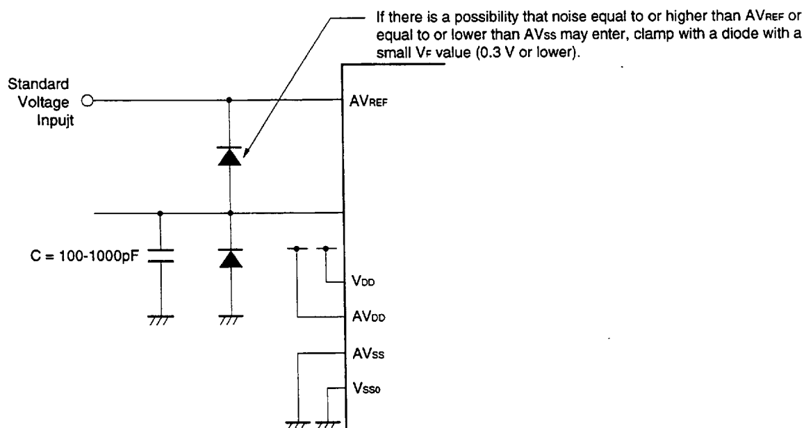
Figure 13-10. Analog Input Pin Handling
