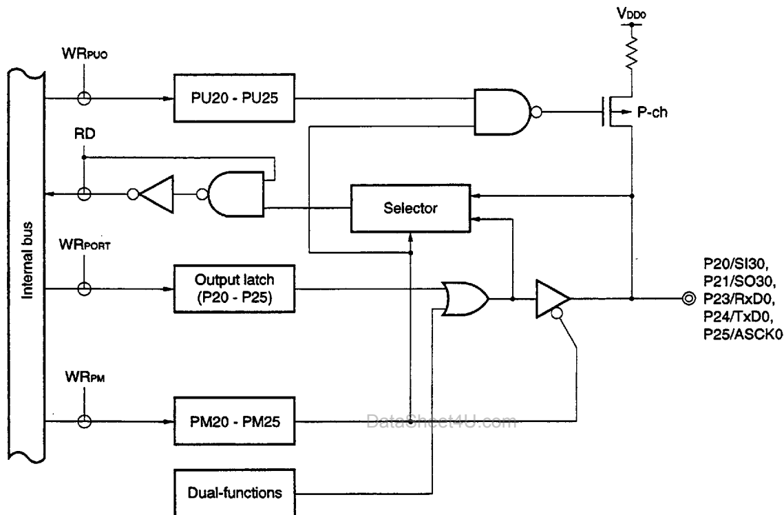
Figure 6-4. P20 to P25 Configurations
