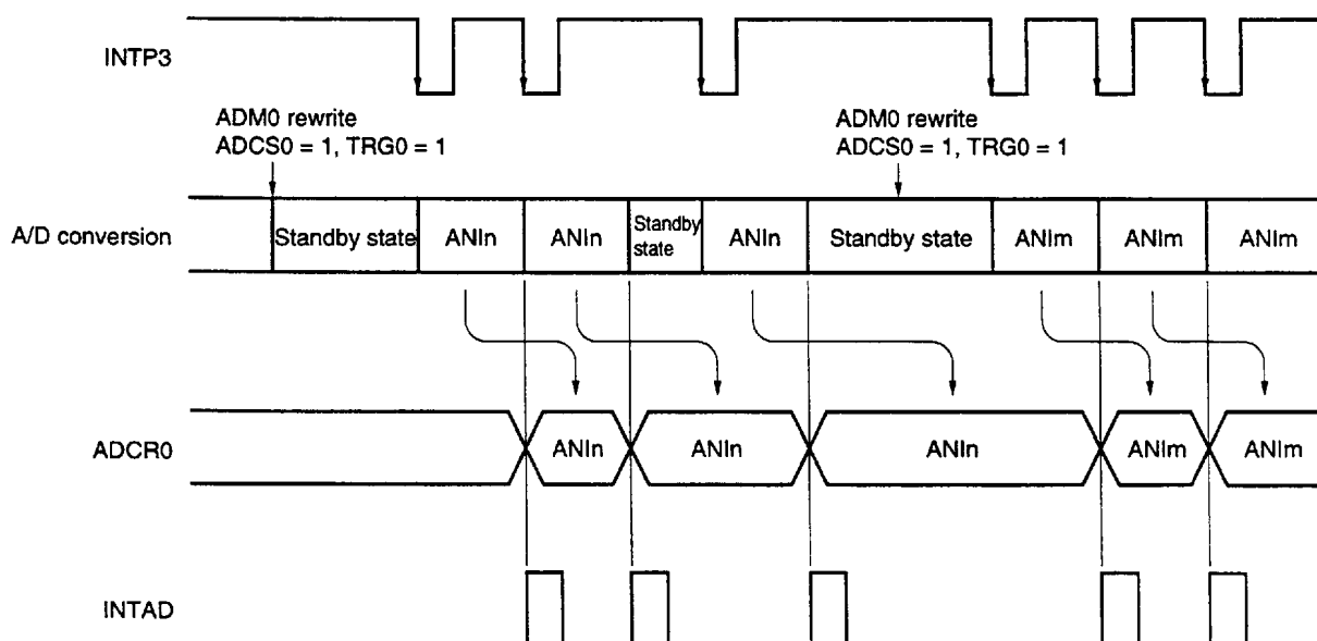
Figure 14-7. A/D Conversion by Hardware Start (When Falling Edge is Specified)
