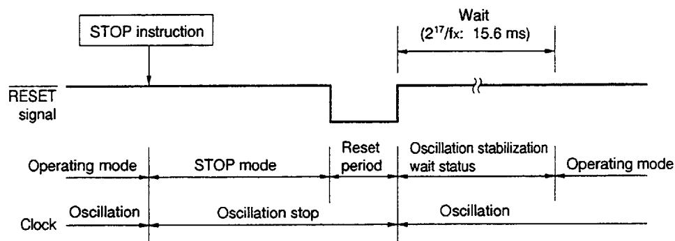
Figure 21-5. Release of STOP Mode \overline{\text{RESET}} Input
