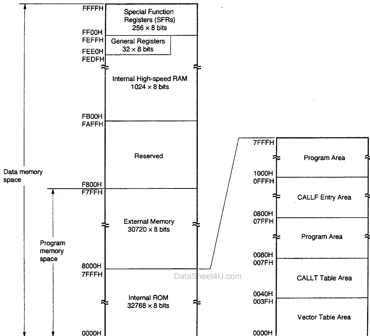
Figure 5-4. Memory Map ( \mu PD780024, 780034, 780024Y, 780034Y)
