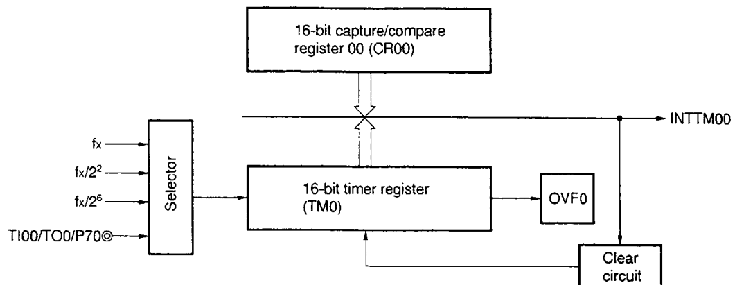
Figure 8-8. Interval Timer Configuration Diagram
