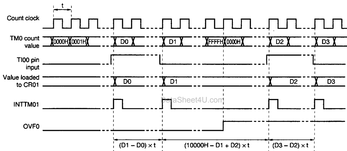
Figure 8-13. Timing of Pulse Width Measurement Operation by Free-Running Counter and One Capture Register (with Both Edges Specified)
