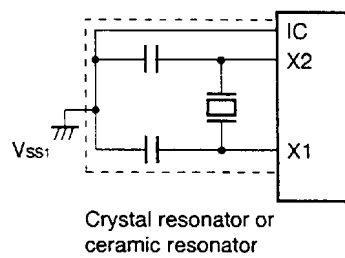
(a) Crystal and ceramic oscillation
