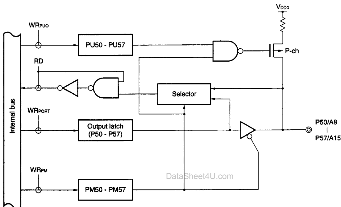
Figure 6-11. P50 to P57 Configurations
