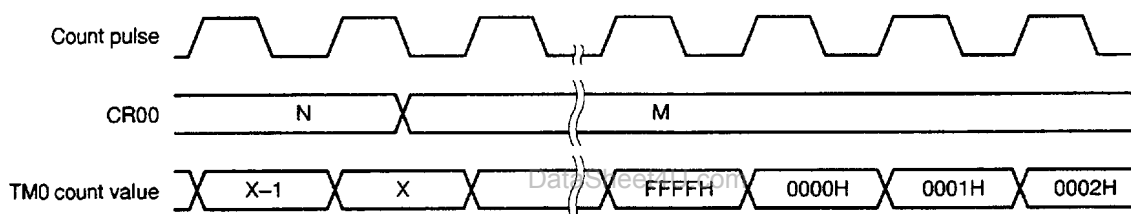
Figure 8-31. Timings After Change of Compare Register During Timer Count Operation
