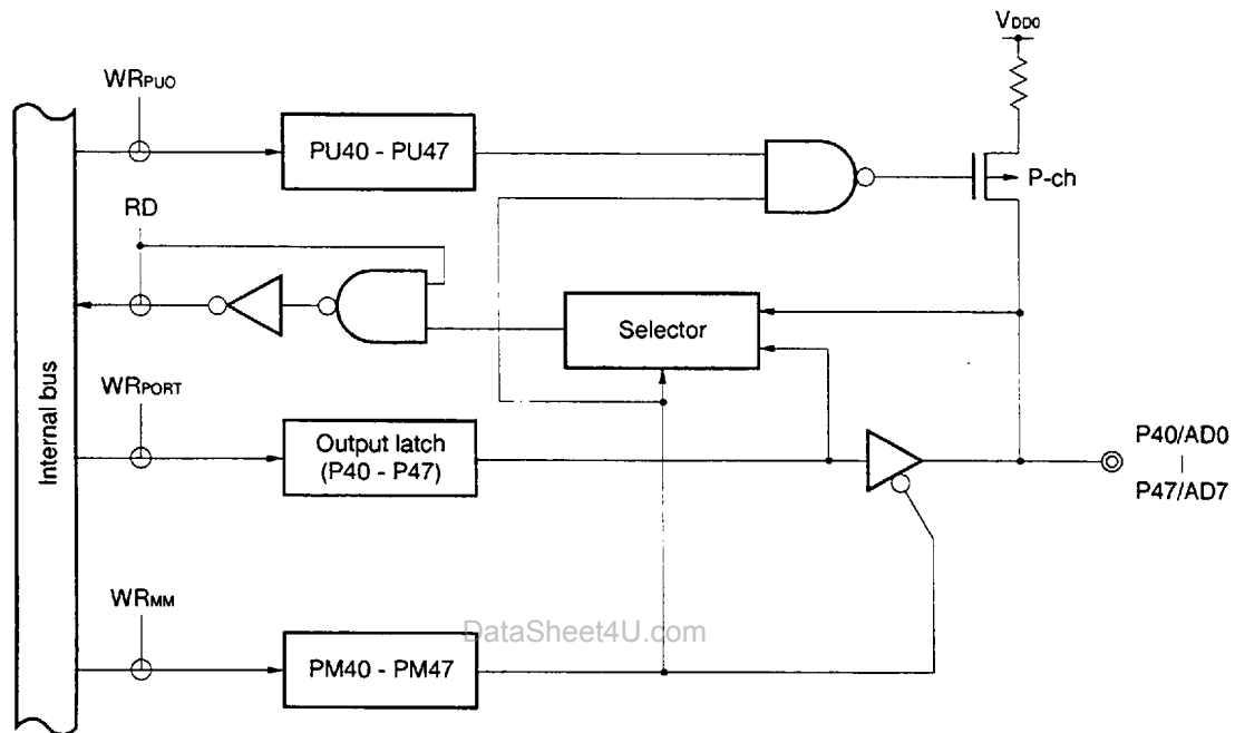
Figure 6-9. P40 to P47 Configurations
