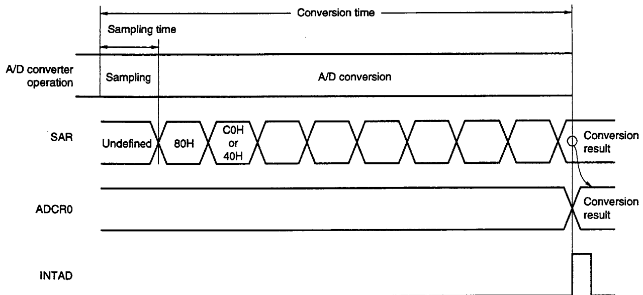
Figure 13-5. Basic Operation of 8-Bit A/D Converter
