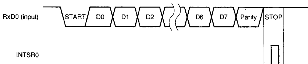
Figure 16-8. Timing of Asynchronous Serial Interface Receive Completion Interrupt
