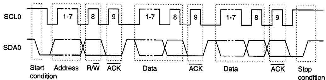
Figure 18-7. I 2 C Bus's Serial Data Transfer Timing
