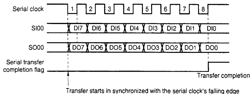
Figure 17-5. Timing of Three-wire Serial I/O Mode
