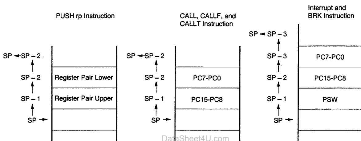
Figure 5-14. Data to be Saved to Stack Memory
