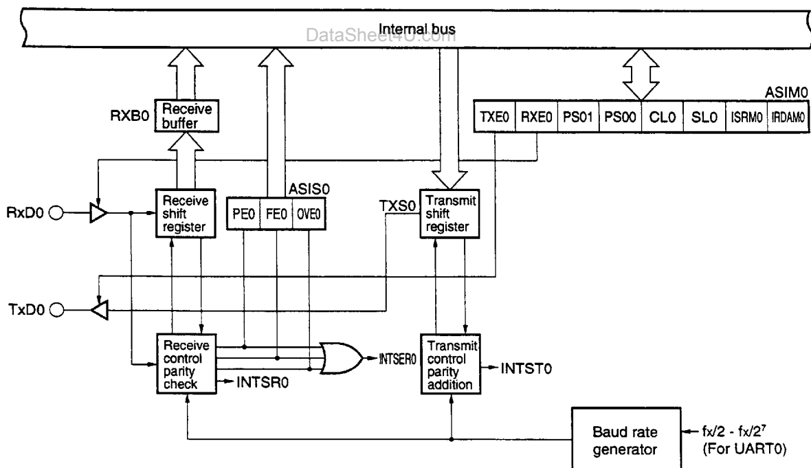
Figure 16-1. Block Diagram of UART0
