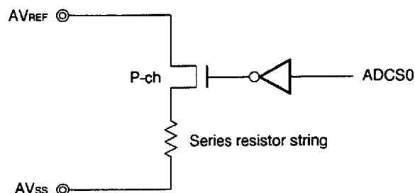
Figure 13-9. Example of Method of Reducing Power Dissipation in Standby Mode
