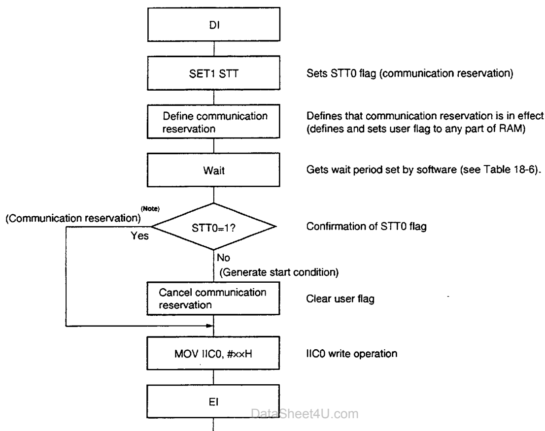
Figure 18-17. Communication Reservation Protocol
