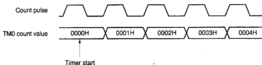
Figure 8-30. 16-Bit Timer Register Start Timing
