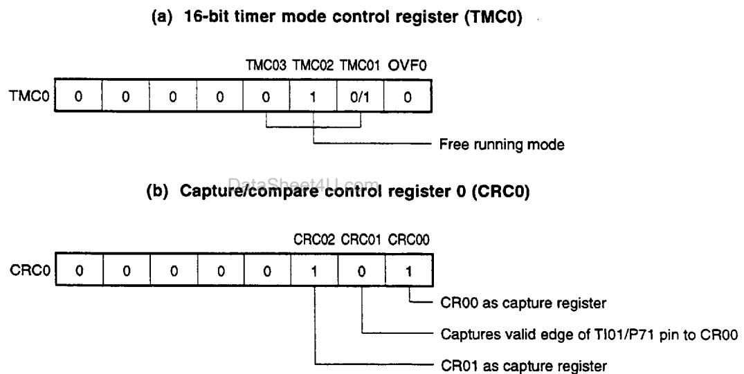
Figure 8-14. Control Register Settings for Measurement of Two Pulse Widths with Free Running Counter
