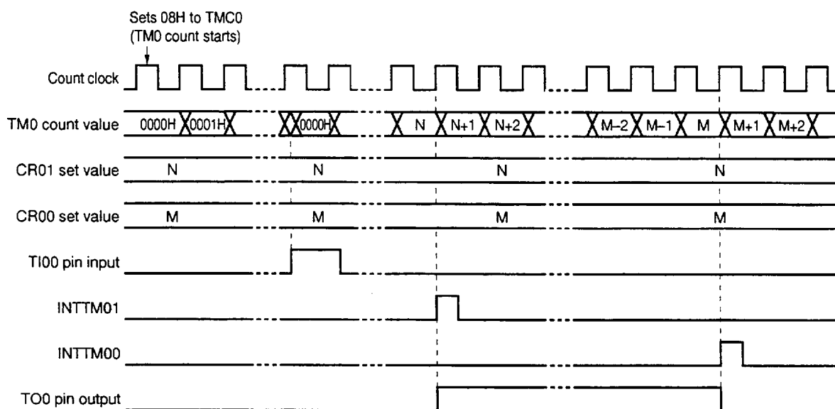
Figure 8-29. Timing of One-Shot Pulse Output Operation Using External Trigger (With Rising Edge Specified)
