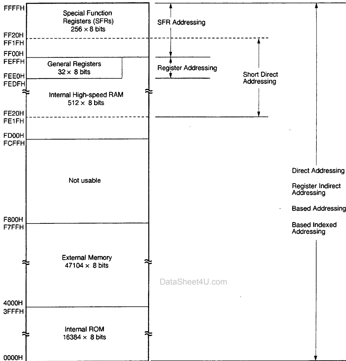
Figure 5-7. Data Memory Addressing ( \mu PD780022, 780032, 780022Y, 780032Y)
