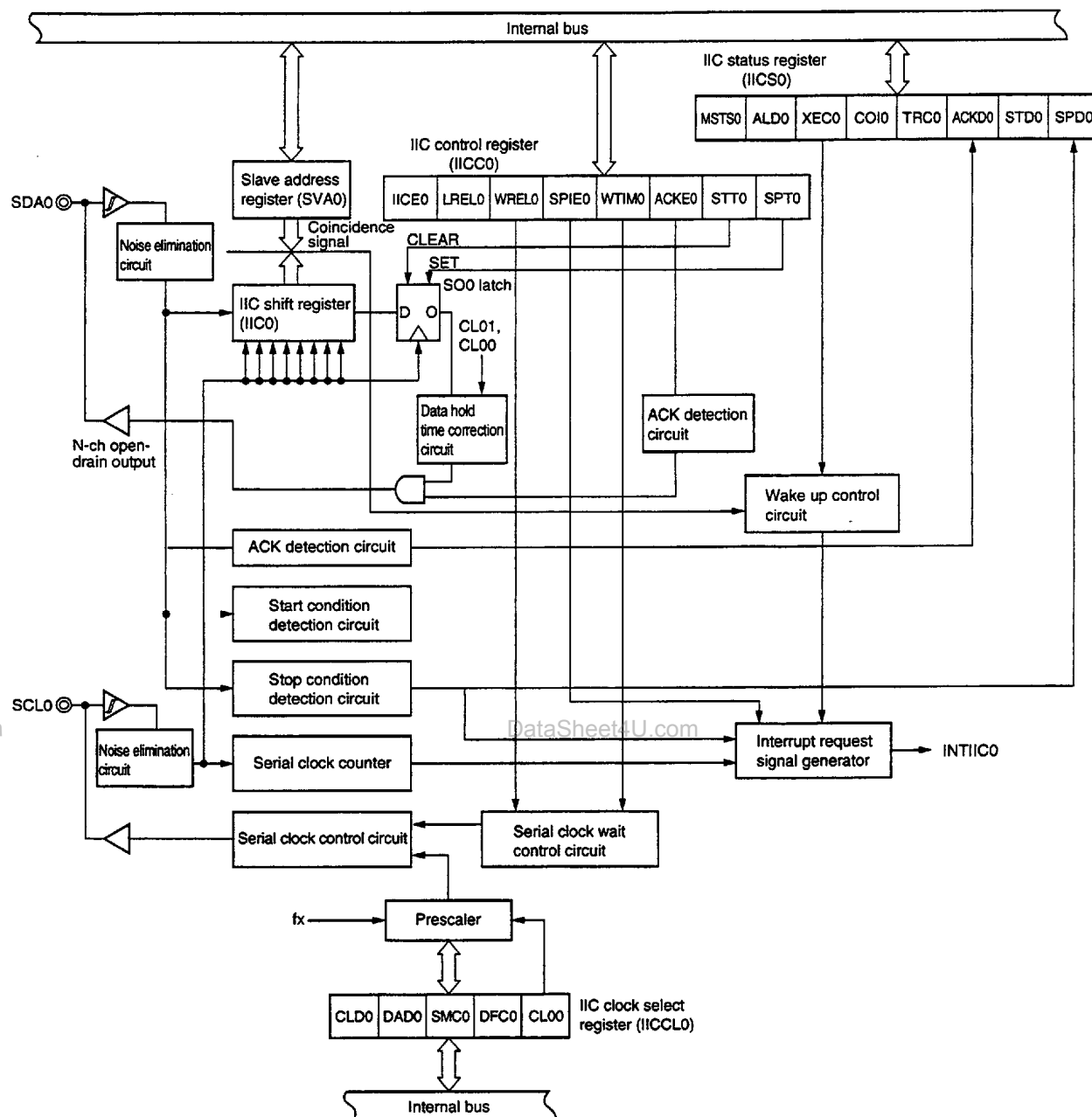
Figure 18-1. Block Diagram of IIC0
