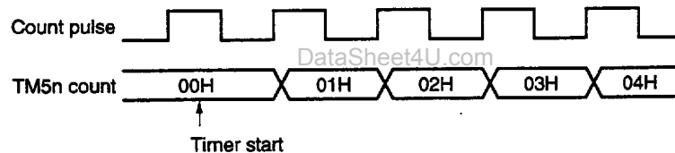
Figure 9-12. Timer 5 Start Timing
