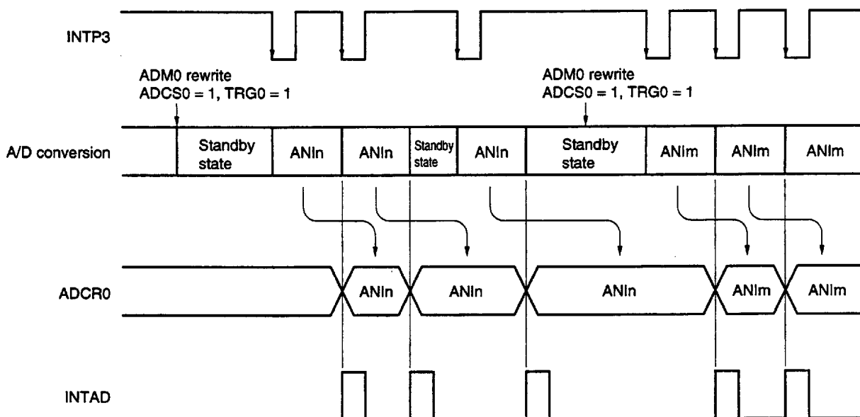
Figure 13-7. A/D Conversion by Hardware Start (When Falling Edge is Specified)
