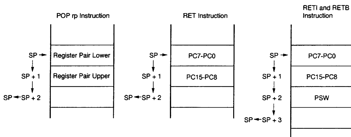
Figure 5-15. Data to be Reset from Stack Memory
