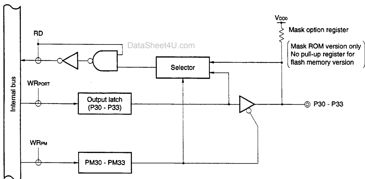
Figure 6-5. P30 to P33 Configurations ( \mu PD780024, 780034 Subseries)
