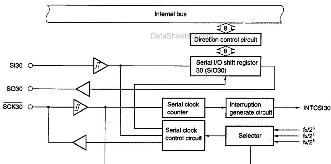
Figure 17-1. Block Diagram of SIO3 Macro
