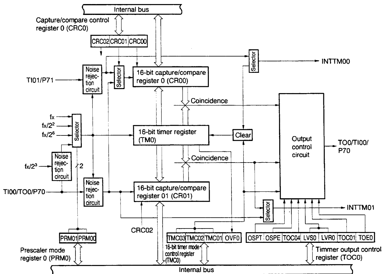
Figure 8-1. Timer 0 (TM0) Block Diagram
