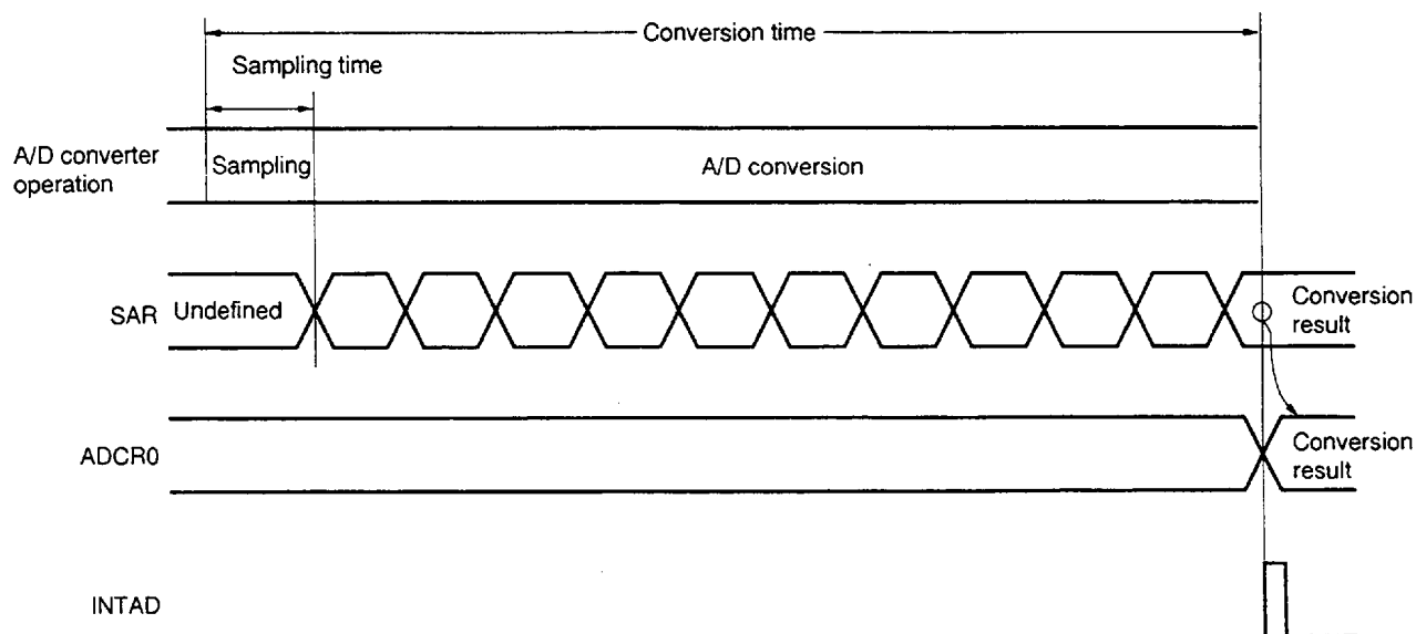
Figure 14-5. Basic Operation of 8-Bit A/D Converter
