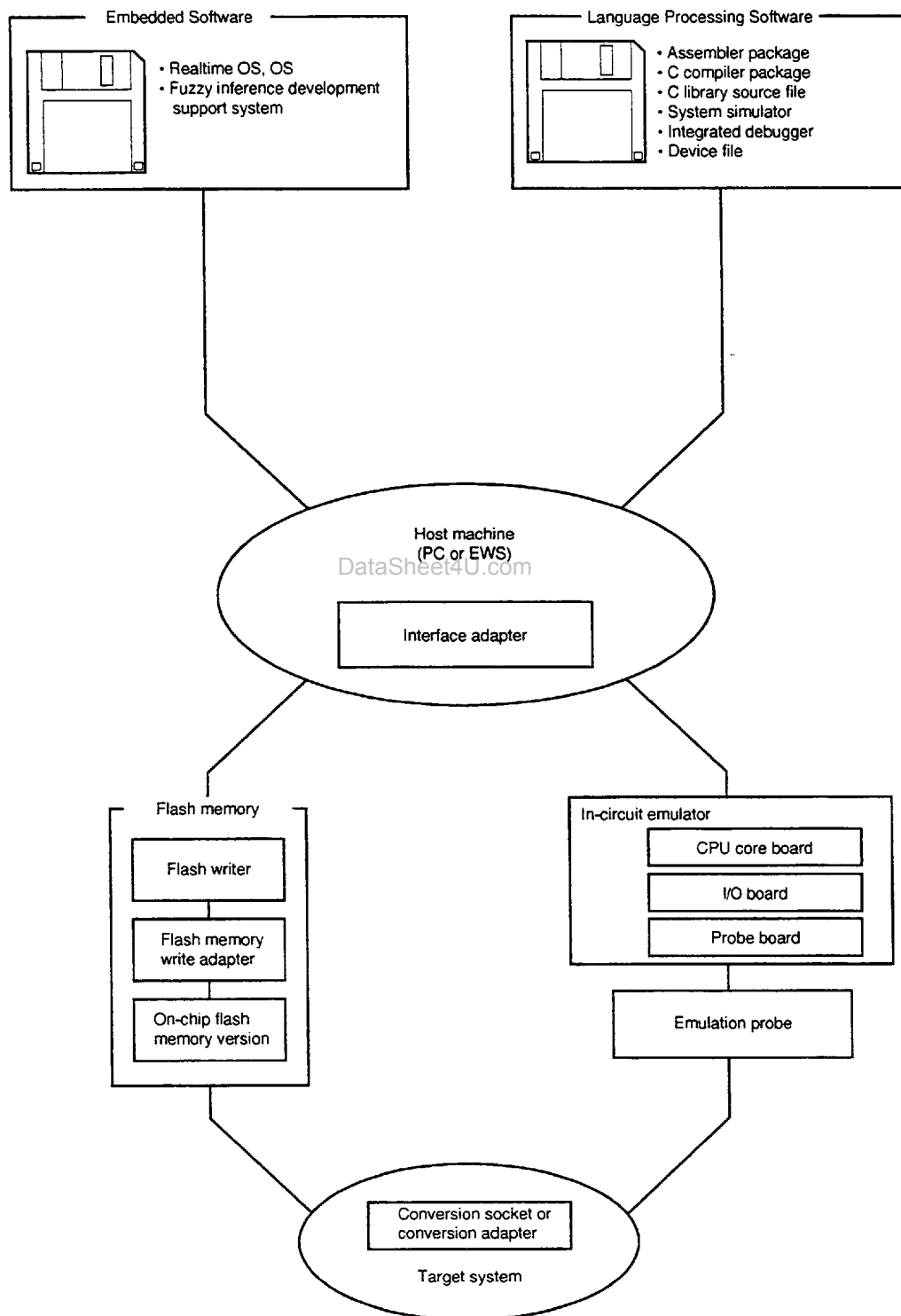
Figure A-1. Development Tool Configuration.
