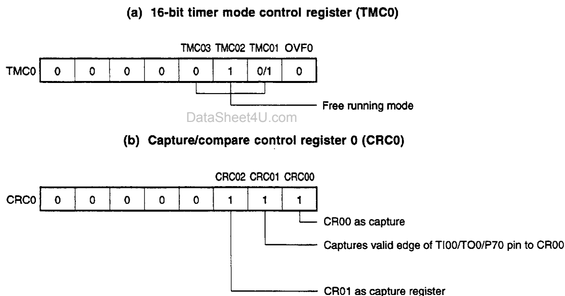
Figure 8-17. Control Register Settings for Pulse Width Measurement with Free-Running Counter and Two Capture Registers
