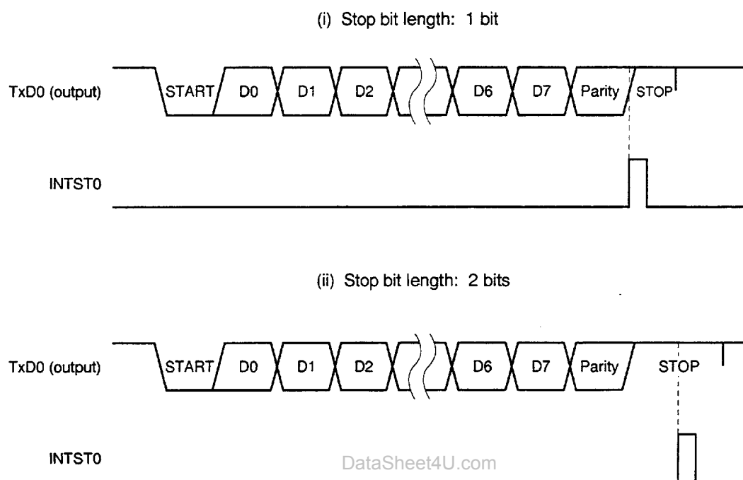
Figure 16-7. Timing of Asynchronous Serial Interface Transmit Completion Interrupt
