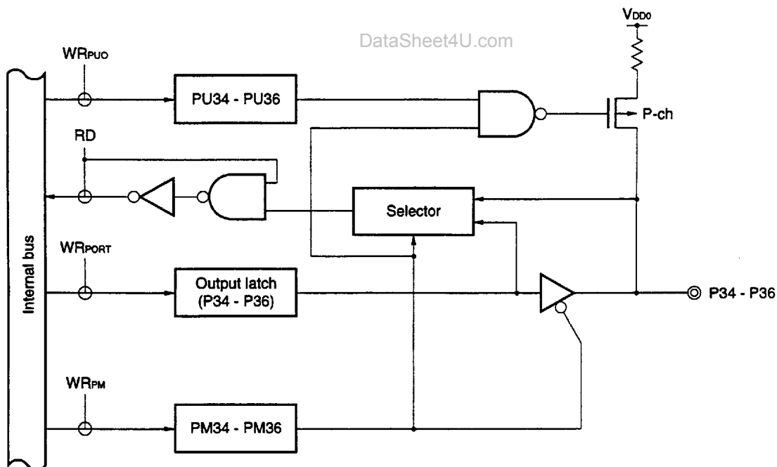
Figure 6-8. P34 to P36 Configurations ( \mu PD780024Y, 780034Y, Subseries)
