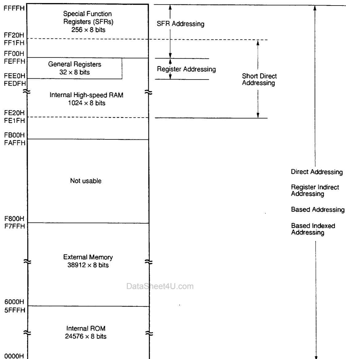
Figure 5-8. Data Memory Addressing ( \mu PD780023, 780033, 780023Y, 780033Y)
