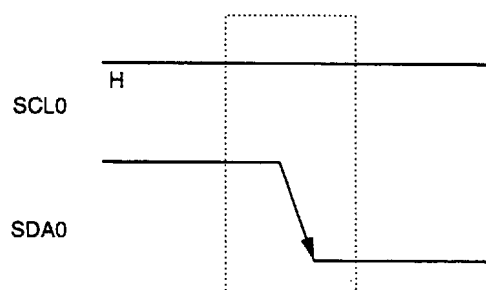
Figure 18-8. Start Conditions
