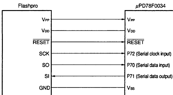
Figure 23-6. Flashpro Connection Using Pseudo 3-wire Serial I/O
