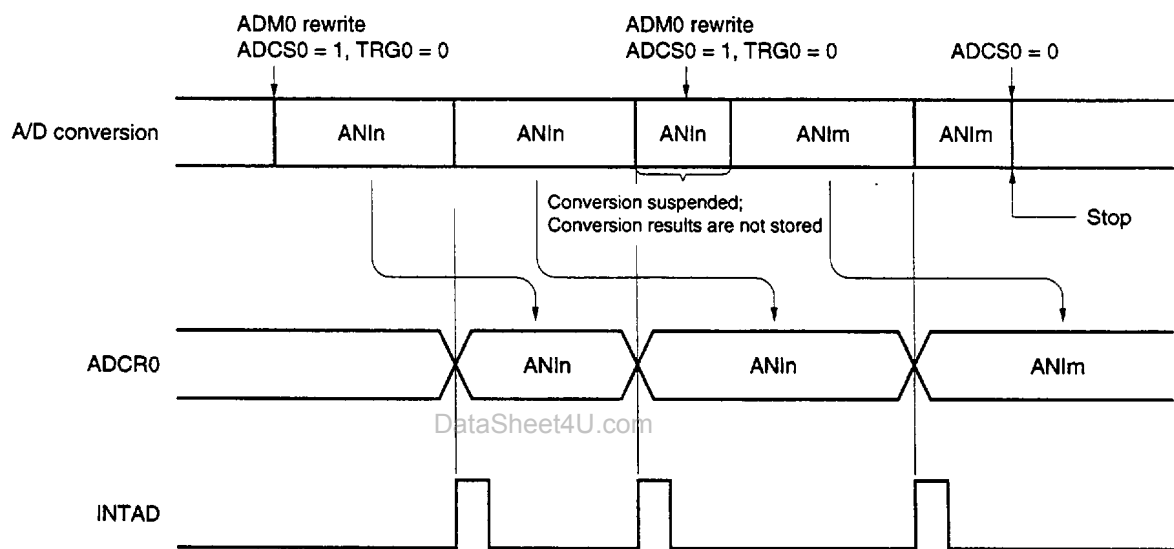
Figure 13-8. A/D Conversion by Software Start
