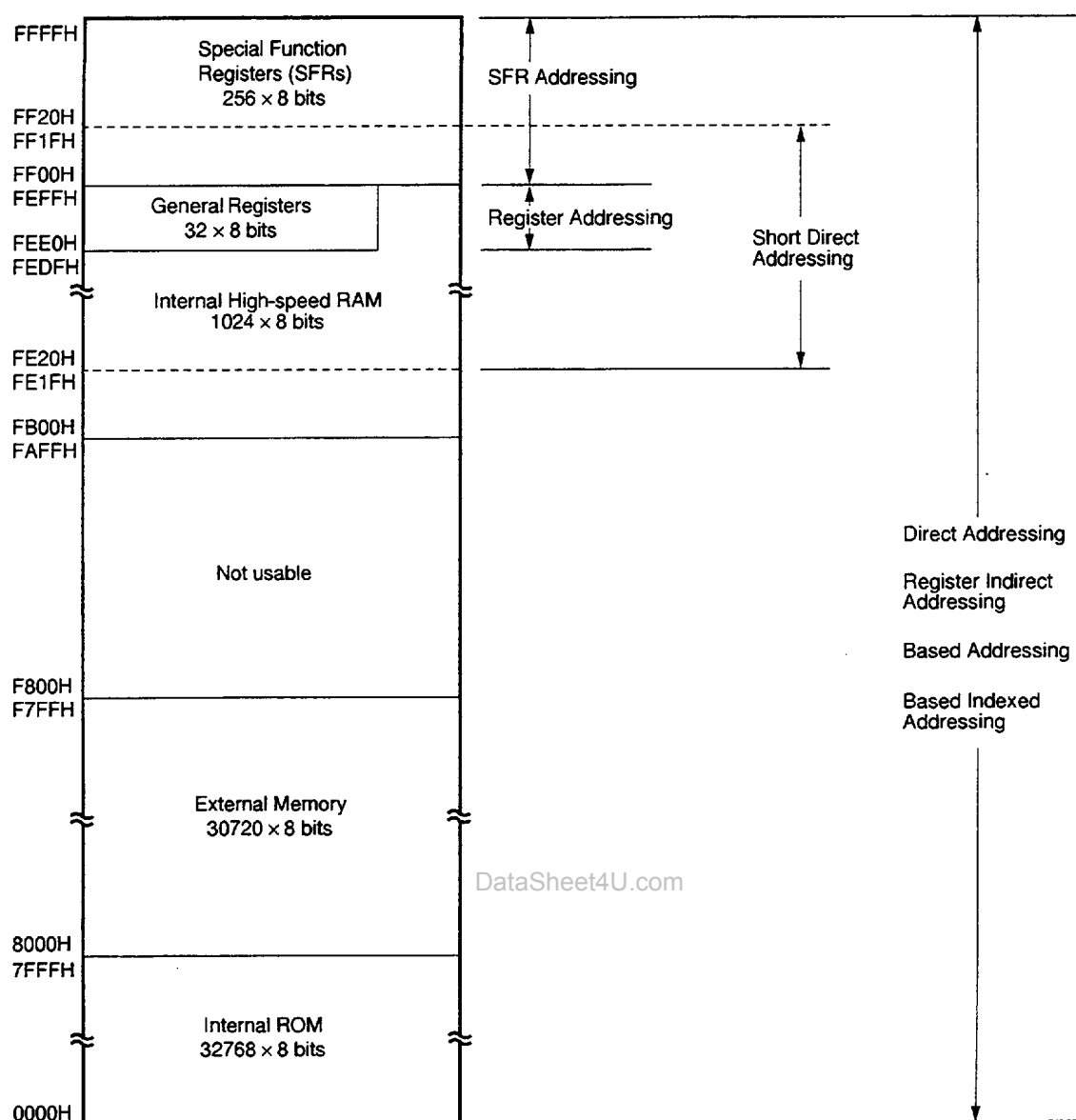
Figure 5-9. Data Memory Addressing ( \mu PD780024, 780034, 780024Y, 780034Y)
