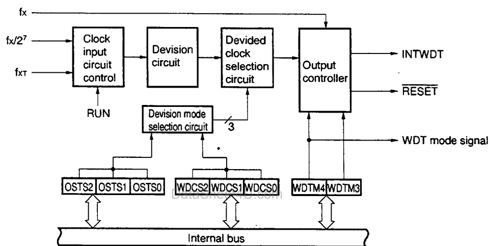
Figure 11-1. Block Diagram of Watchdog Timer
