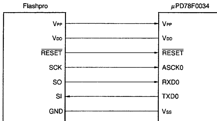
Figure 23-5. Flashpro Connection Using I 2 C Bus Method
