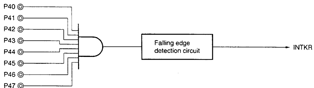
Figure 6-10. Block Diagram of Falling Edge Detection Circuit
