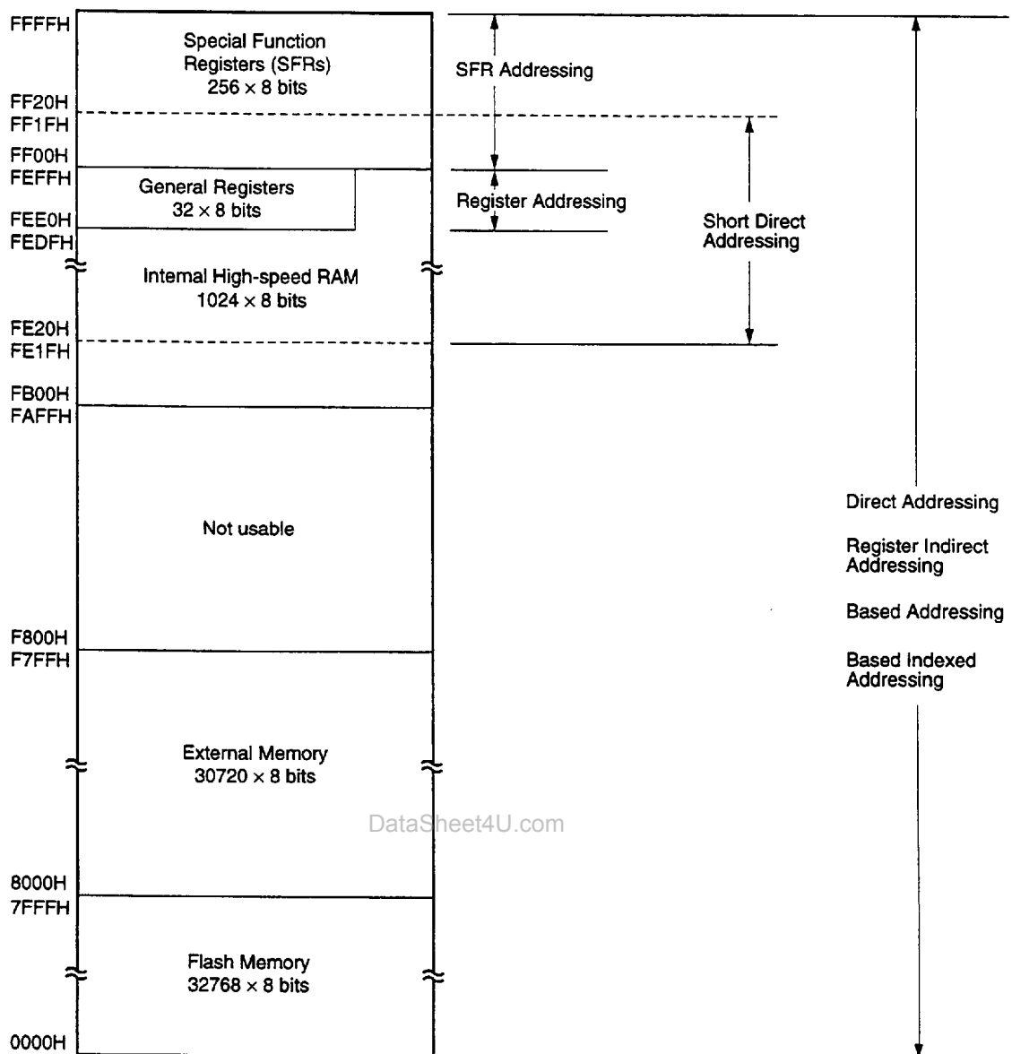
Figure 5-10. Data Memory Addressing ( \mu PD78F0034, 78F0034Y)
