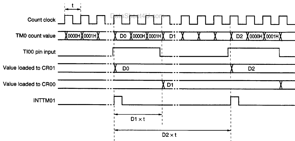
Figure 8-20. Timing of Pulse Width Measurement Operation by Means of Restart (with Rising Edge Specified)
