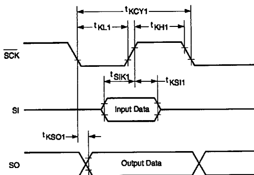
Figure 23. Serial Transfer Timing
