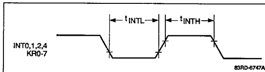
Figure 21. Interrupt Input Timing
