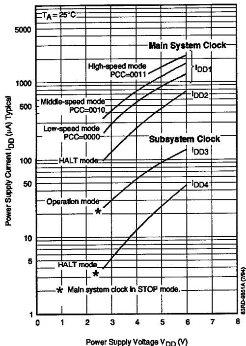
I_{DD} vs V_{DD} (Ceramic Oscillator at 2.00 MHz) μPD7500x
