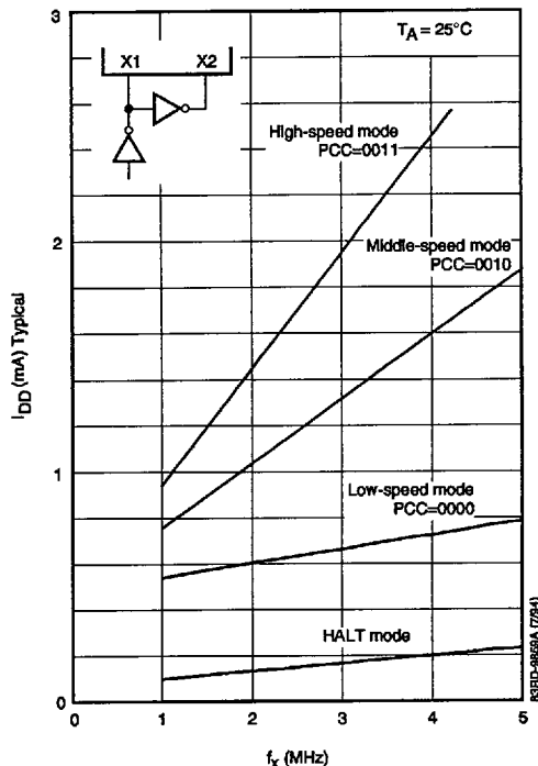
I_{DD} vs f_X ( V_{DD} = 5 V) μPD7500x
