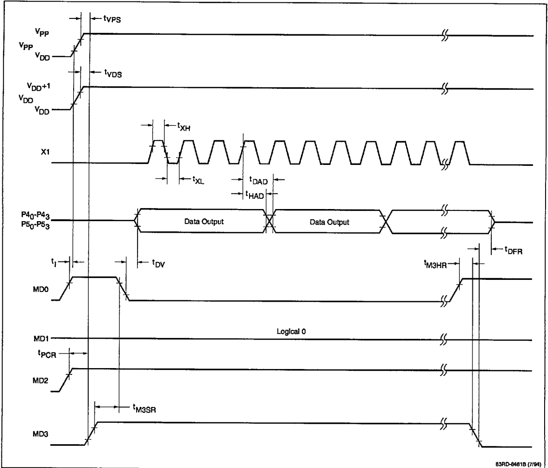
Figure 28. Program Memory Read Timing ( \mu PD75P008)
