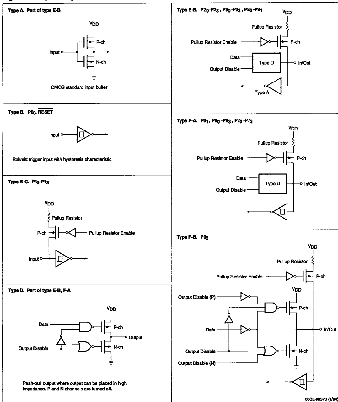
Figure 5. Input/Output Circuits
