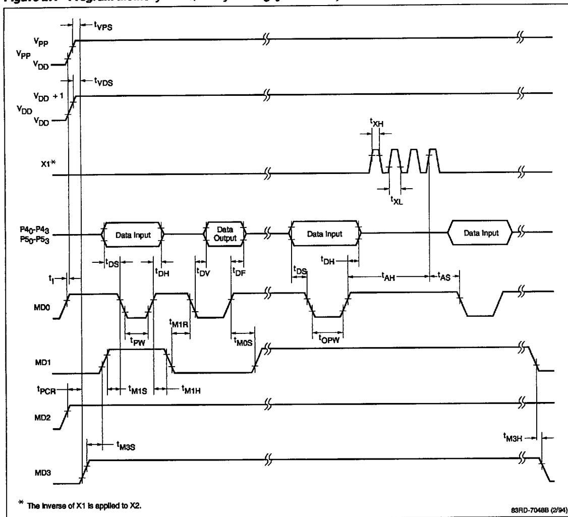
Figure 27. Program Memory Write/Verify Timing (μPD75P008)
