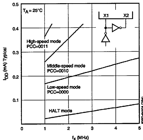
I_{DD} vs f_X ( V_{DD} = 3 V) μPD7500x
