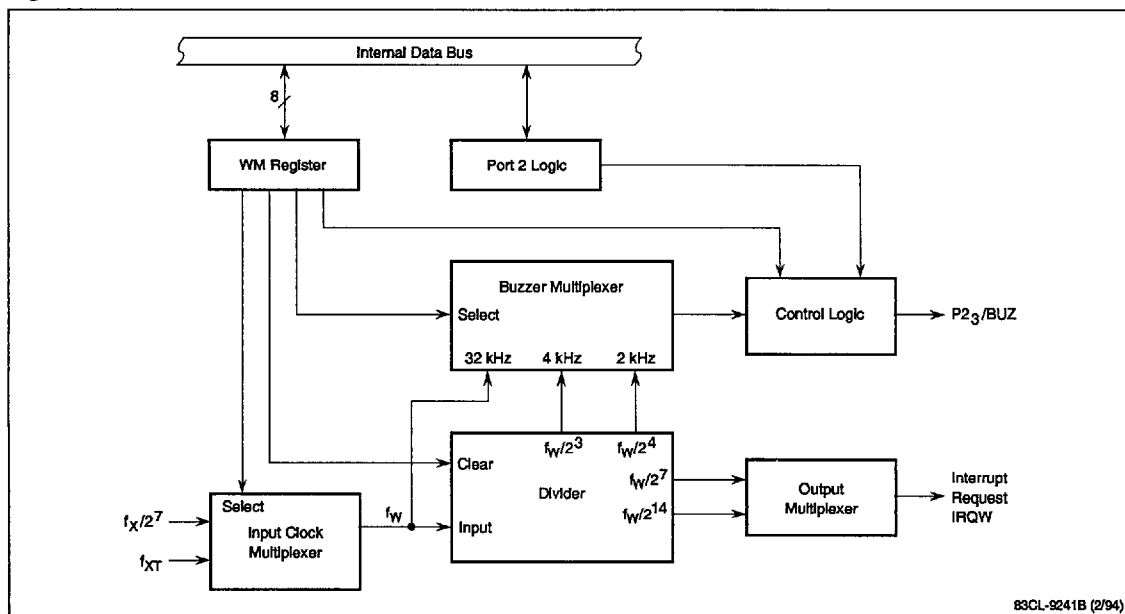
Figure 9. Watch/Timer
