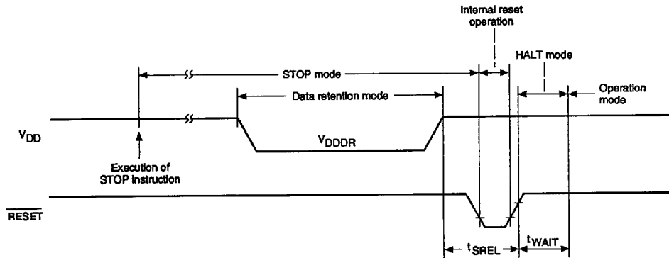
Figure 24. Data Retention Timing
