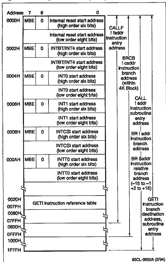
Figure 1. Program Memory Map
