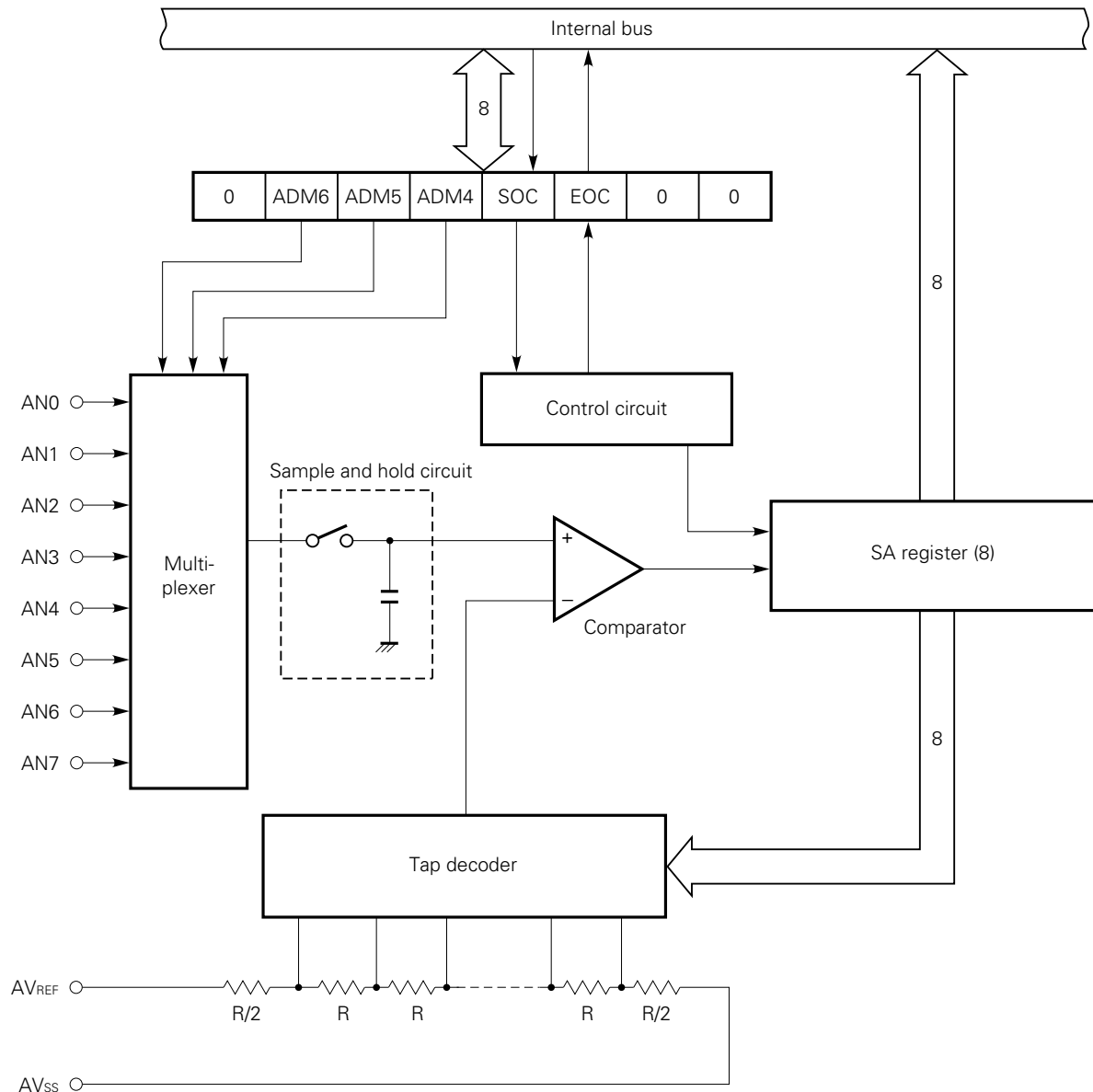
Fig. 4-62 Block Diagram of the A/D Converter
