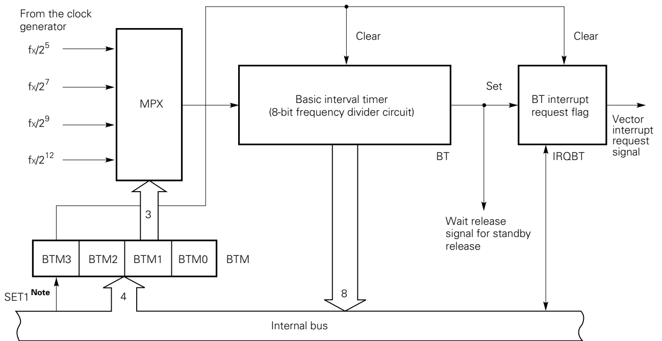
Fig. 4-23 Configuration of the Basic Interval Timer
