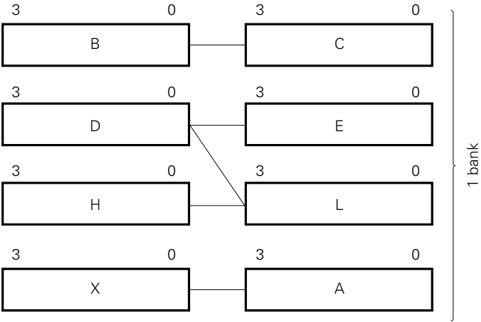
Fig. 3-6 Register Pair Format
