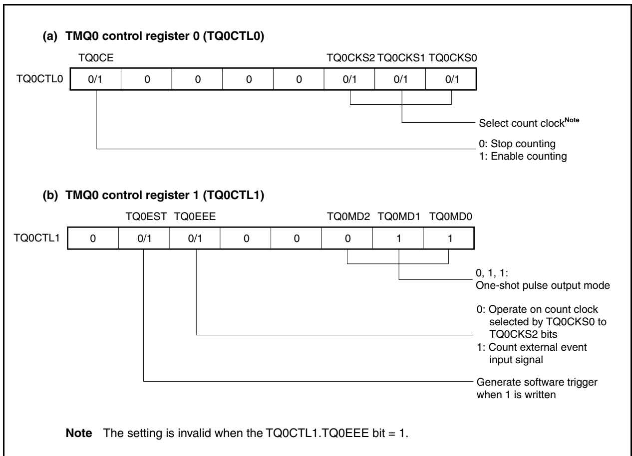
Figure 8-22. Setting of Registers in One-Shot Pulse Output Mode (1/3)
