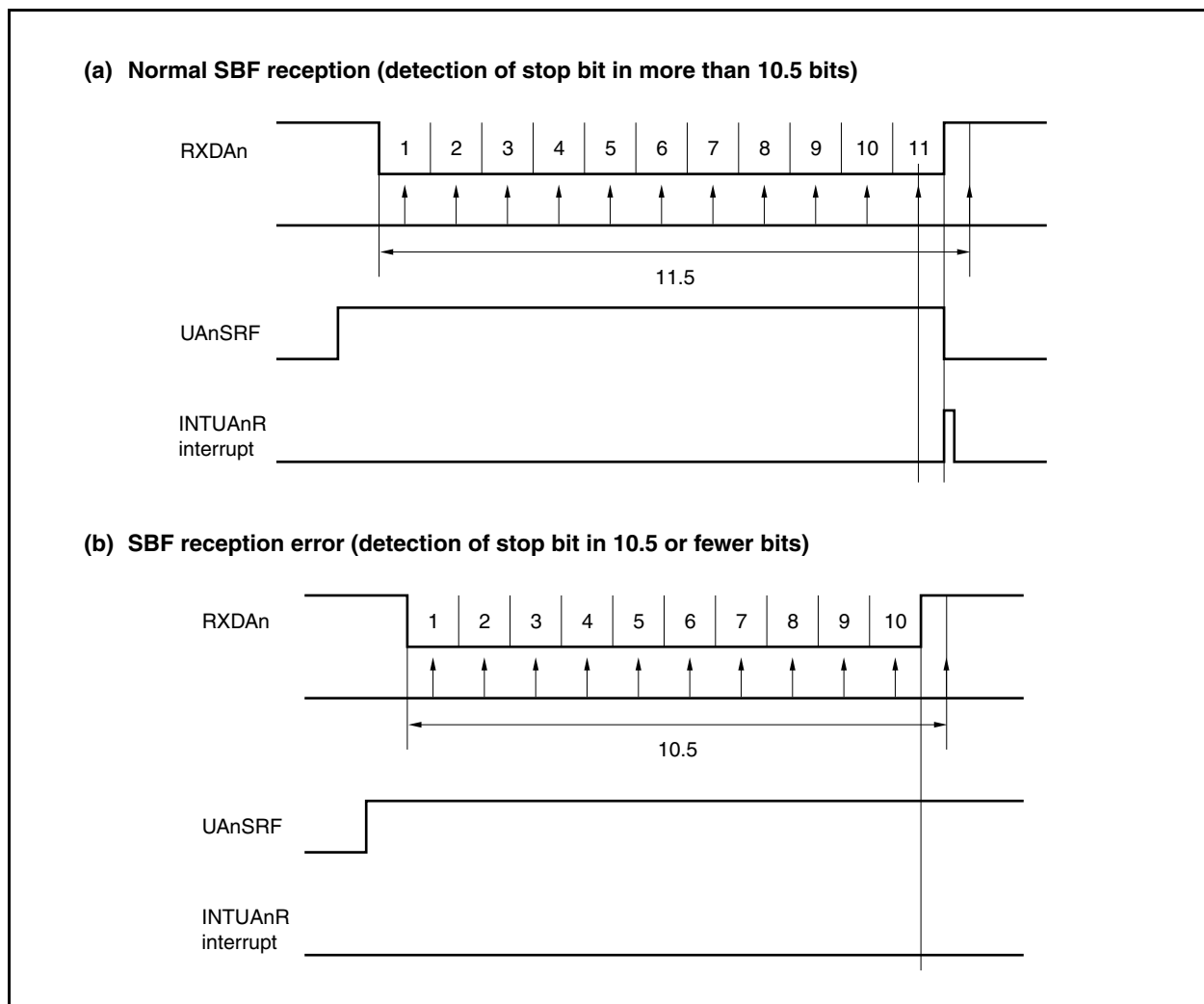
Figure 15-9. SBF Reception
