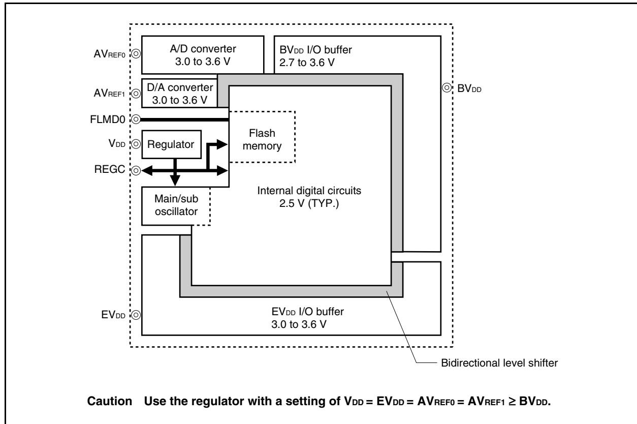
Figure 25-1. Regulator
