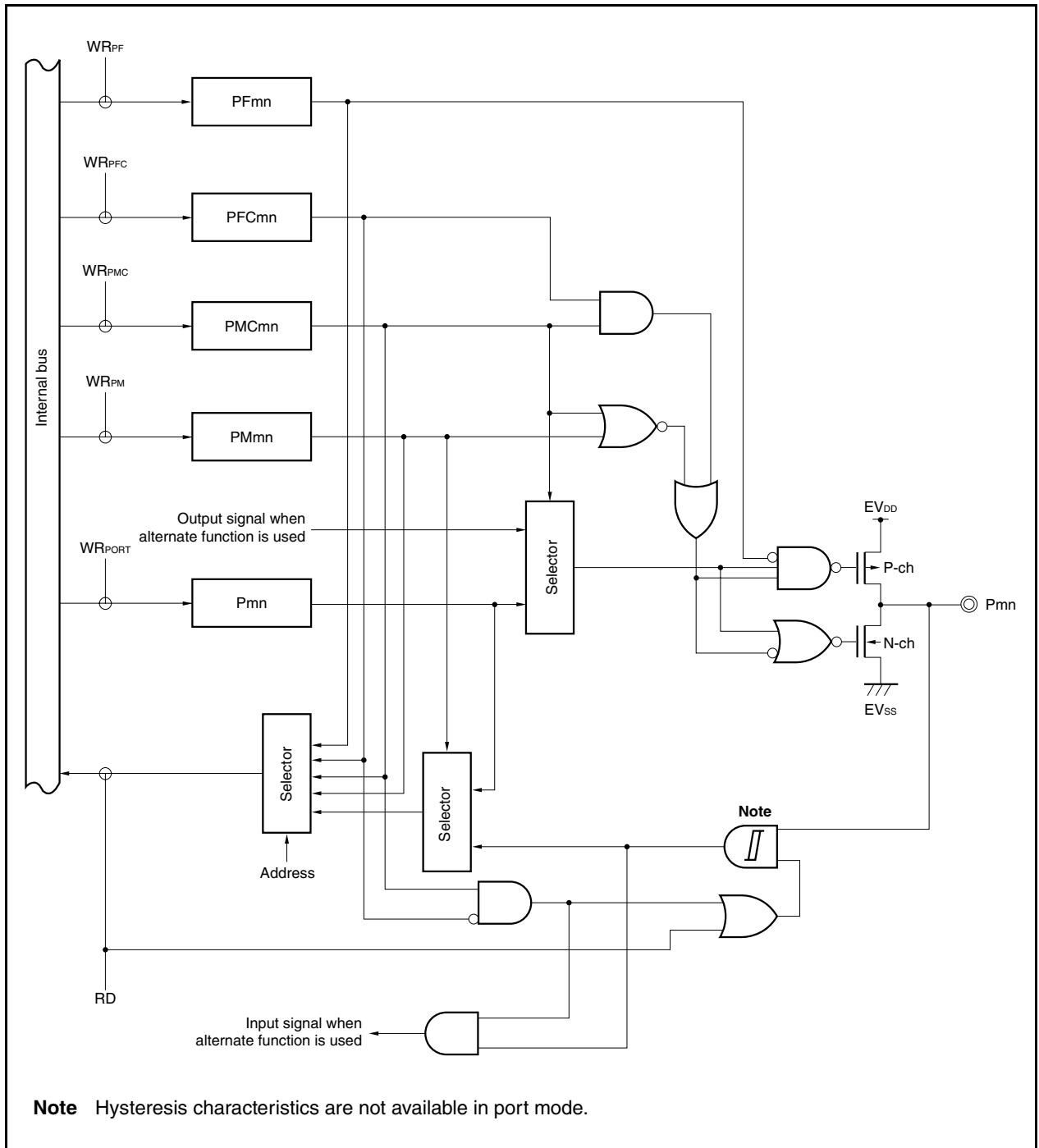
Figure 4-10. Block Diagram of Type G-1
