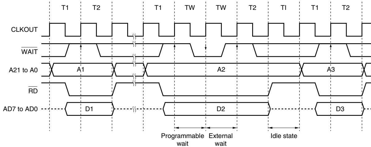
Figure 5-10. Separate Bus Read Timing (Bus Size: 8 Bits)
