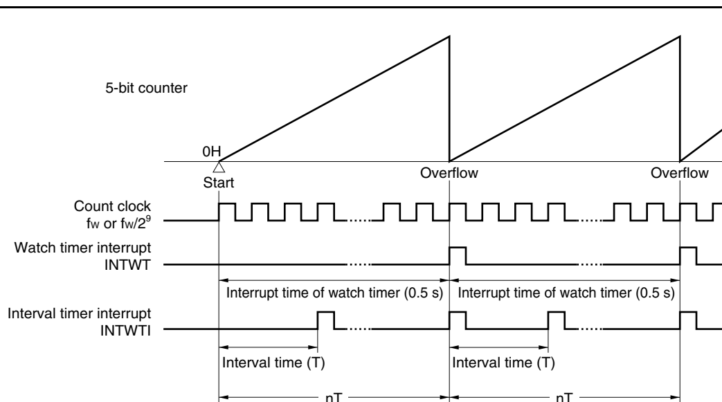
Figure 10-2. Operation Timing of Watch Timer/Interval Timer
