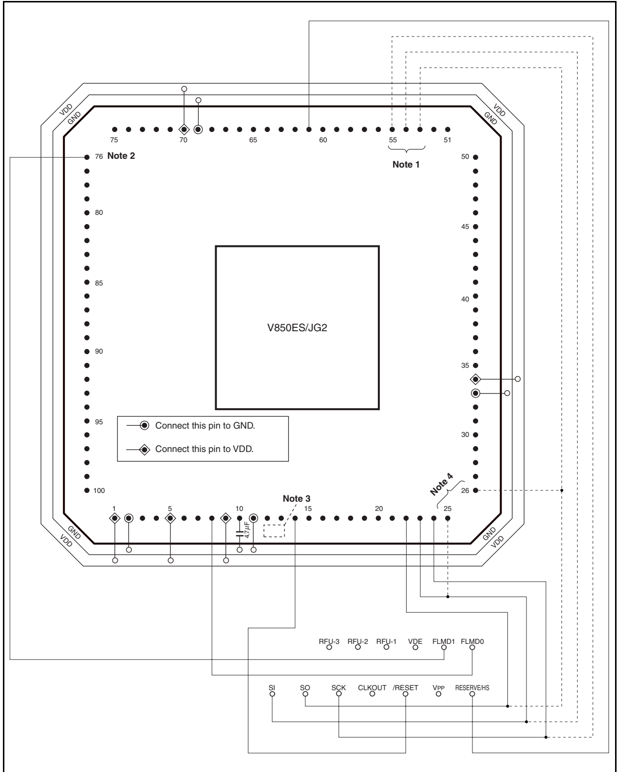
Figure 26-7. Wiring Example of V850ES/JG2 Flash Writing Adapter (FA-100GC-8EA) (In CSIB0 + HS Mode) (1/2)
