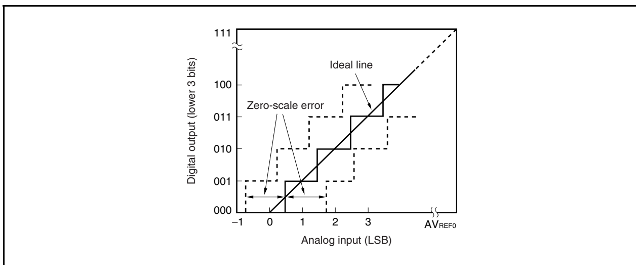
Figure 13-18. Zero-Scale Error
