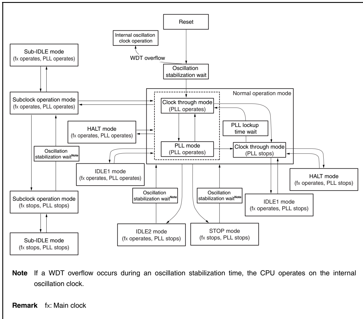
Figure 21-1. Status Transition
