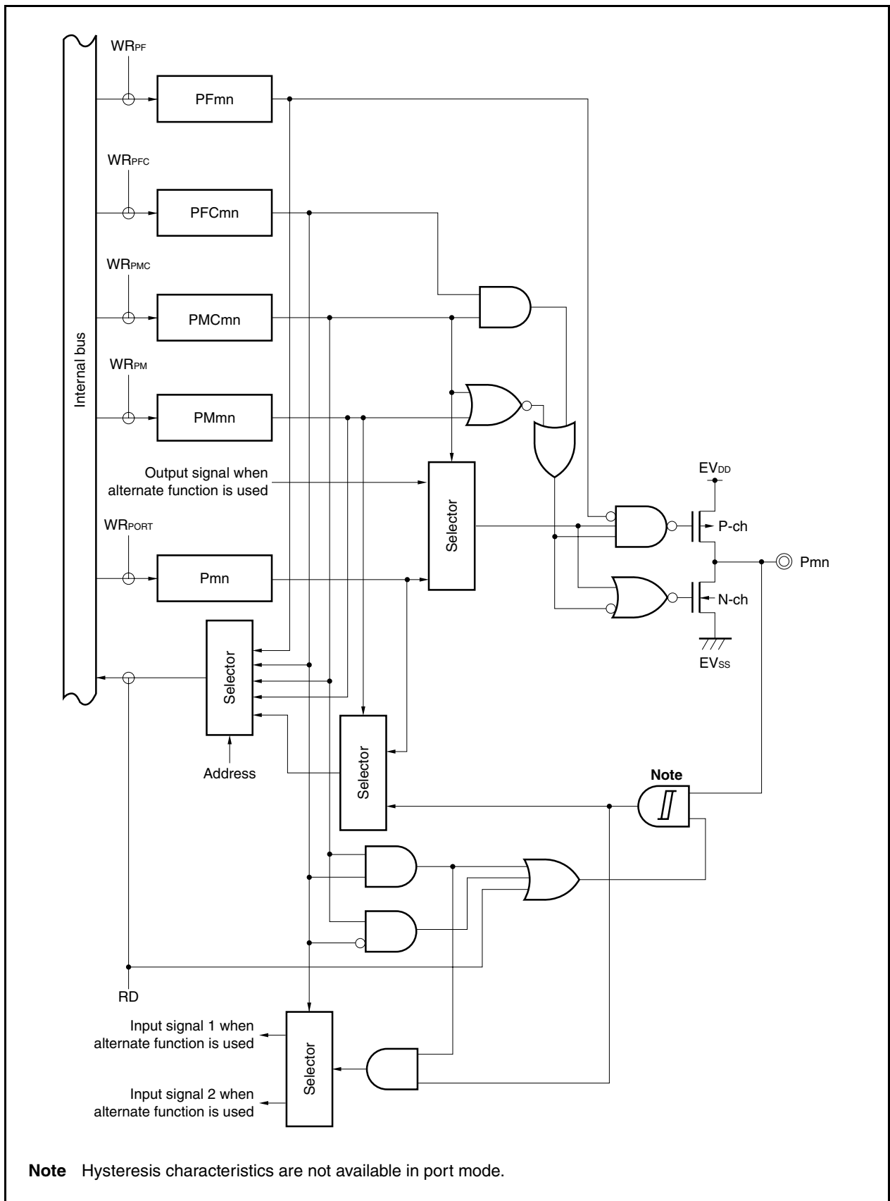
Figure 4-14. Block Diagram of Type G-6
