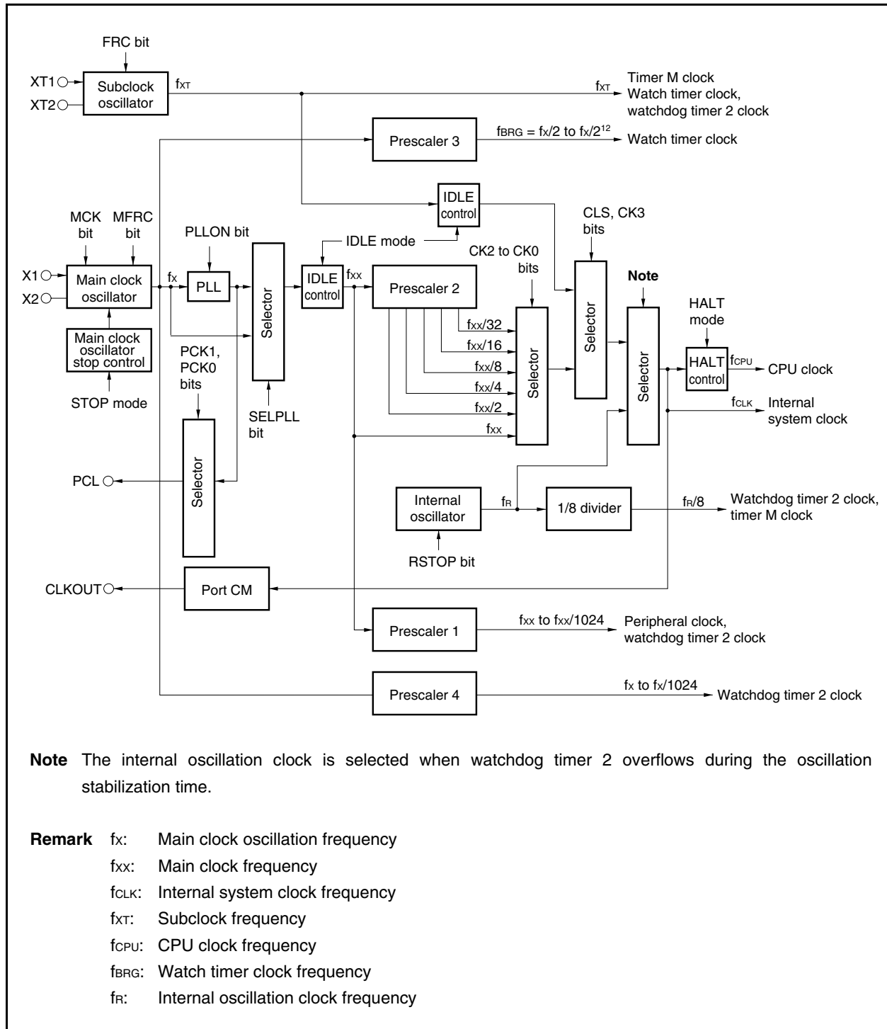
Figure 5-1. Clock Generator
