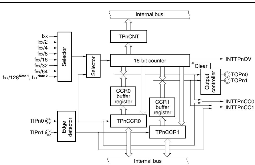
Figure 6-1. Block Diagram of TMPn
