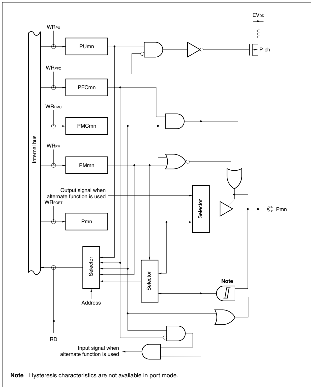
Figure 4-8. Block Diagram of Type G-1
