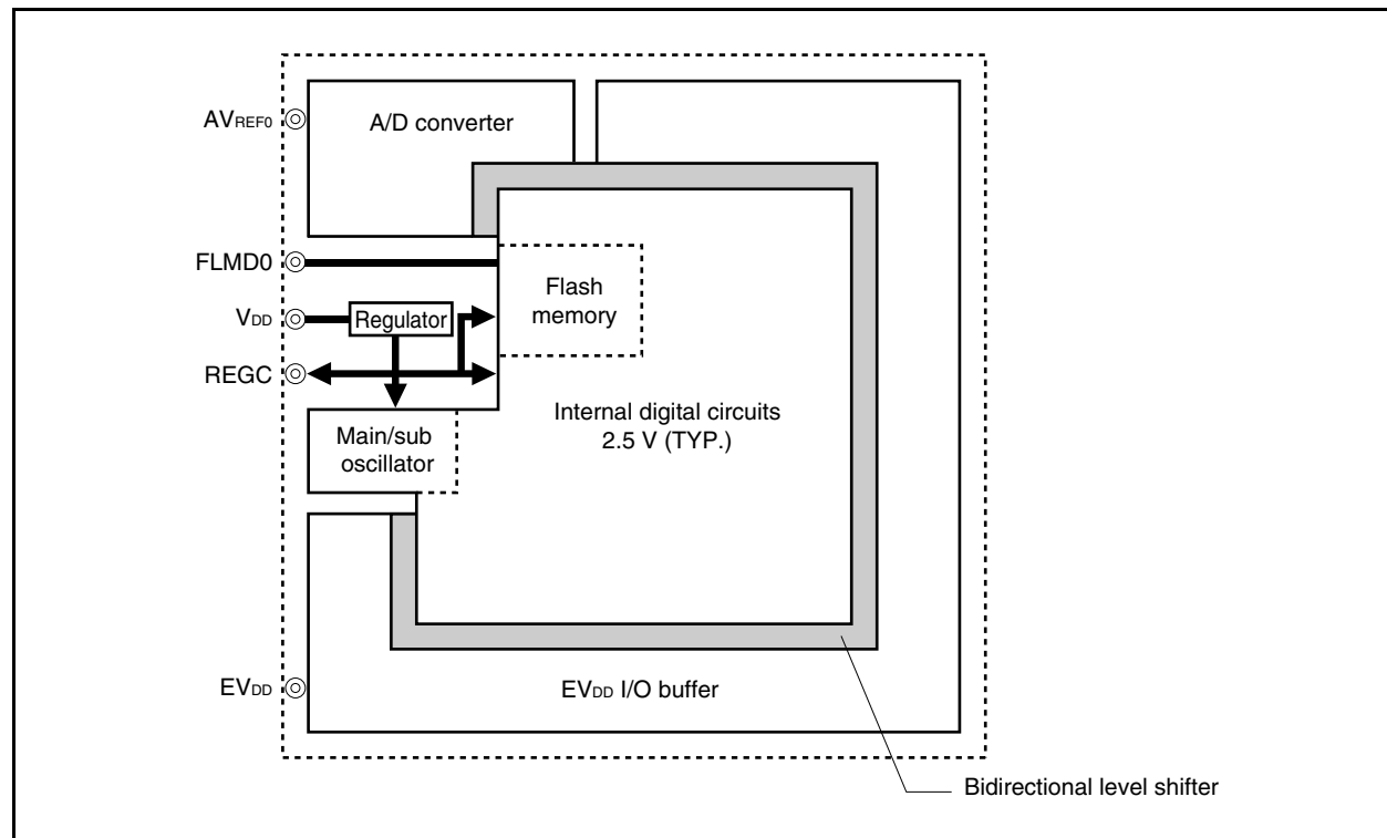
Figure 21-1. Regulator
