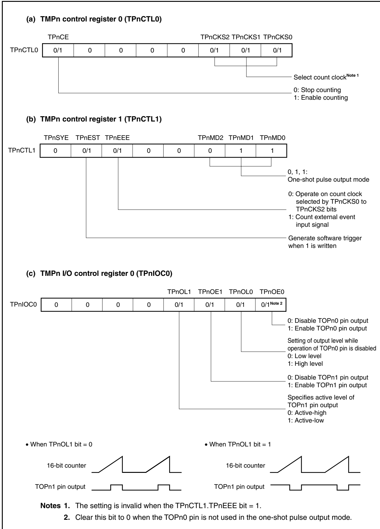
Figure 6-22. Setting of Registers in One-Shot Pulse Output Mode (1/2)
