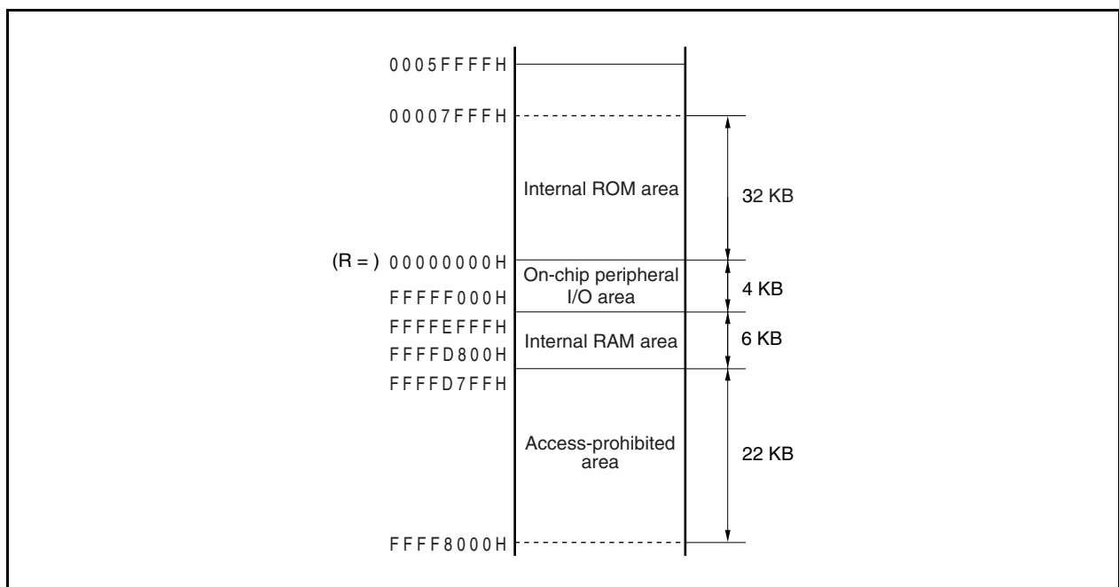
Figure 3-8. Wraparound
