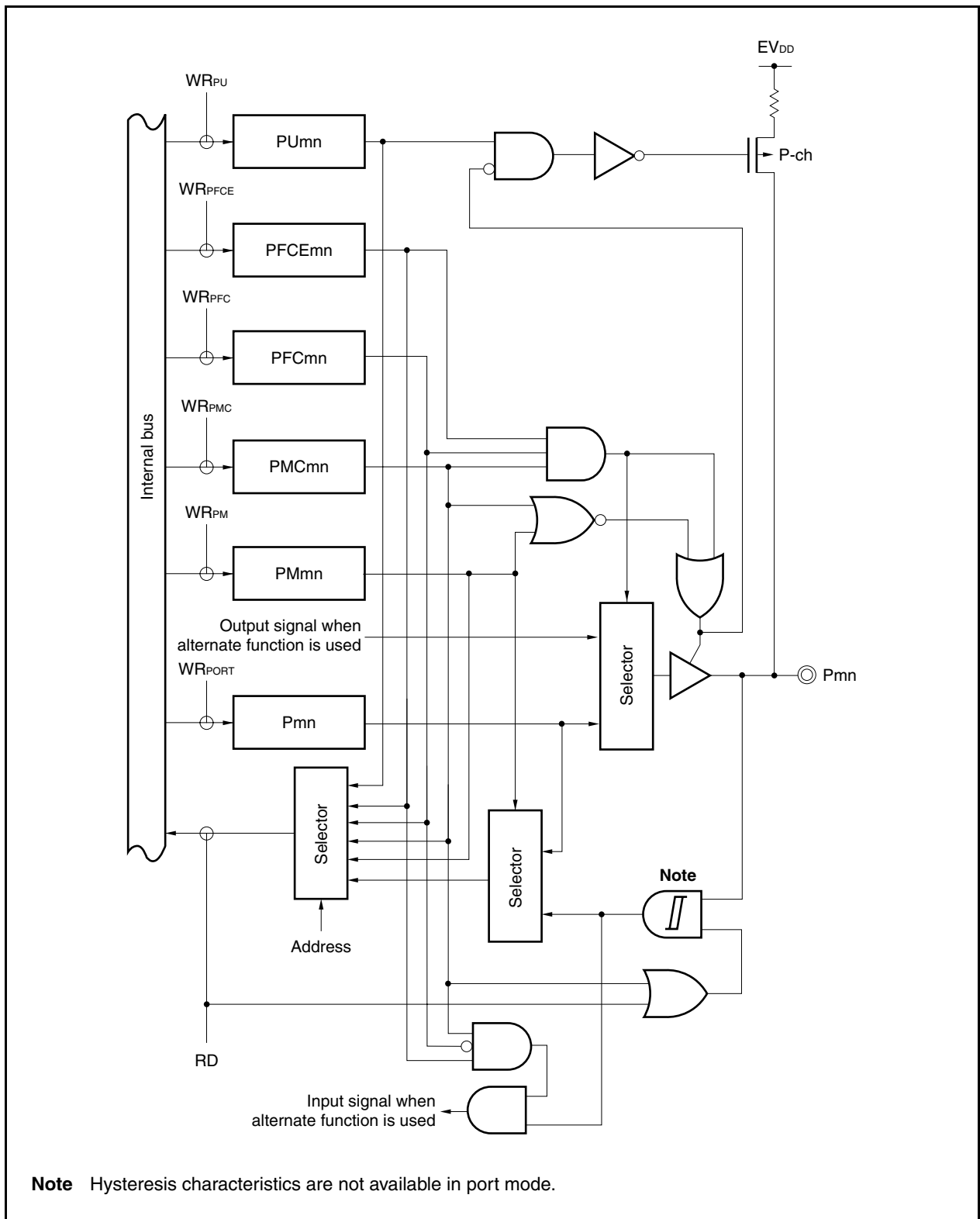
Figure 4-21. Block Diagram of Type U-9
