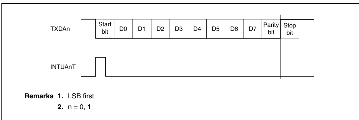
Figure 12-7. UART Transmission
