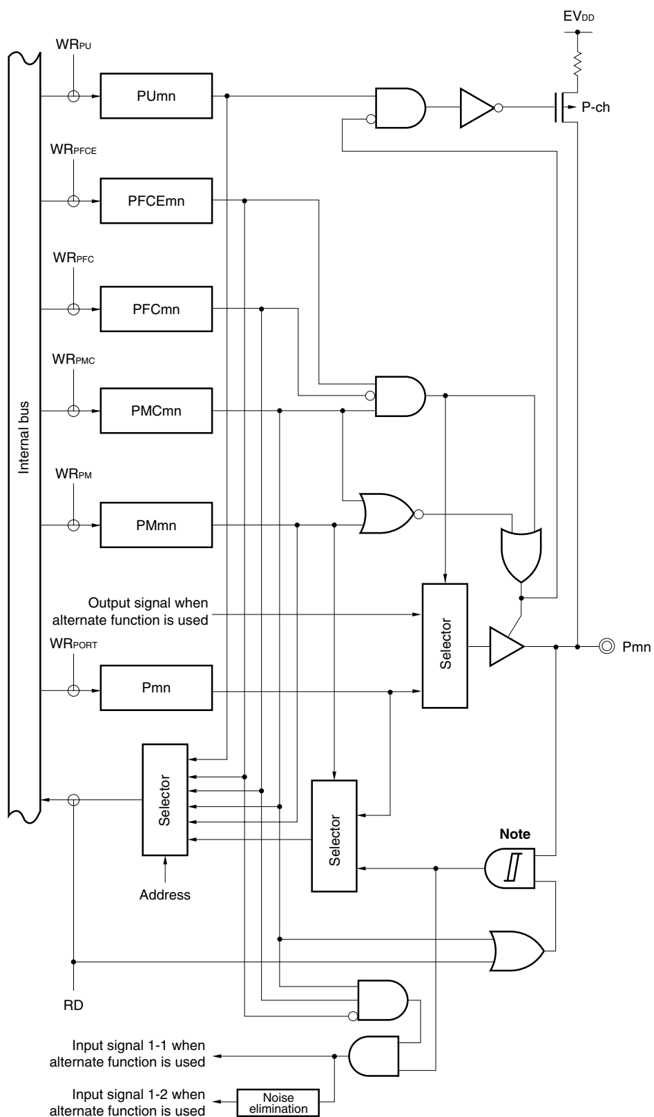
Figure 4-16. Block Diagram of Type U-4
