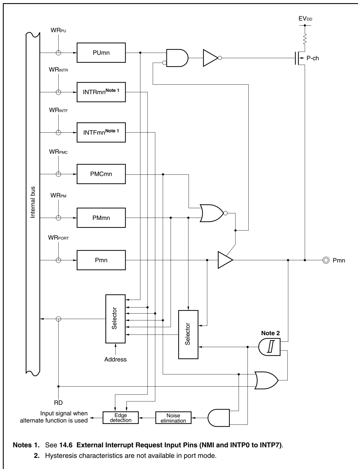
Figure 4-12. Block Diagram of Type L-1
