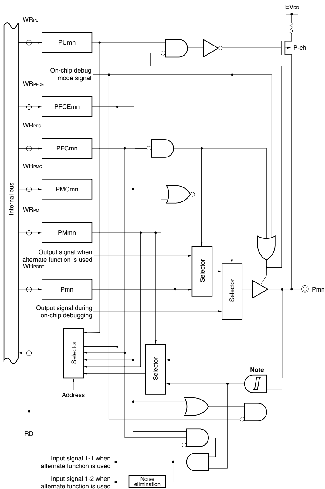
Figure 4-18. Block Diagram of Type U-6
