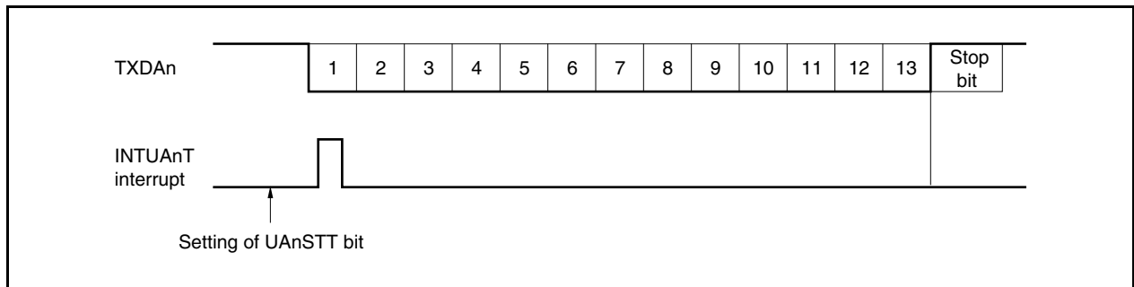
Figure 12-5. SBF Transmission
