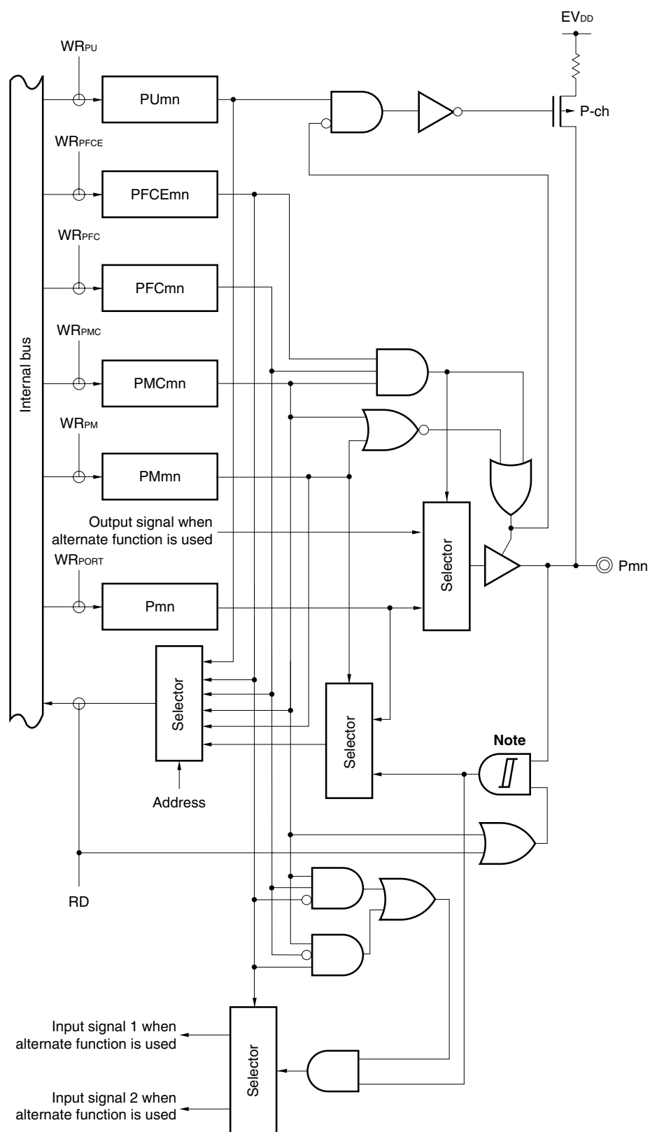
Figure 4-20. Block Diagram of Type U-8
