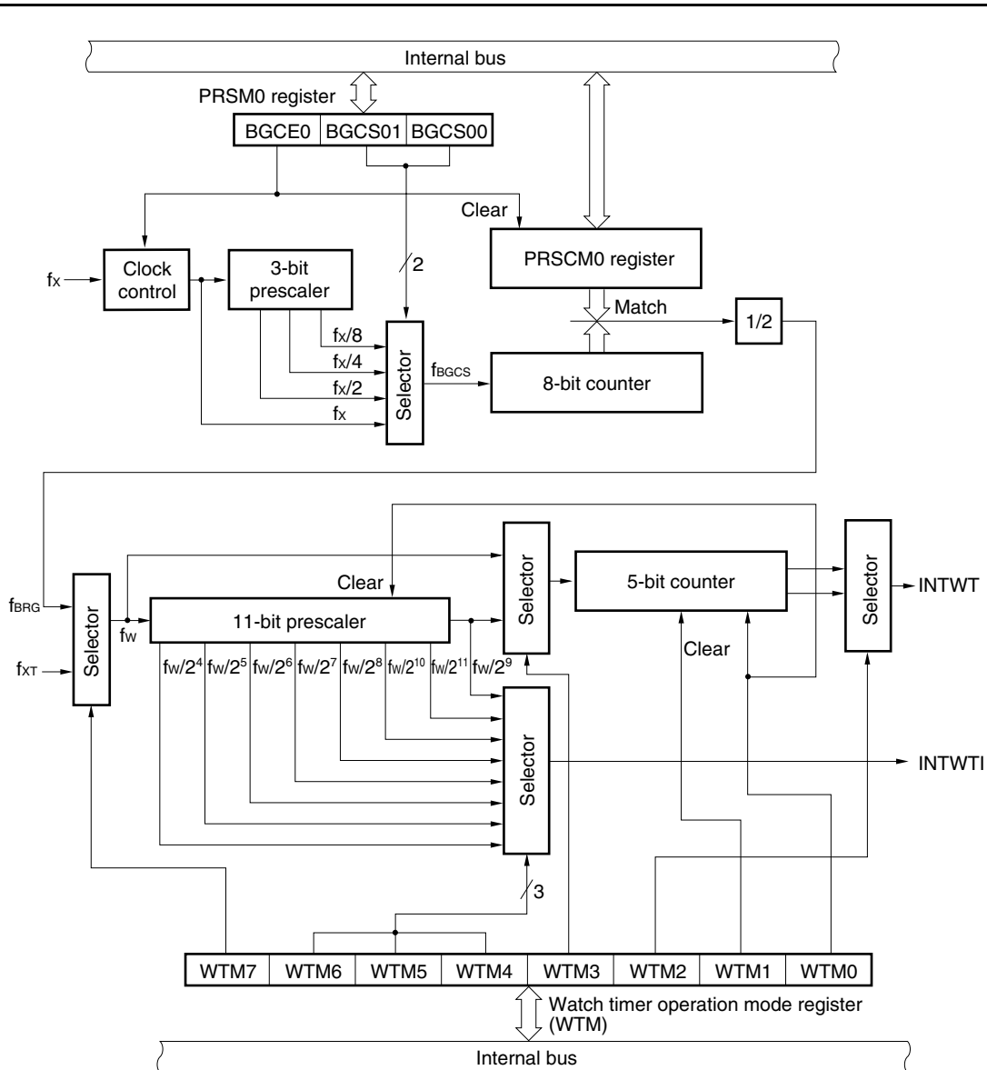
Figure 9-1. Block Diagram of Watch Timer
