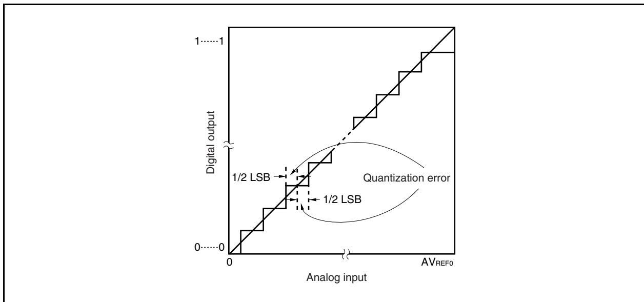
Figure 11-14. Quantization Error
