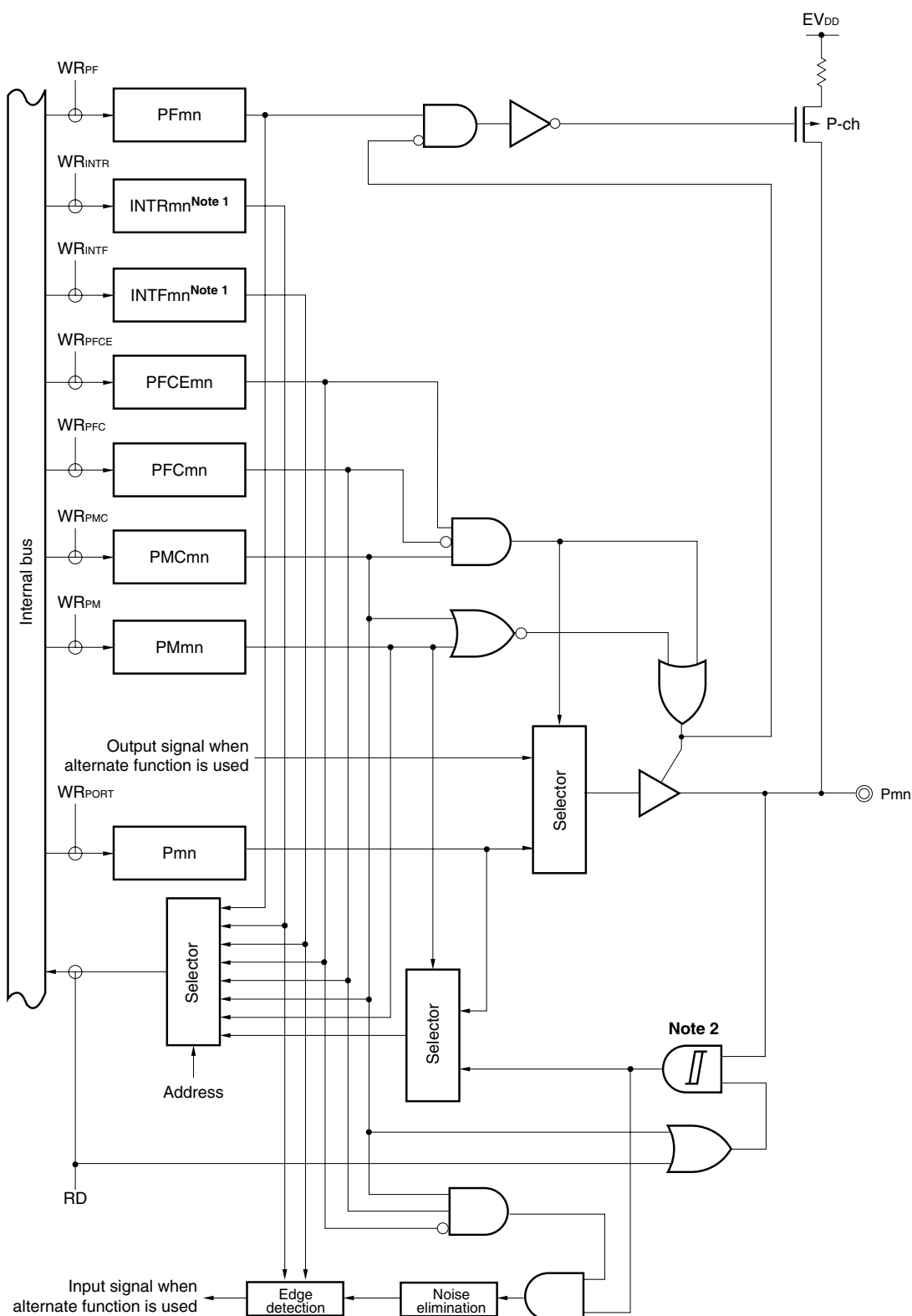
Figure 4-24. Block Diagram of Type W-1
