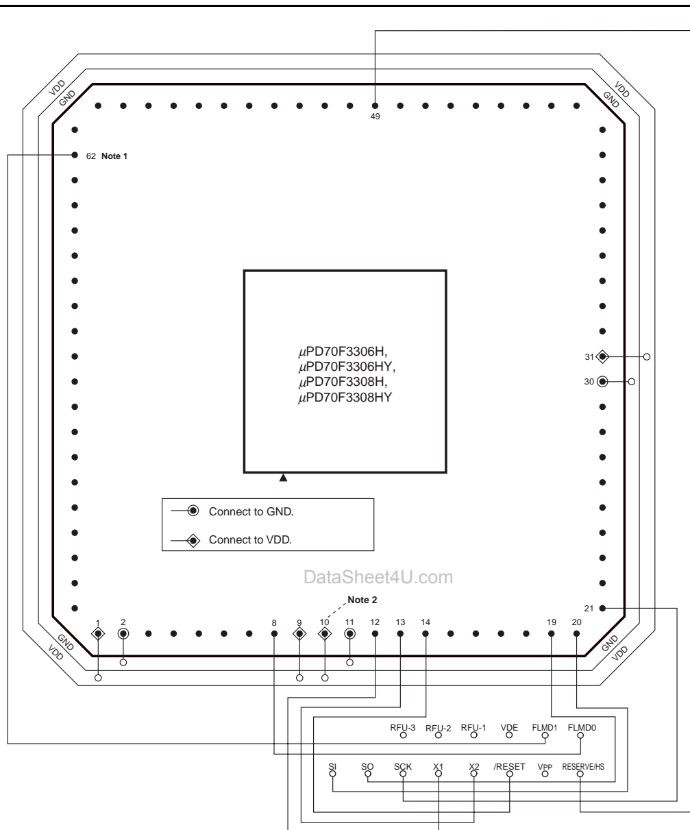
Figure 29-6. Wiring Example of V850ES/KF1+ Flash Writing Adapter (FA-80GC-8BT, FA-80GK-9EU)
