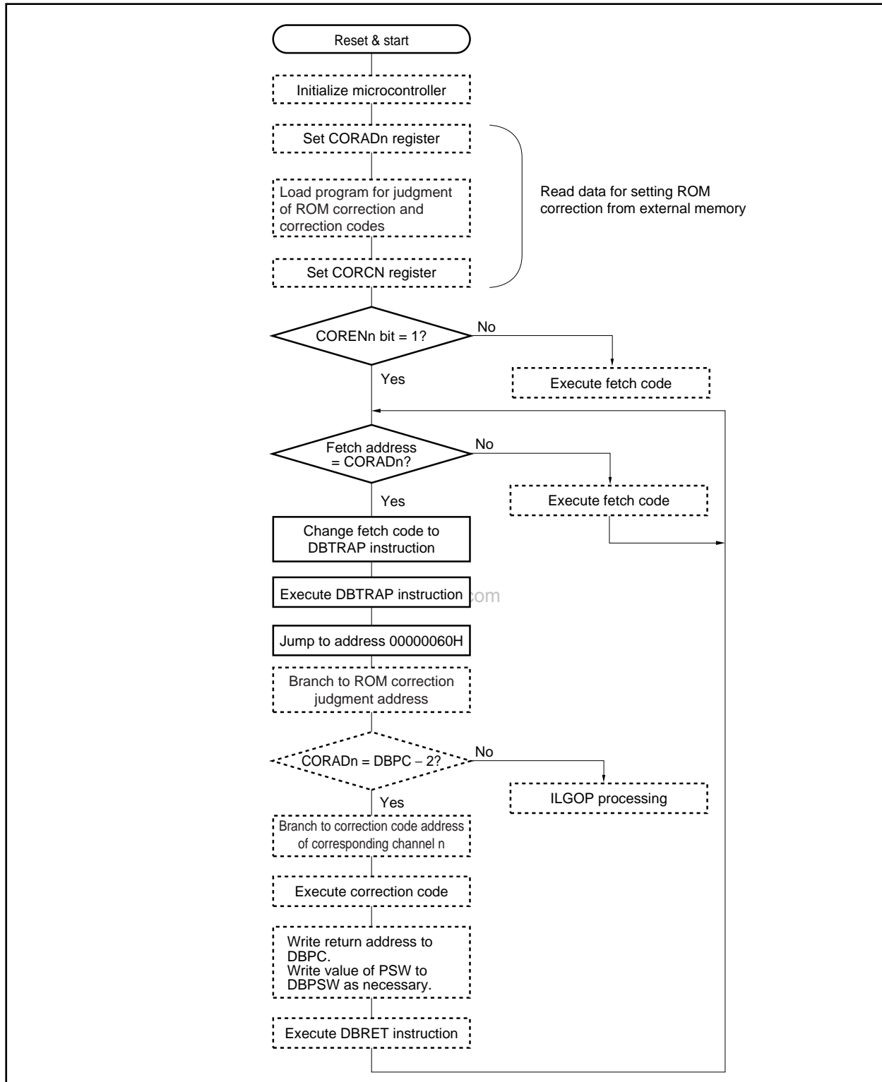
Figure 27-2. ROM Correction Operation and Program Flow
