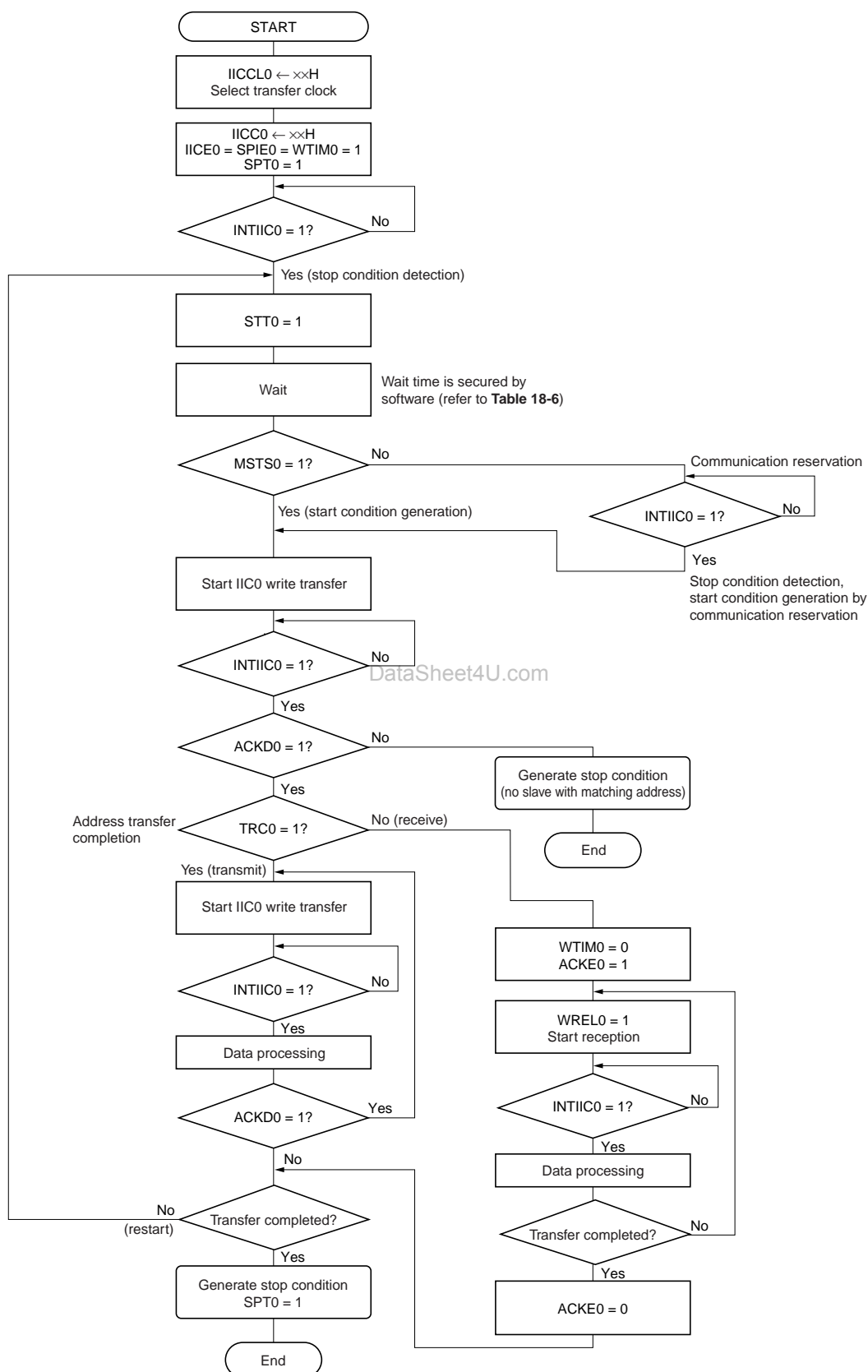
Figure 18-15. Master Operation Flowchart (1)
