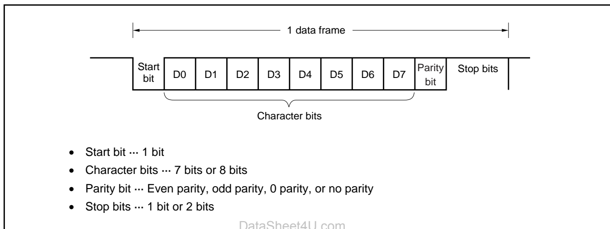
Figure 15-2. Format of UARTn Transmit/Receive Data
