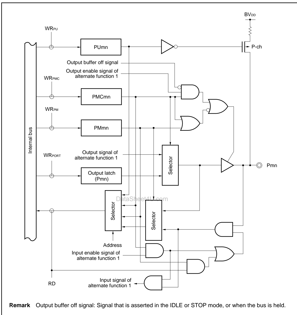
Figure 4-12. Block Diagram of Type D2-ULZ
