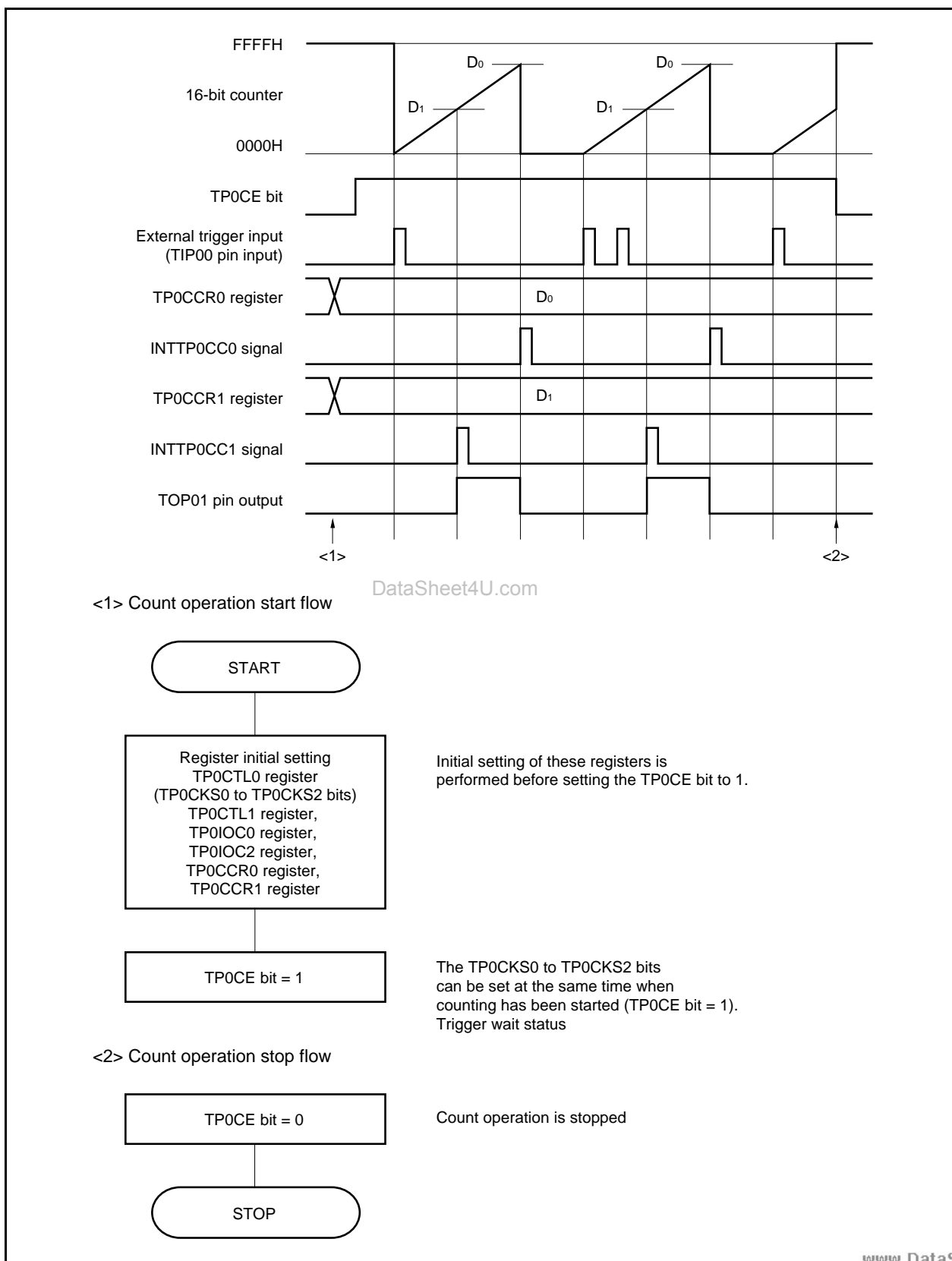
Figure 7-23. Software Processing Flow in One-Shot Pulse Output Mode
