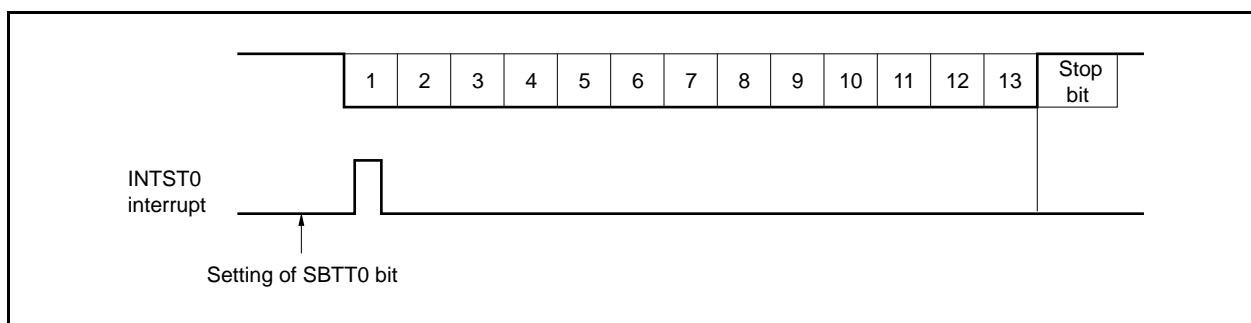
Figure 15-14. SBF Transmission
