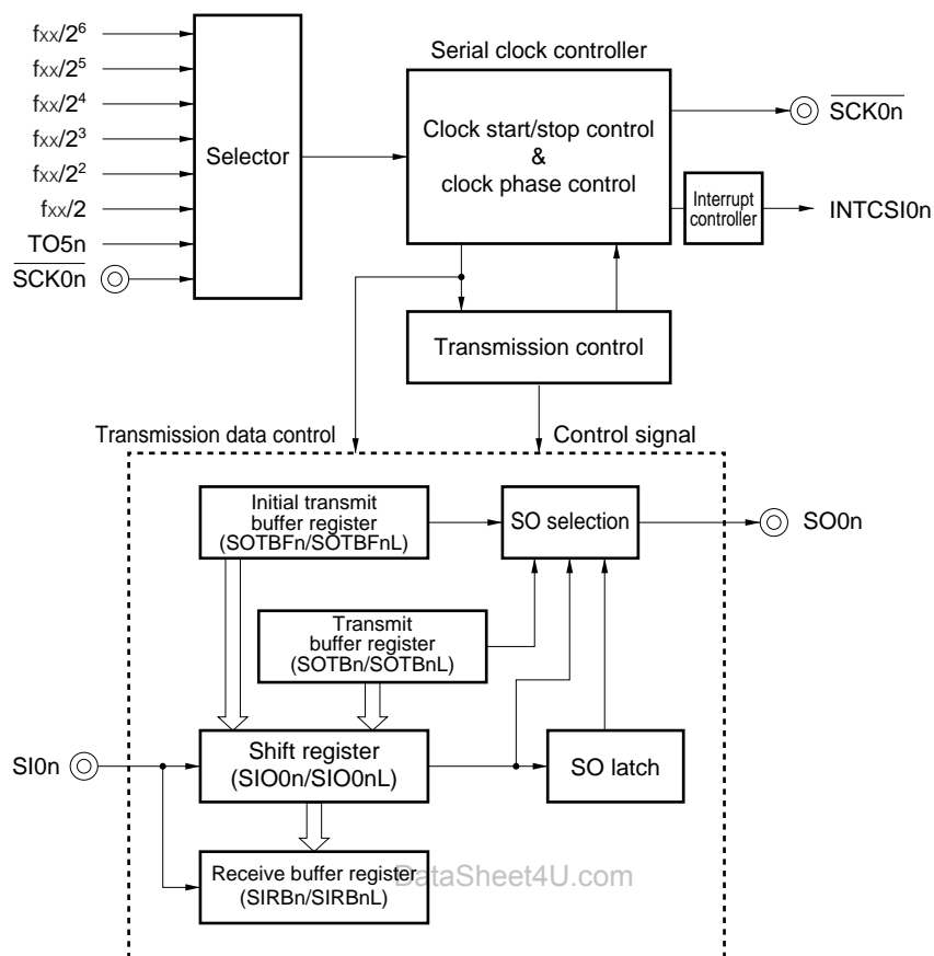
Figure 16-1. Block Diagram of Clocked Serial Interface
