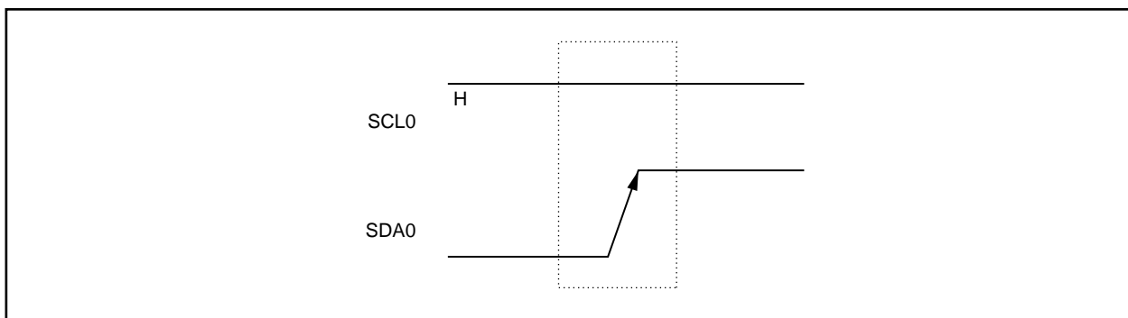
Figure 18-9. Stop Condition
