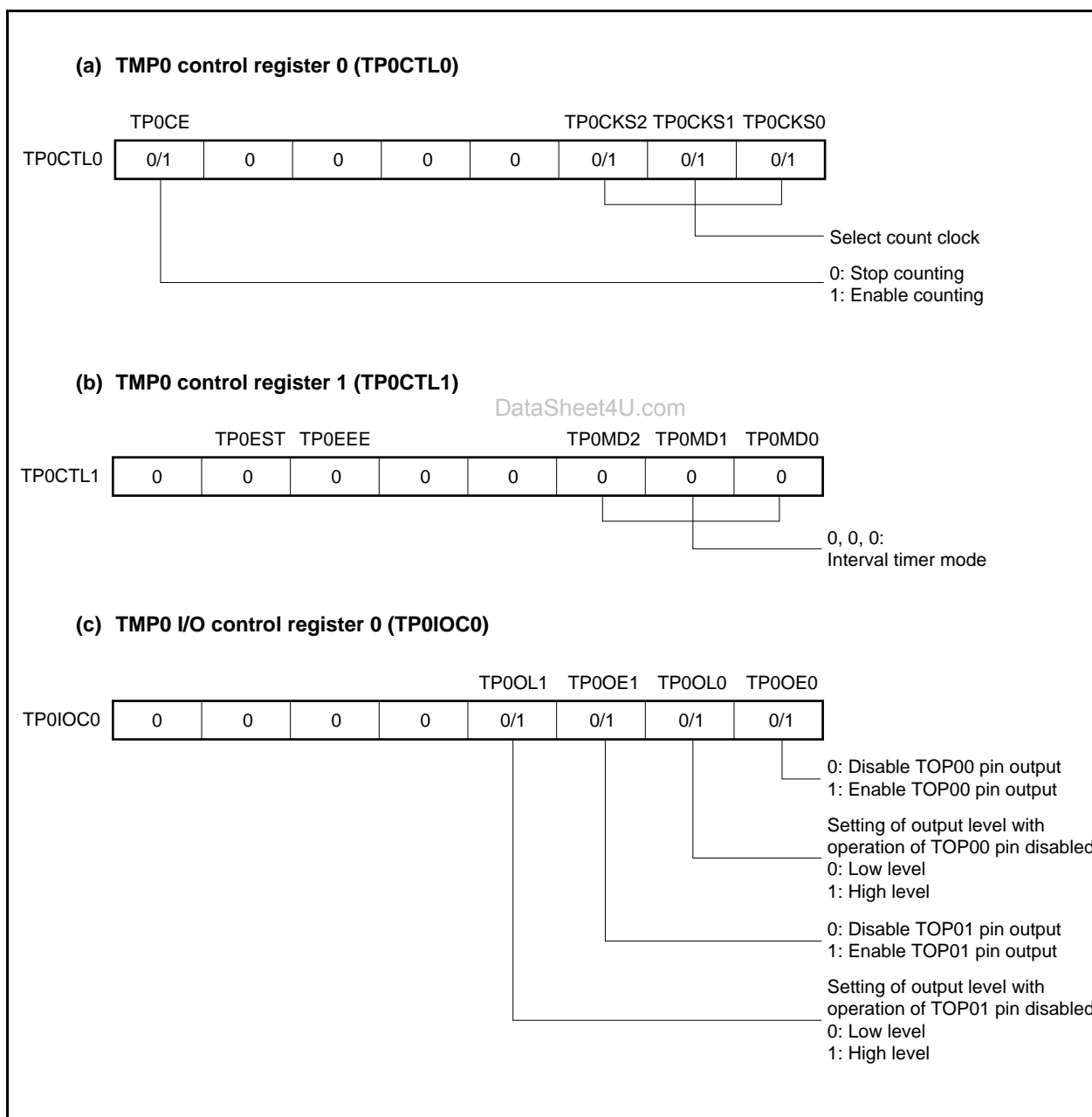
Figure 7-4. Register Setting for Interval Timer Mode Operation (1/2)
