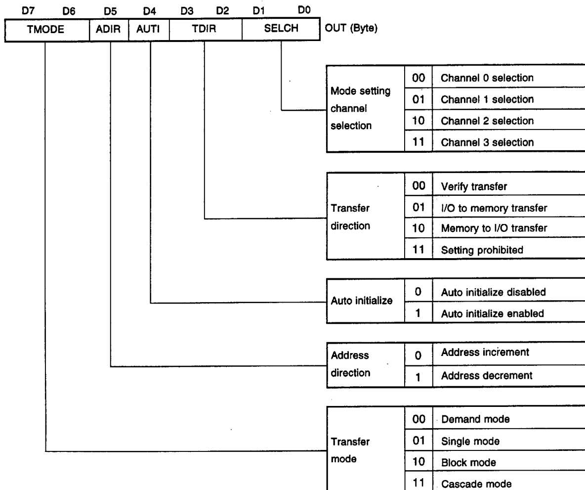
Fig. 10-15 Write Mode Register
