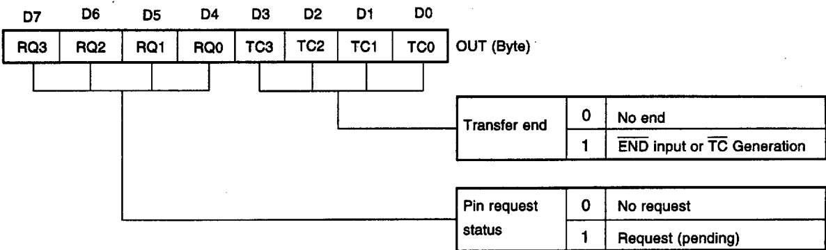
Fig. 10-10 Read Status Register
