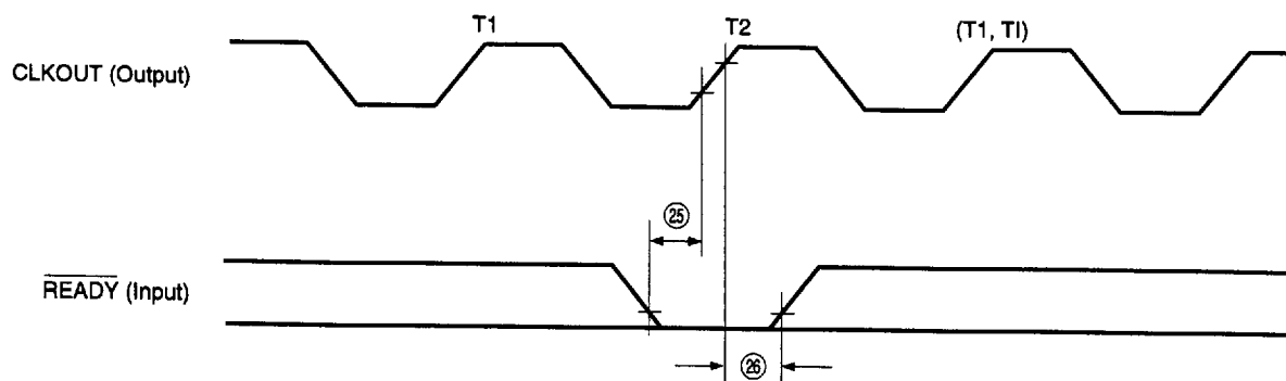
Fig. 15-3 CPU Ready Timing (No Wait)
