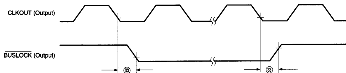
Fig. 15-12 Bus Lock
