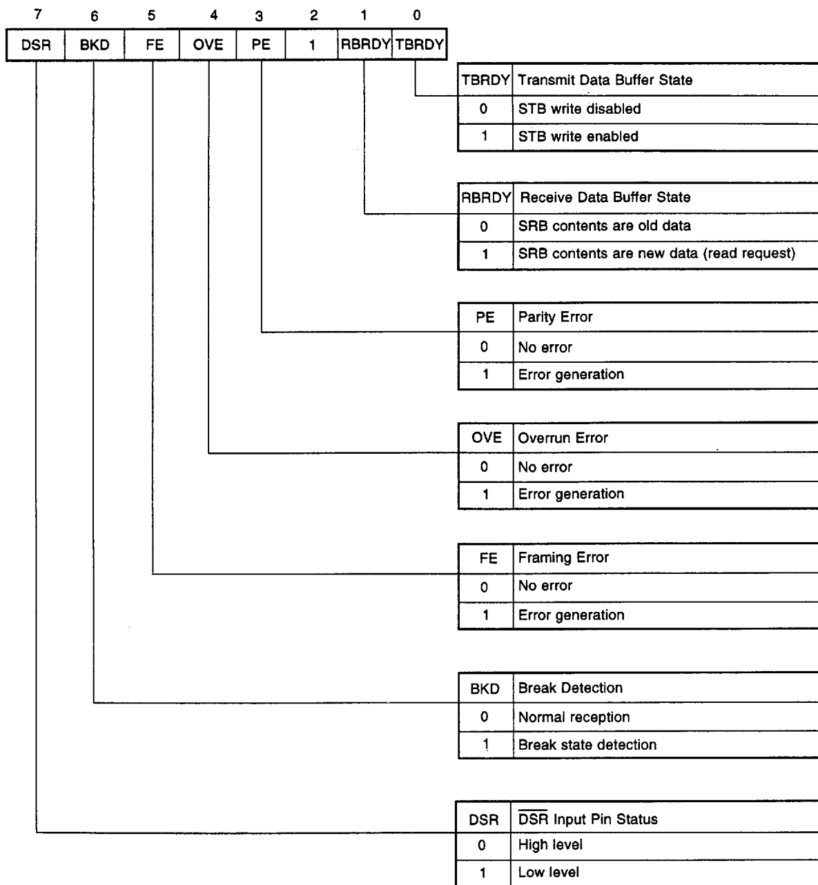
Fig. 8-5 SST (Serial Status Register)
