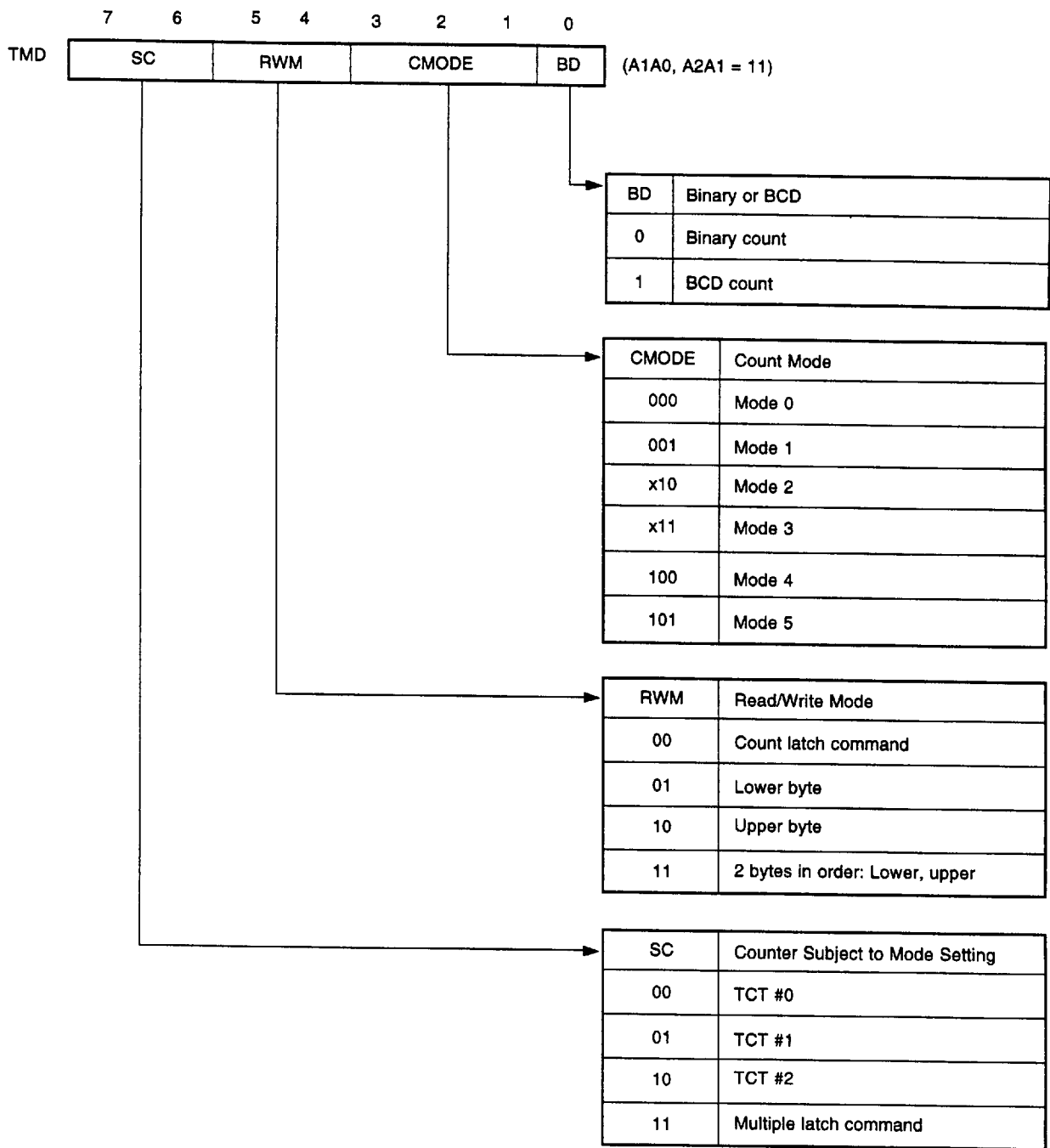
Fig. 7-2 Mode Word
