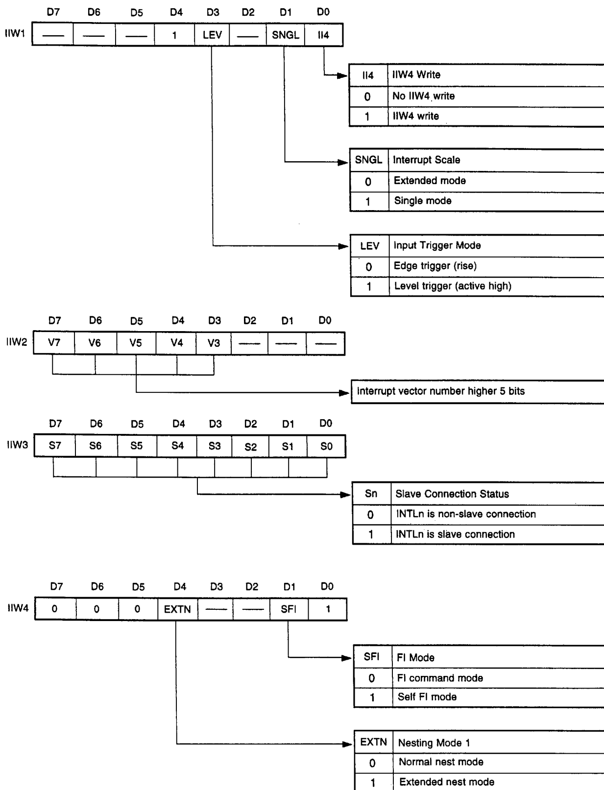
Fig. 9-2 ICU Initialization Words
