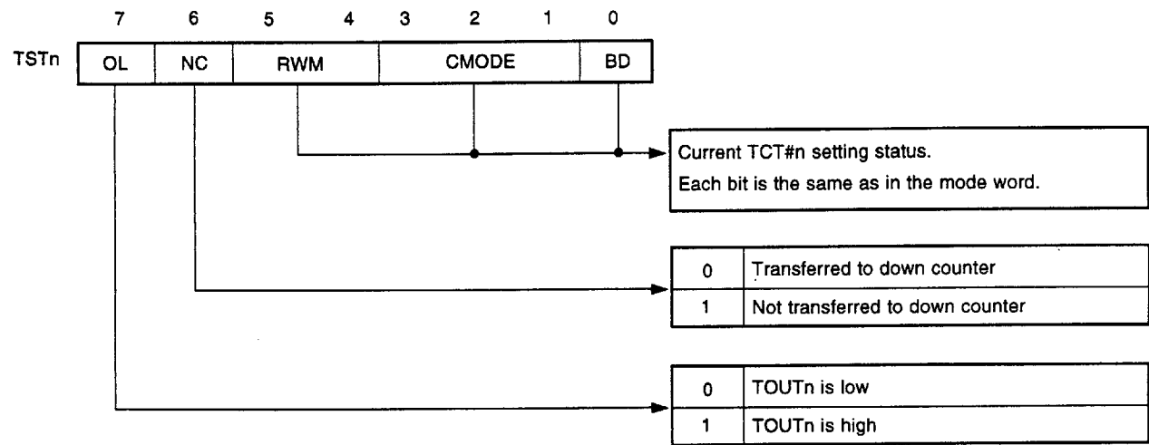
Fig. 7-5 Status
